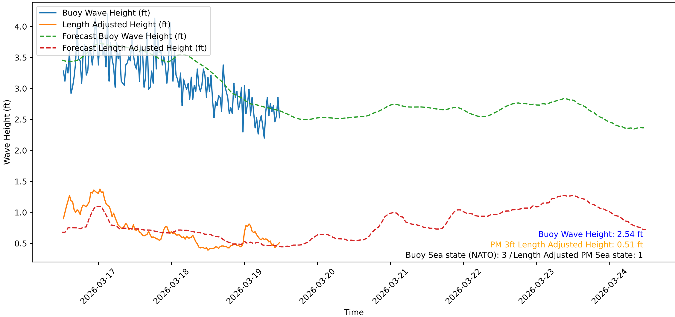
Wave Heights over Time for Green Beach at 2026-03-19 12:21:11
