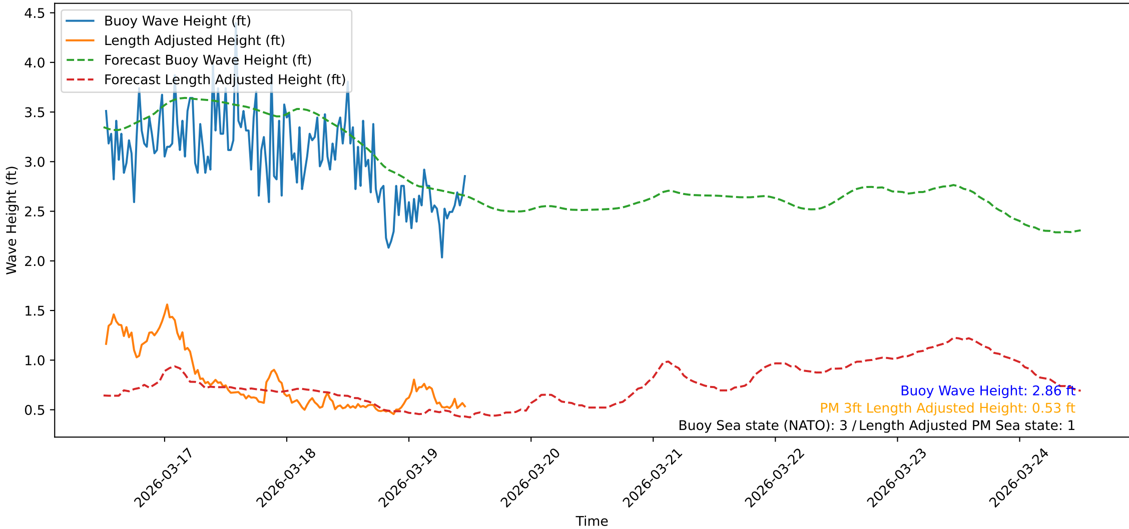
Wave Heights over Time for Oceanside Harbor at 2026-03-19 12:20:32
