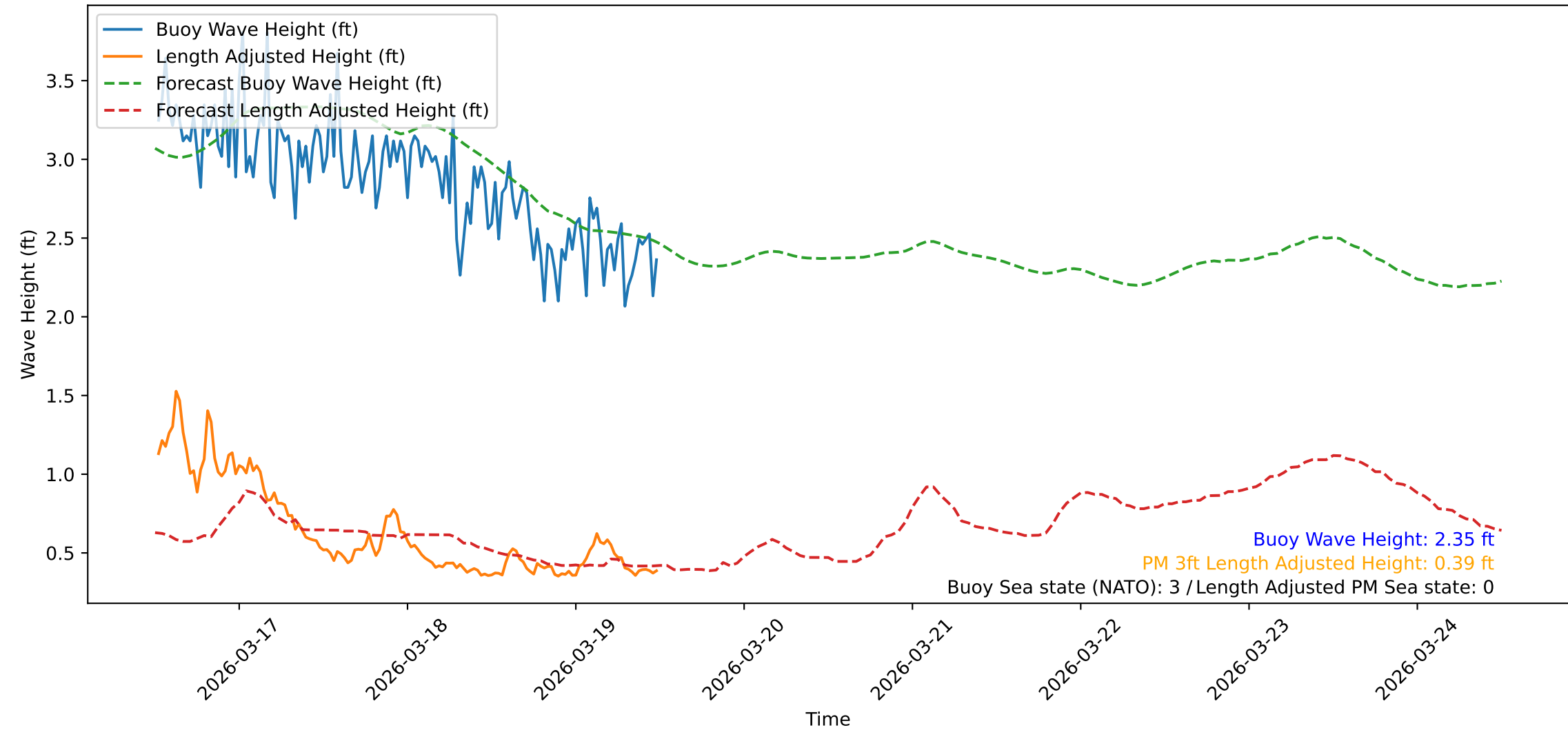
Wave Heights over Time for Red Beach at 2026-03-19 12:20:48
