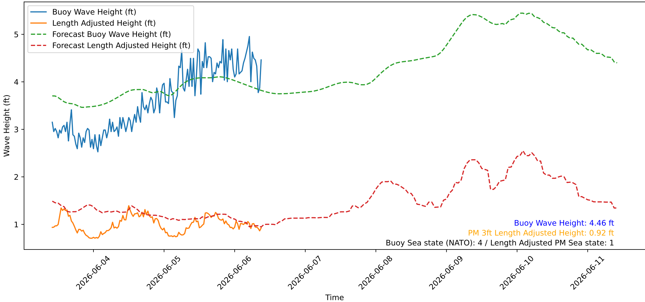
Wave Heights over Time for Red Beach at 2026-06-06 09:40:45
