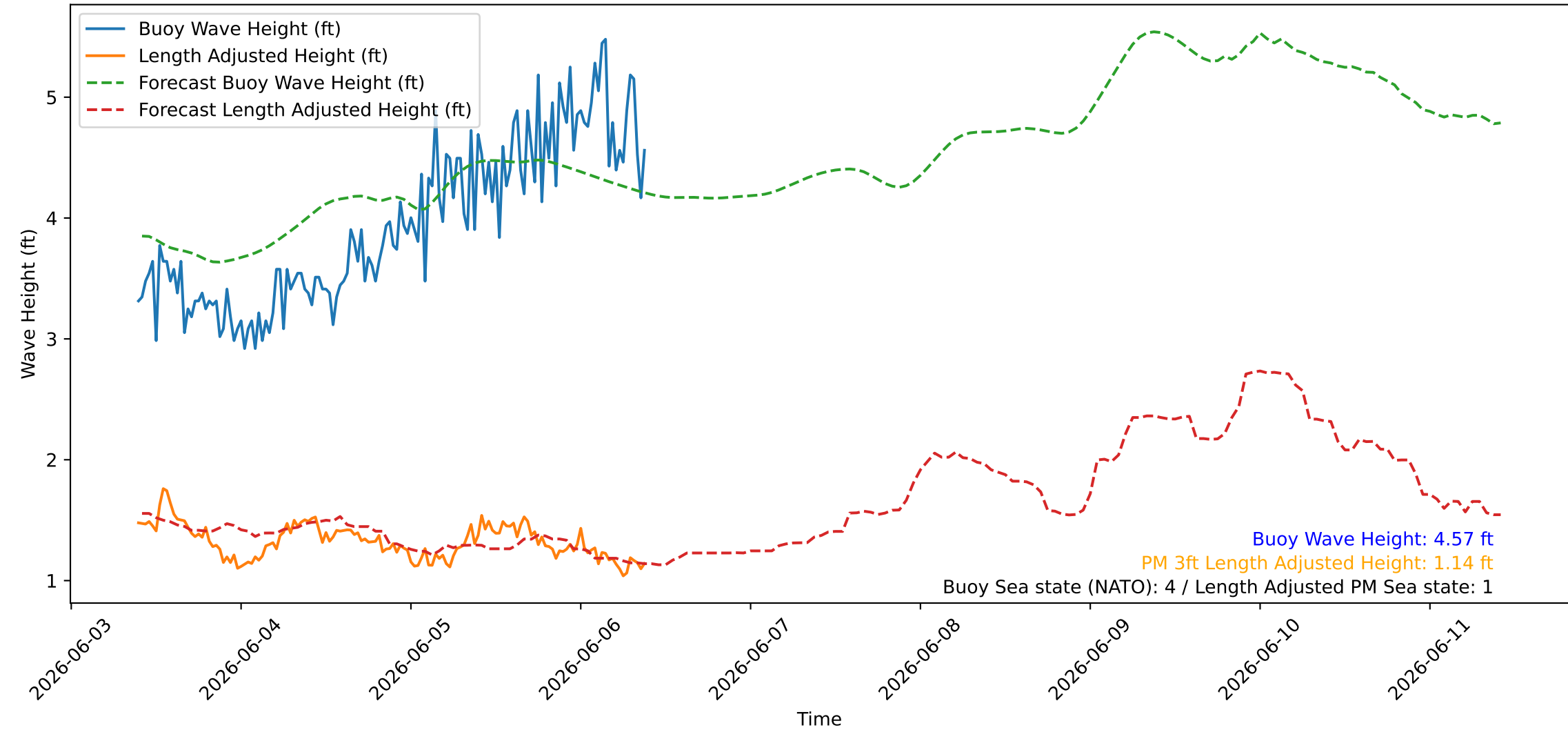
Wave Heights over Time for Oceanside Harbor at 2026-06-06 09:40:25
