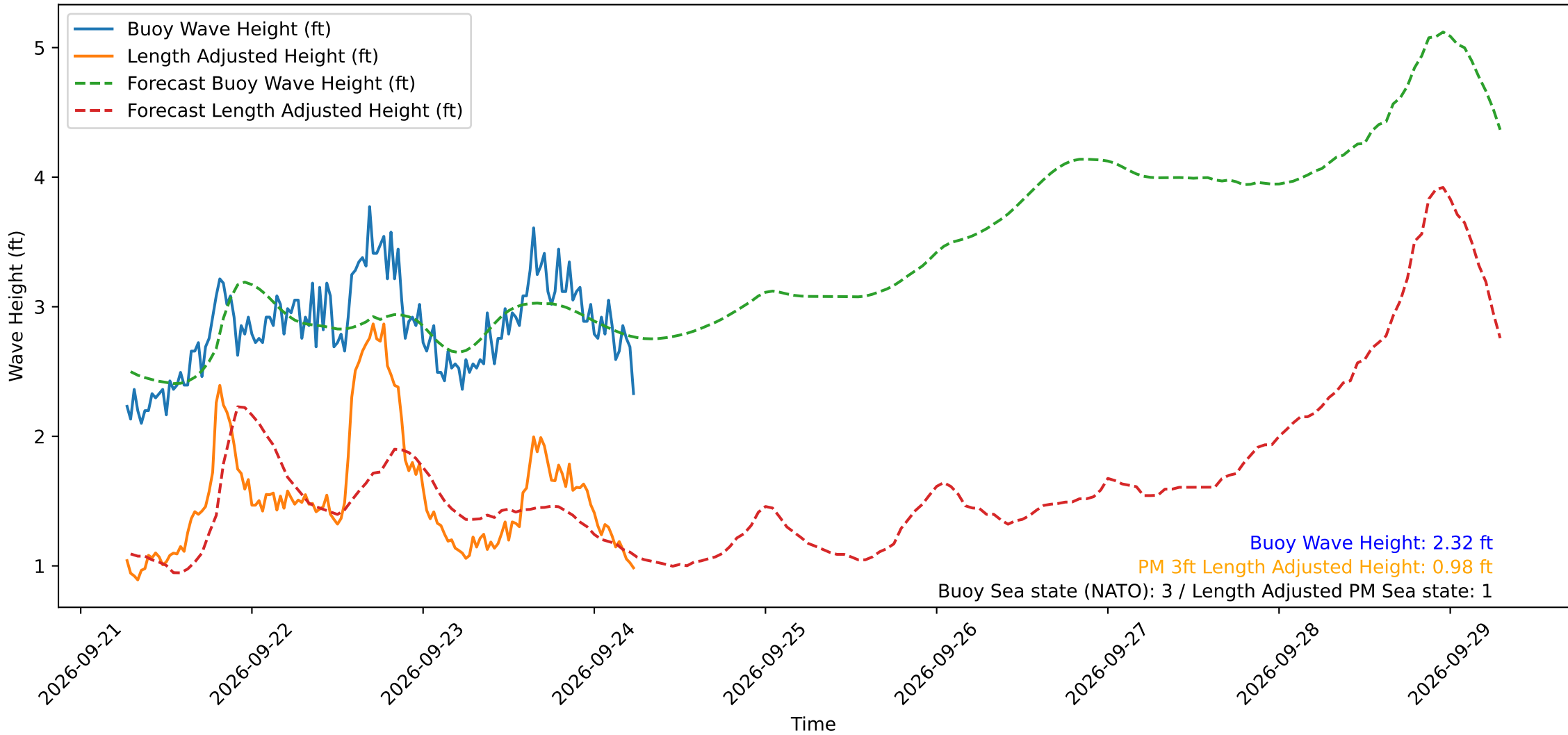
Wave Heights over Time for Oceanside Harbor at 2026-09-24 06:30:30
