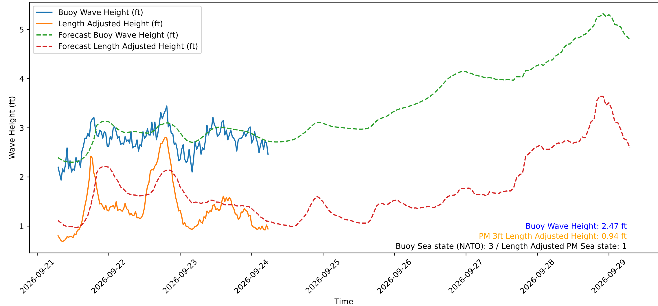
Wave Heights over Time for Green Beach at 2026-09-24 06:31:11
