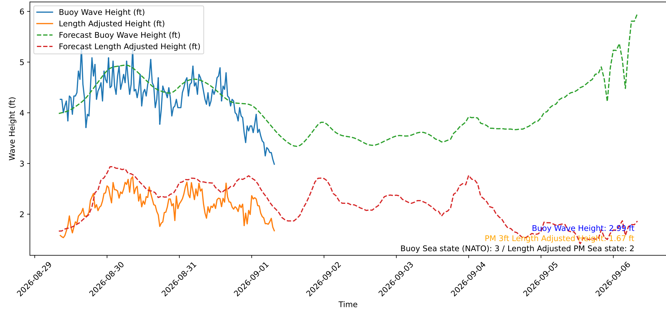
Wave Heights over Time for Oceanside Harbor at 2026-09-01 08:20:30
