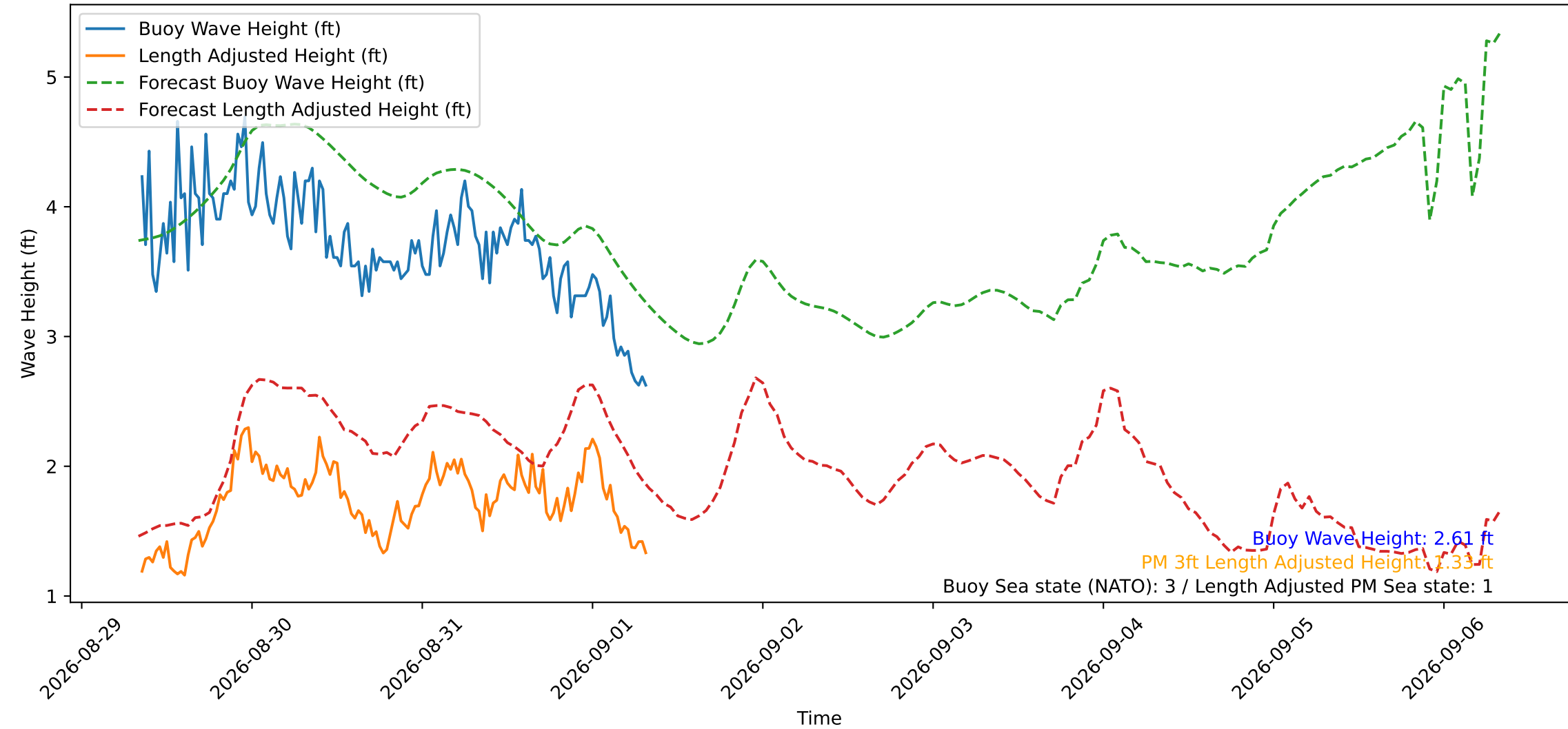
Wave Heights over Time for Red Beach at 2026-09-01 08:20:51
