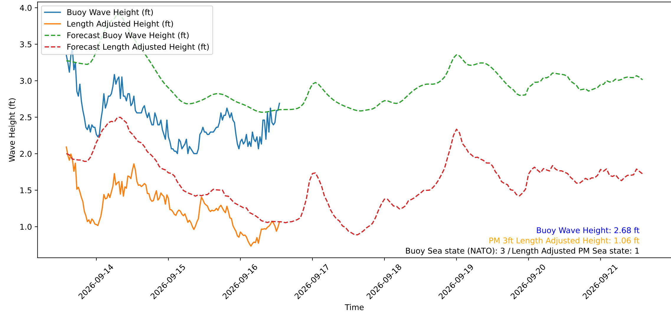
Wave Heights over Time for Red Beach at 2026-09-16 13:50:50
