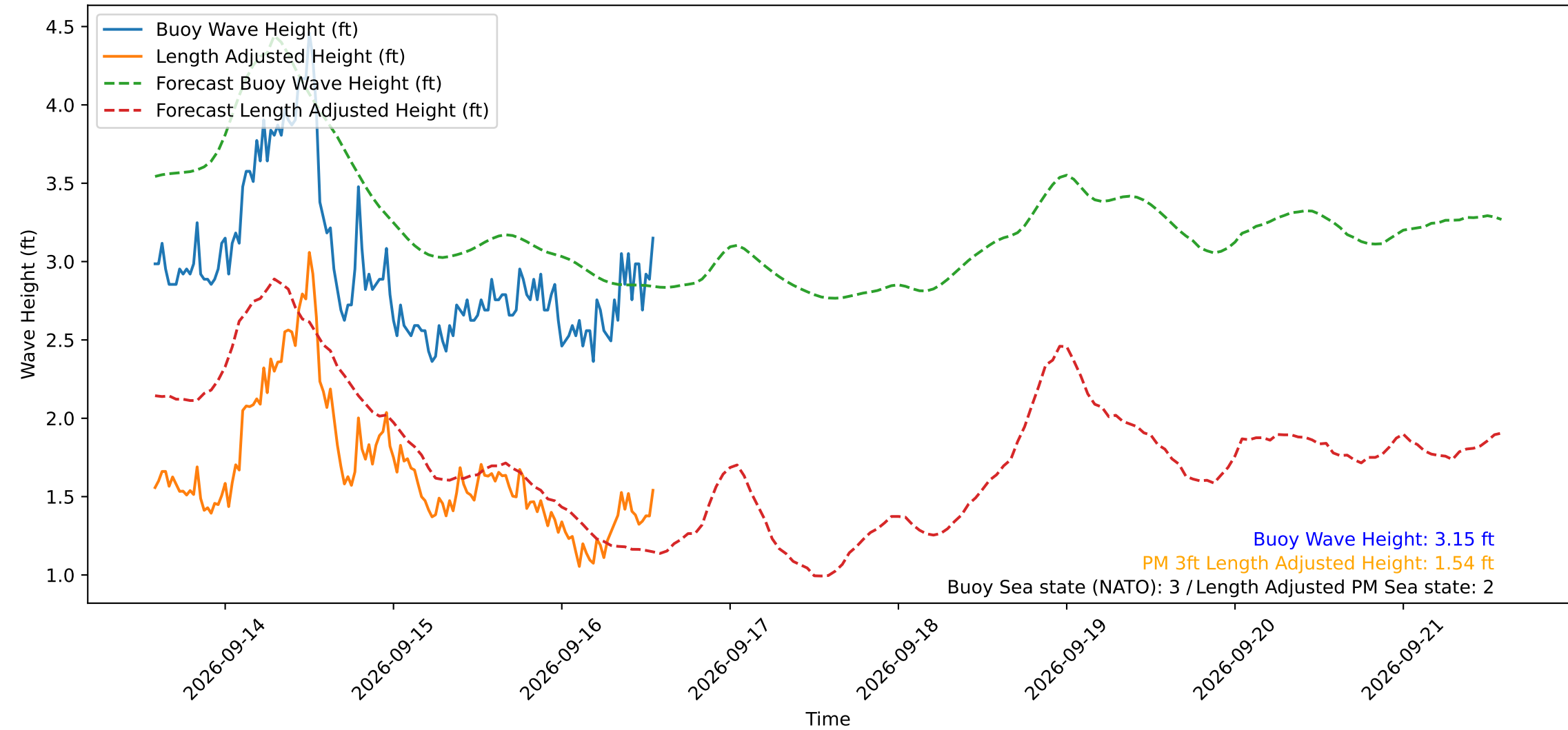
Wave Heights over Time for Oceanside Harbor at 2026-09-16 13:50:29
