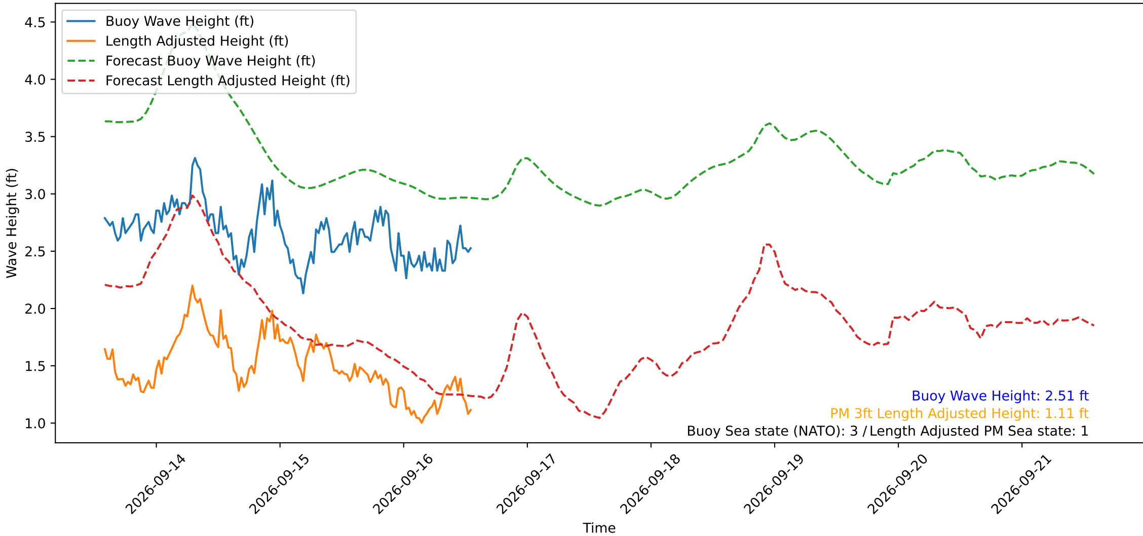
Wave Heights over Time for Green Beach at 2026-09-16 13:51:14
