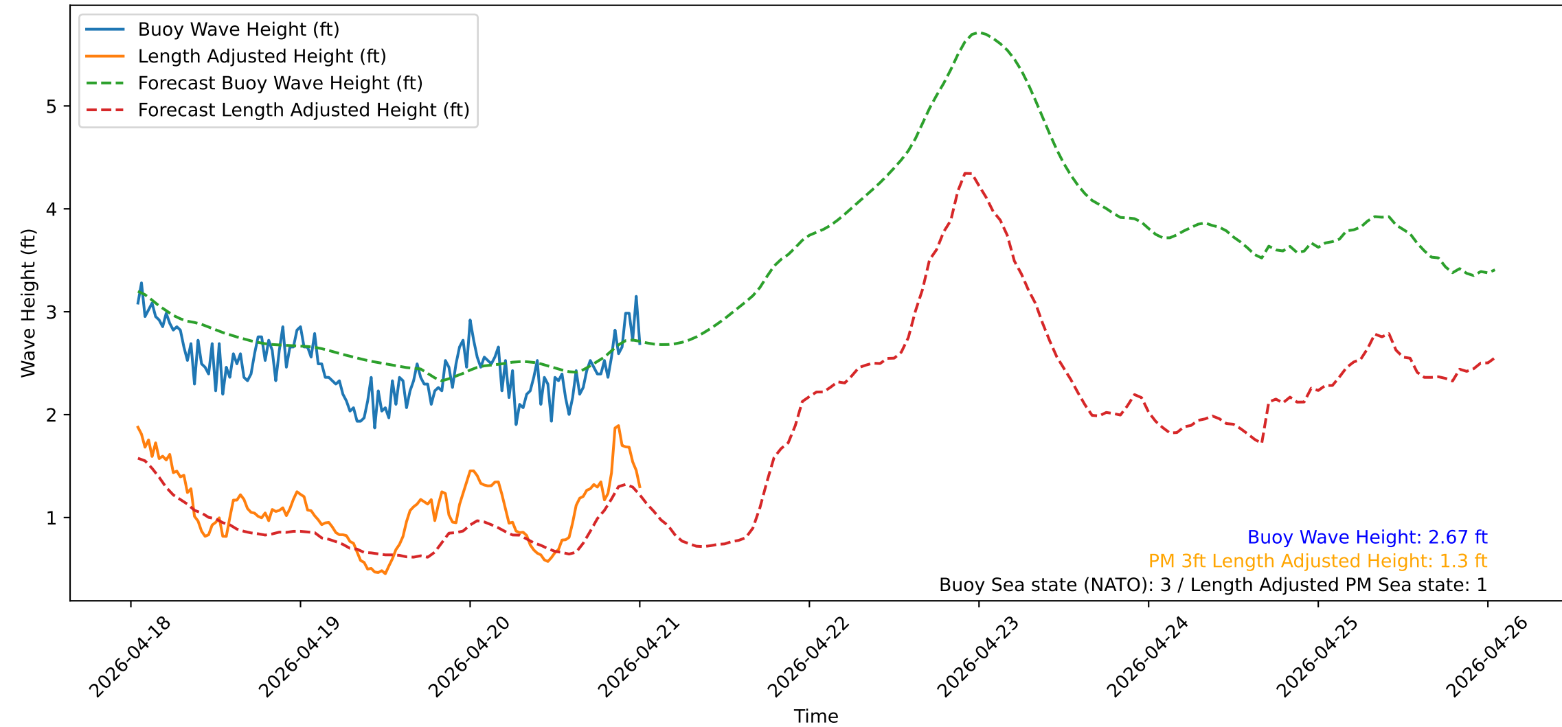
Wave Heights over Time for Green Beach at 2026-04-21 00:51:14
