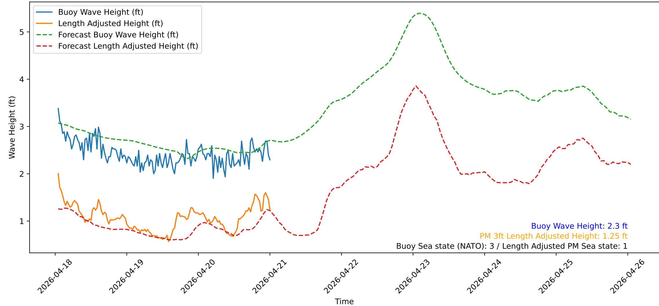
Wave Heights over Time for Oceanside Harbor at 2026-04-21 00:50:31
