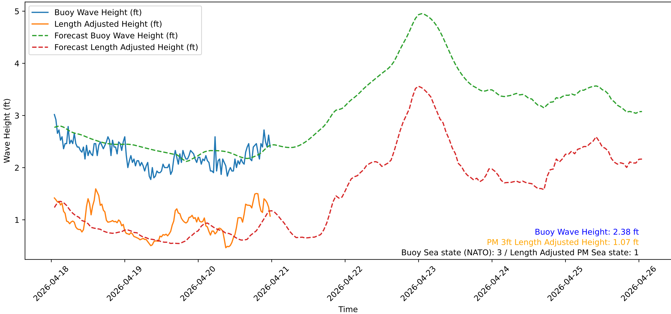
Wave Heights over Time for Red Beach at 2026-04-21 00:50:51
