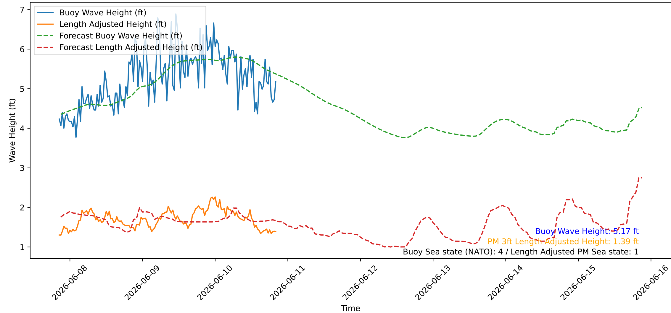
Wave Heights over Time for Green Beach at 2026-06-10 20:41:10
