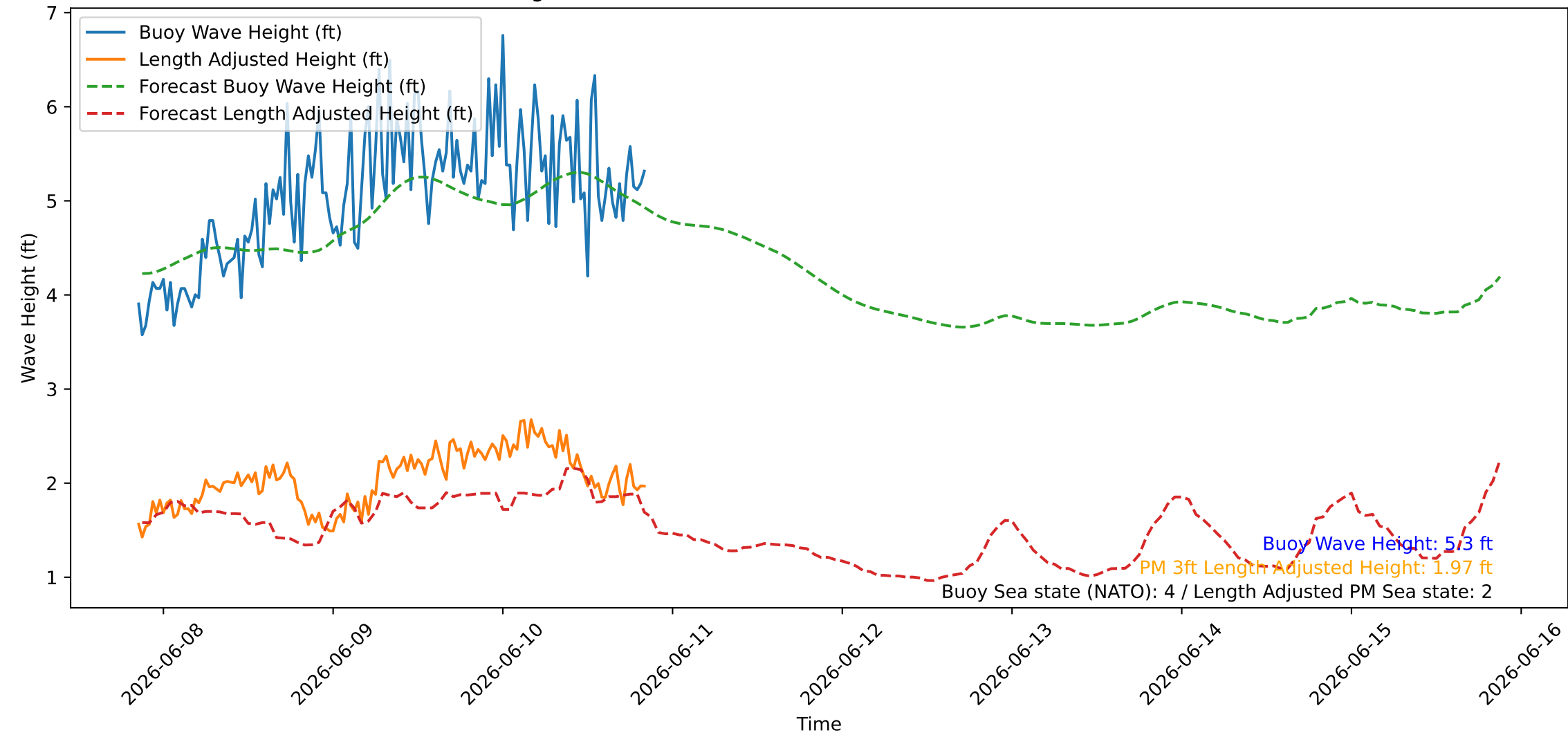
Wave Heights over Time for Oceanside Harbor at 2026-06-10 20:40:26
