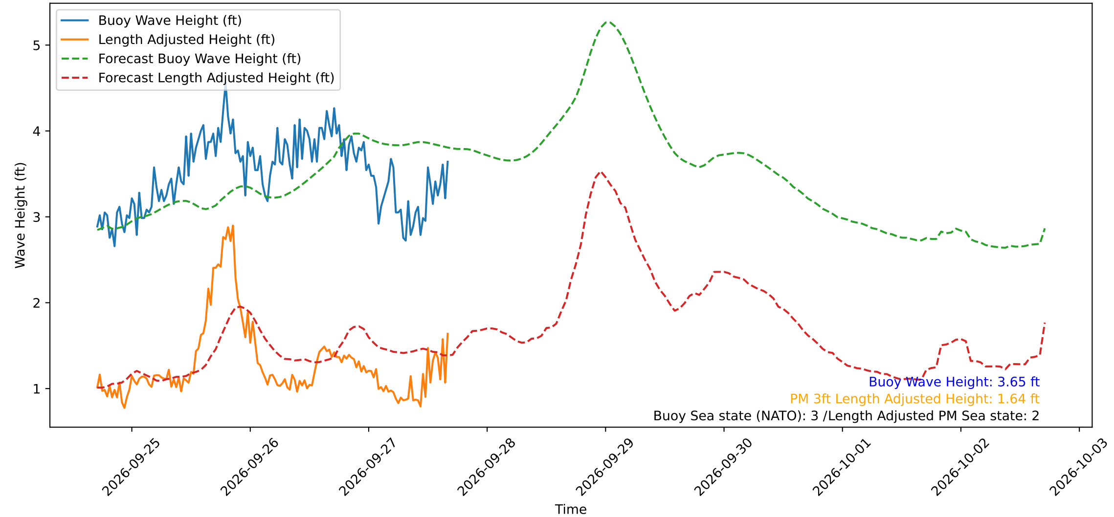
Wave Heights over Time for Green Beach at 2026-09-27 16:41:12
