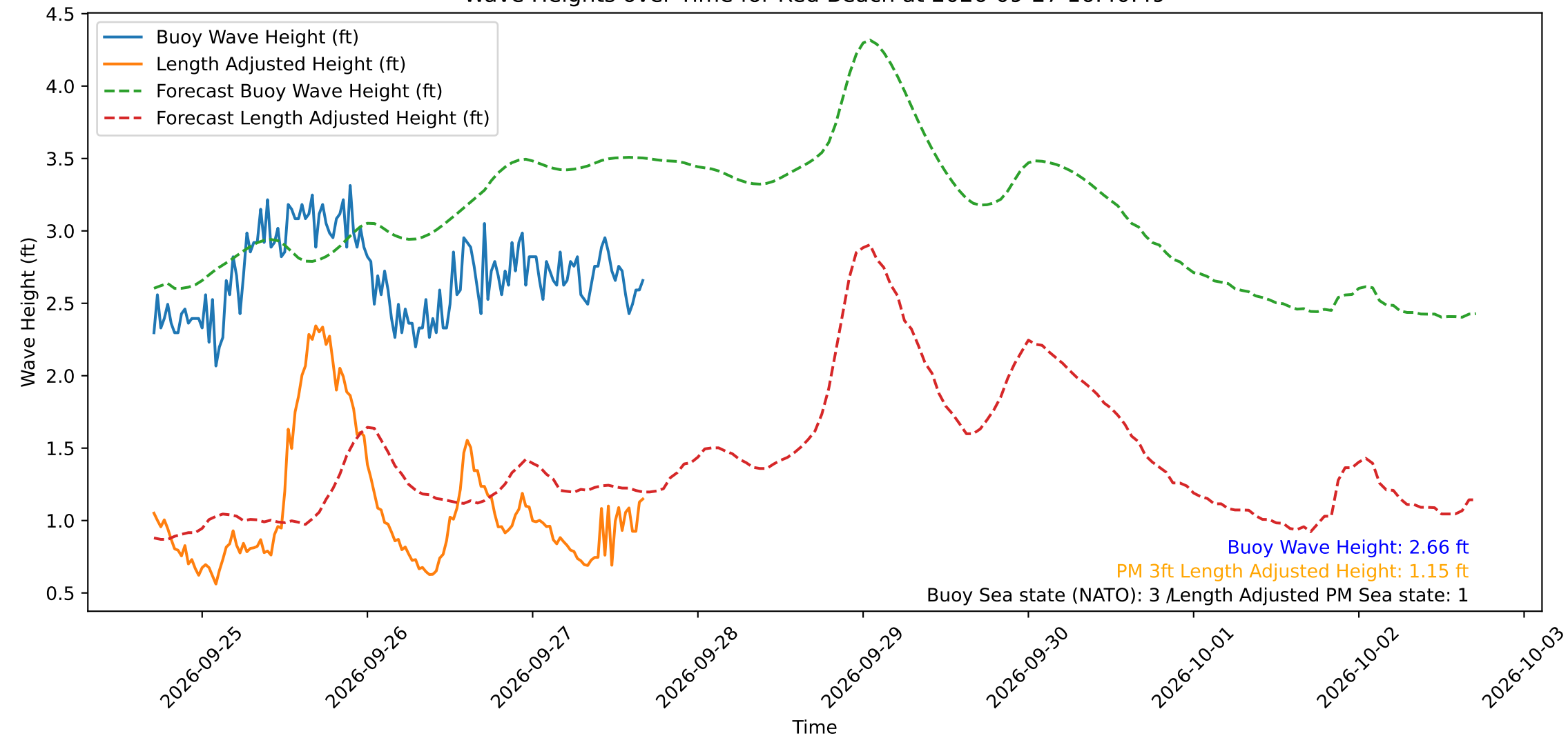
Wave Heights over Time for Red Beach at 2026-09-27 16:40:49
