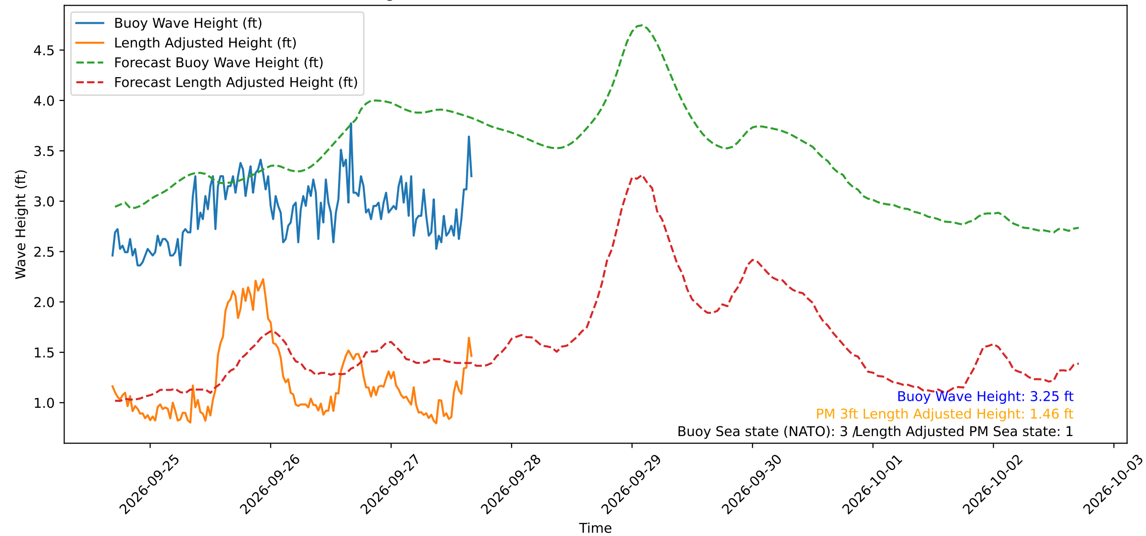
Wave Heights over Time for Oceanside Harbor at 2026-09-27 16:40:29
