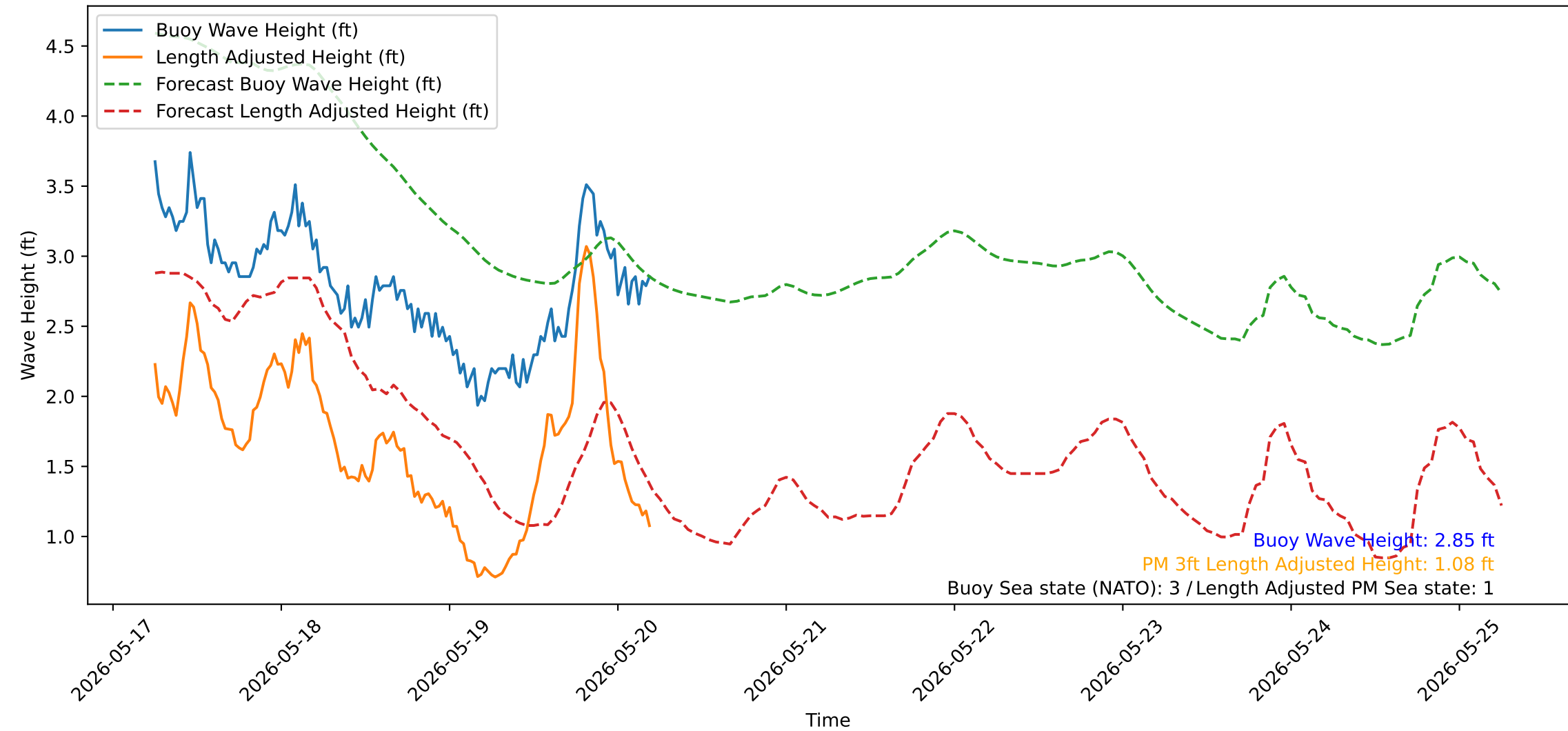
Wave Heights over Time for Red Beach at 2026-05-20 05:50:51
