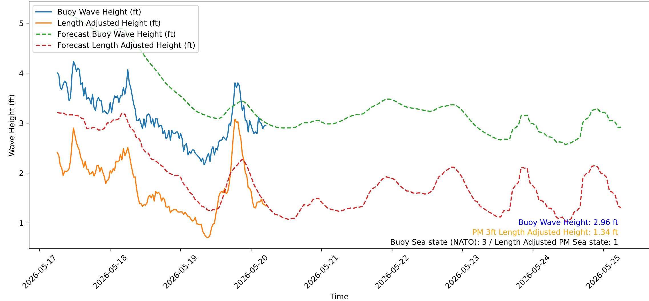
Wave Heights over Time for Green Beach at 2026-05-20 05:51:14
