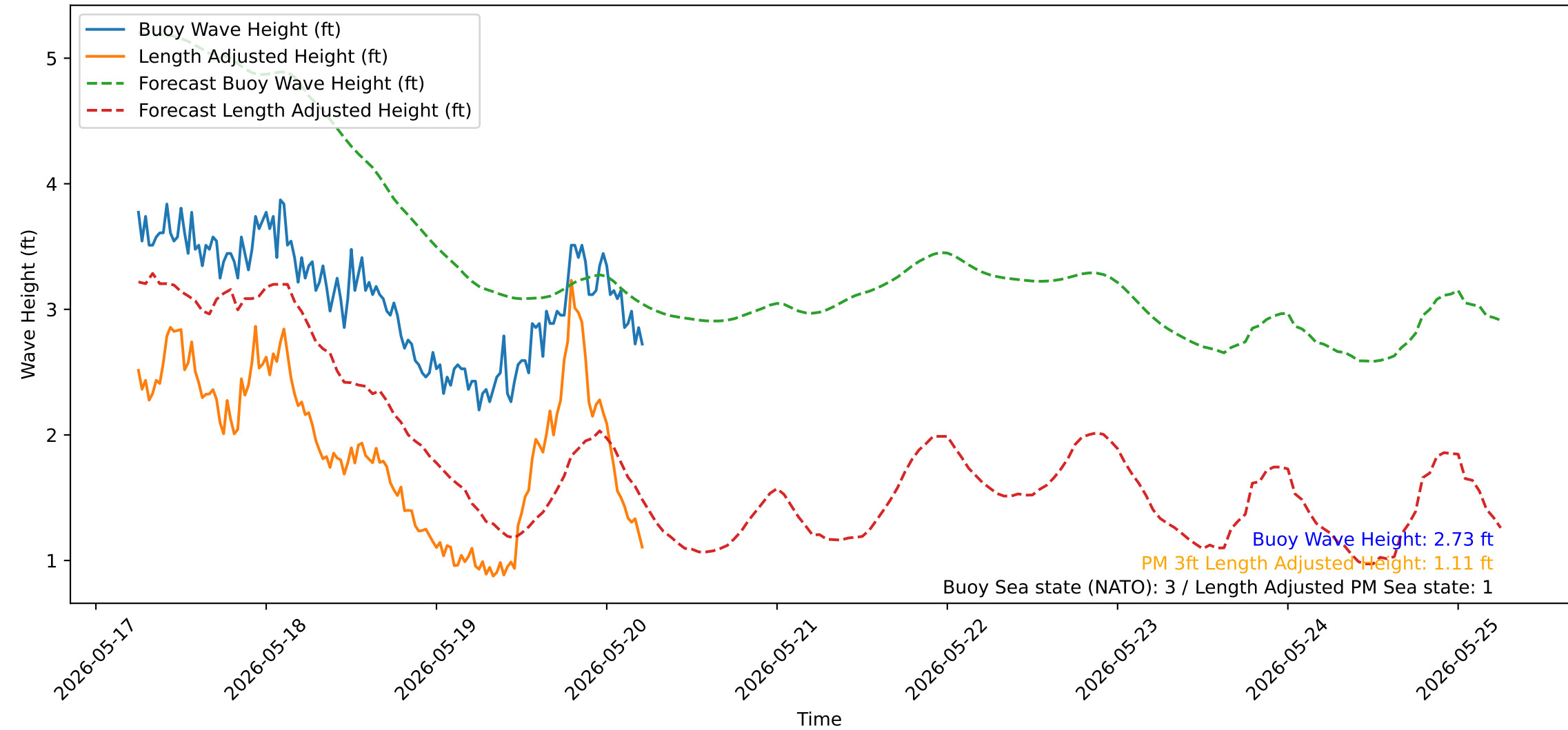
Wave Heights over Time for Oceanside Harbor at 2026-05-20 05:50:31
