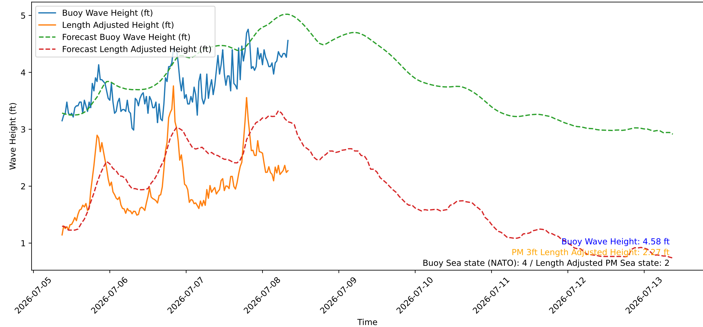
Wave Heights over Time for Green Beach at 2026-07-08 08:51:09
