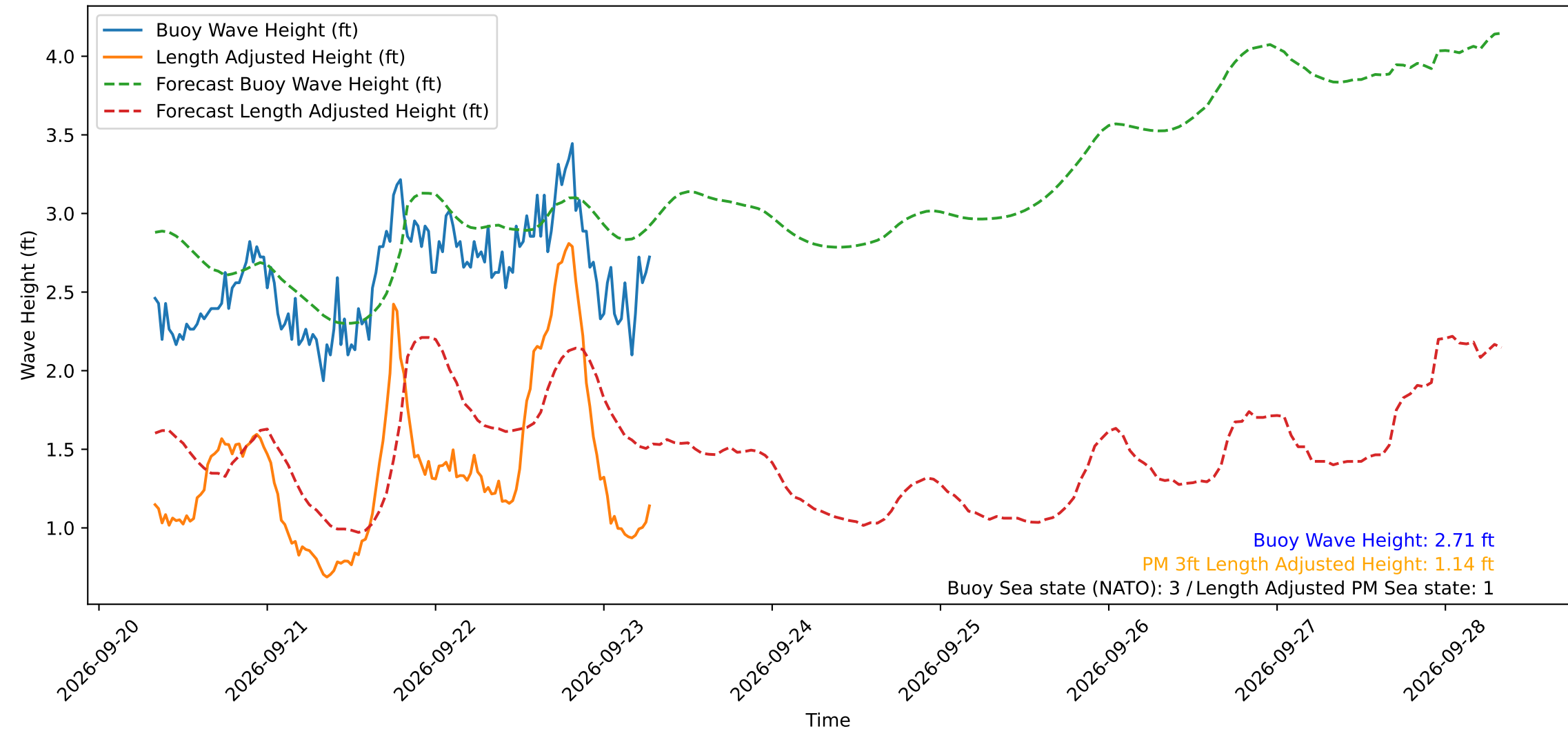
Wave Heights over Time for Green Beach at 2026-09-23 07:31:12
