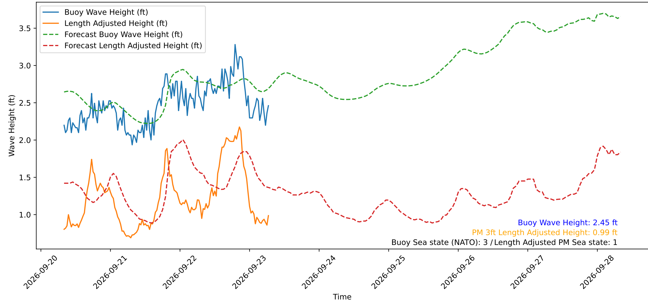
Wave Heights over Time for Red Beach at 2026-09-23 07:30:50
