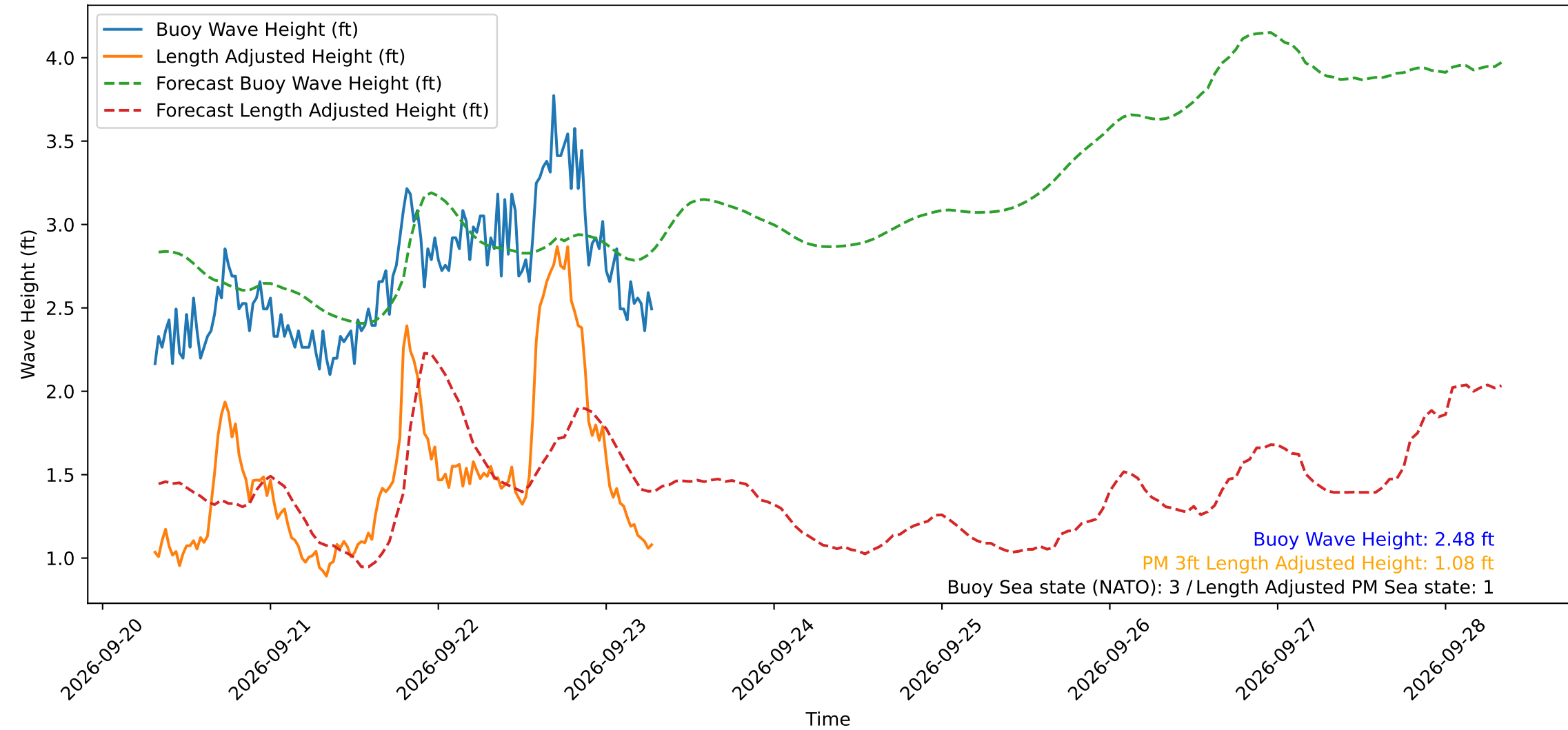
Wave Heights over Time for Oceanside Harbor at 2026-09-23 07:30:30
