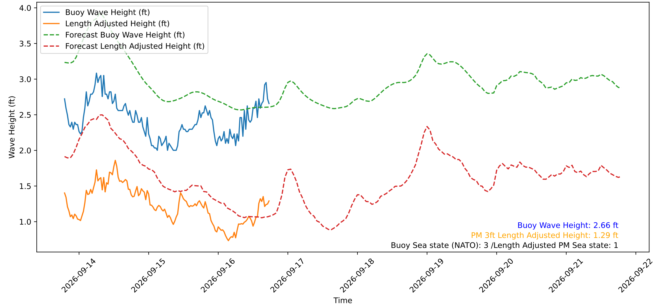
Wave Heights over Time for Red Beach at 2026-09-16 18:30:50
