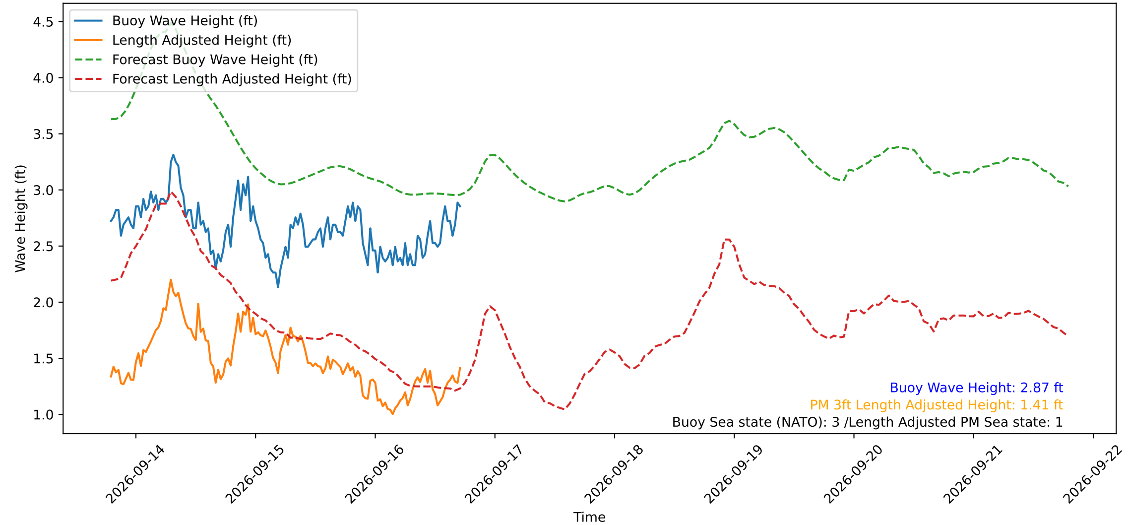
Wave Heights over Time for Green Beach at 2026-09-16 18:31:14
