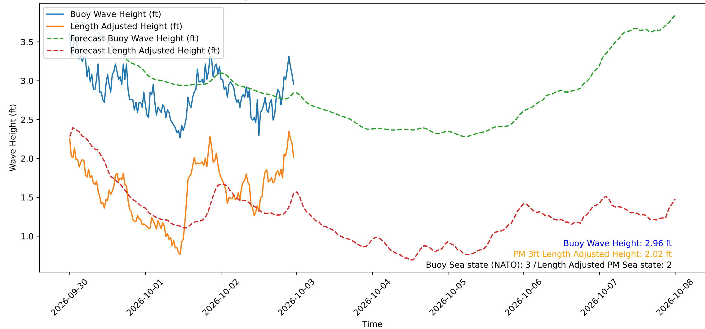
Wave Heights over Time for Oceanside Harbor at 2026-10-02 23:50:29
