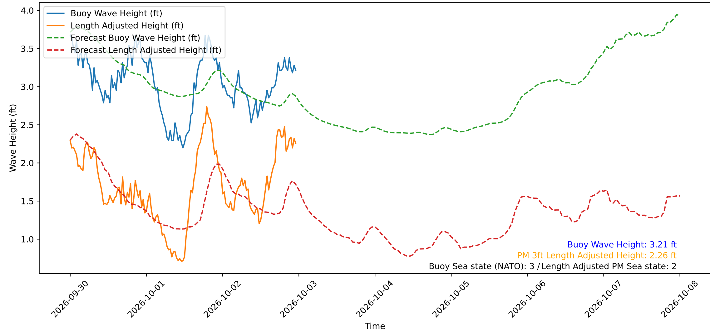
Wave Heights over Time for Green Beach at 2026-10-02 23:51:13
