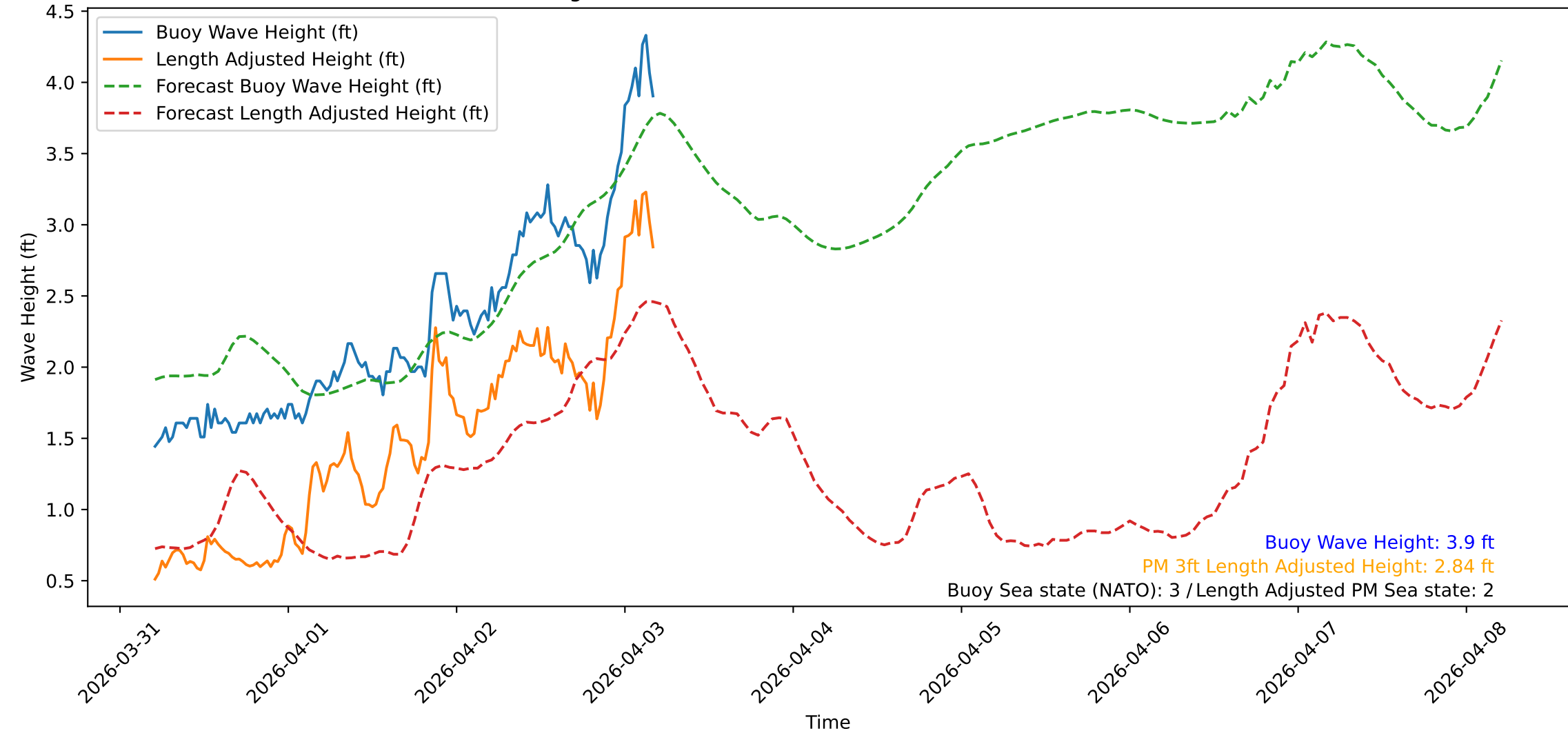
Wave Heights over Time for Green Beach at 2026-04-03 04:51:09
