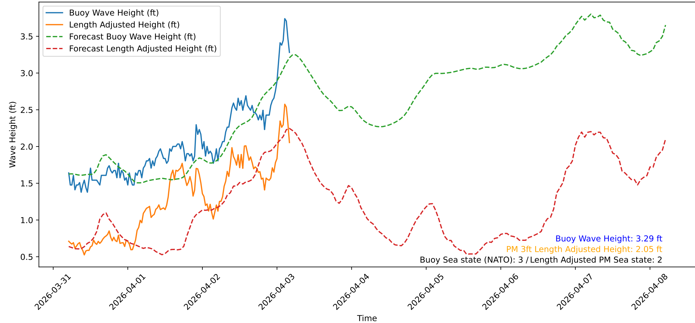
Wave Heights over Time for Red Beach at 2026-04-03 04:50:47
