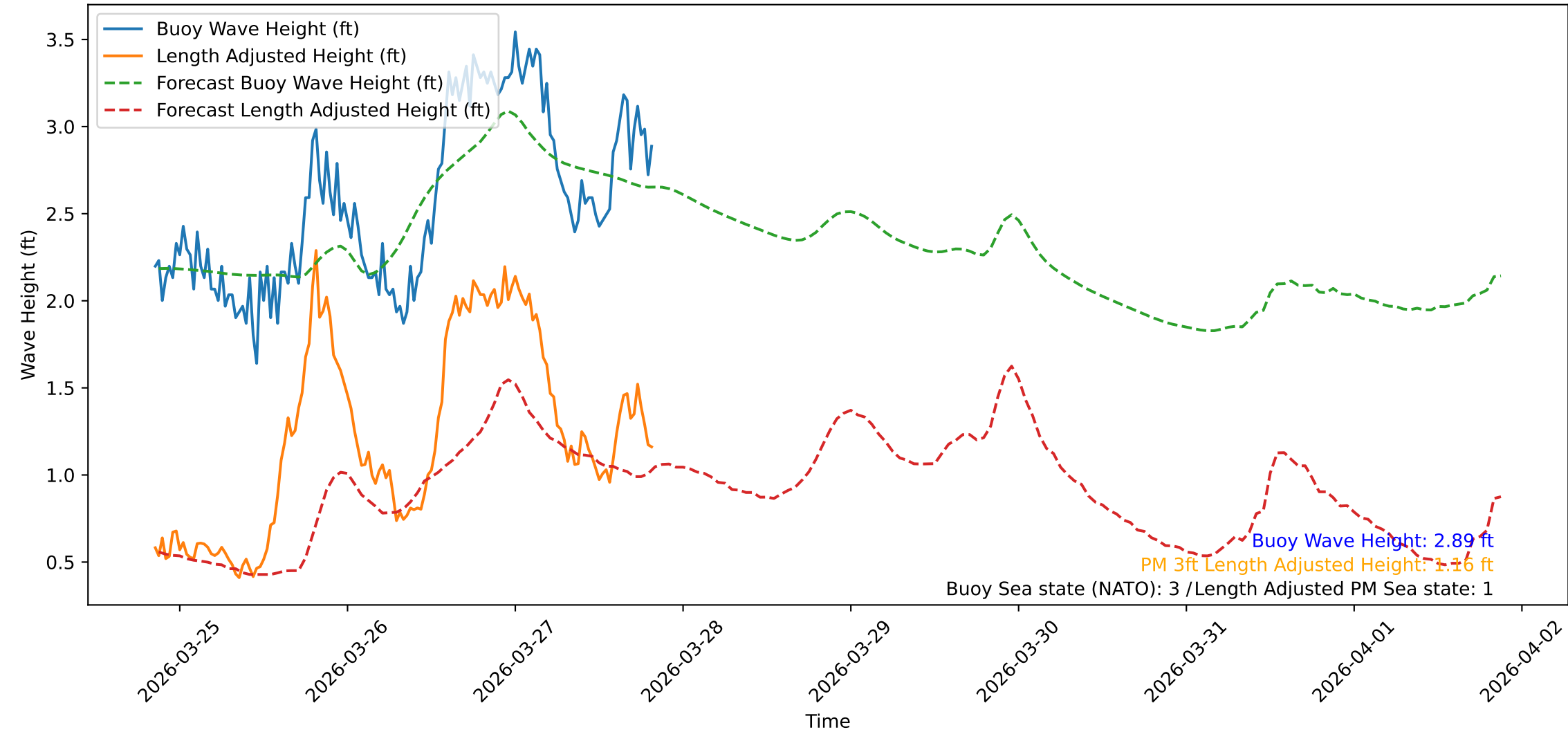
Wave Heights over Time for Green Beach at 2026-03-27 20:31:10
