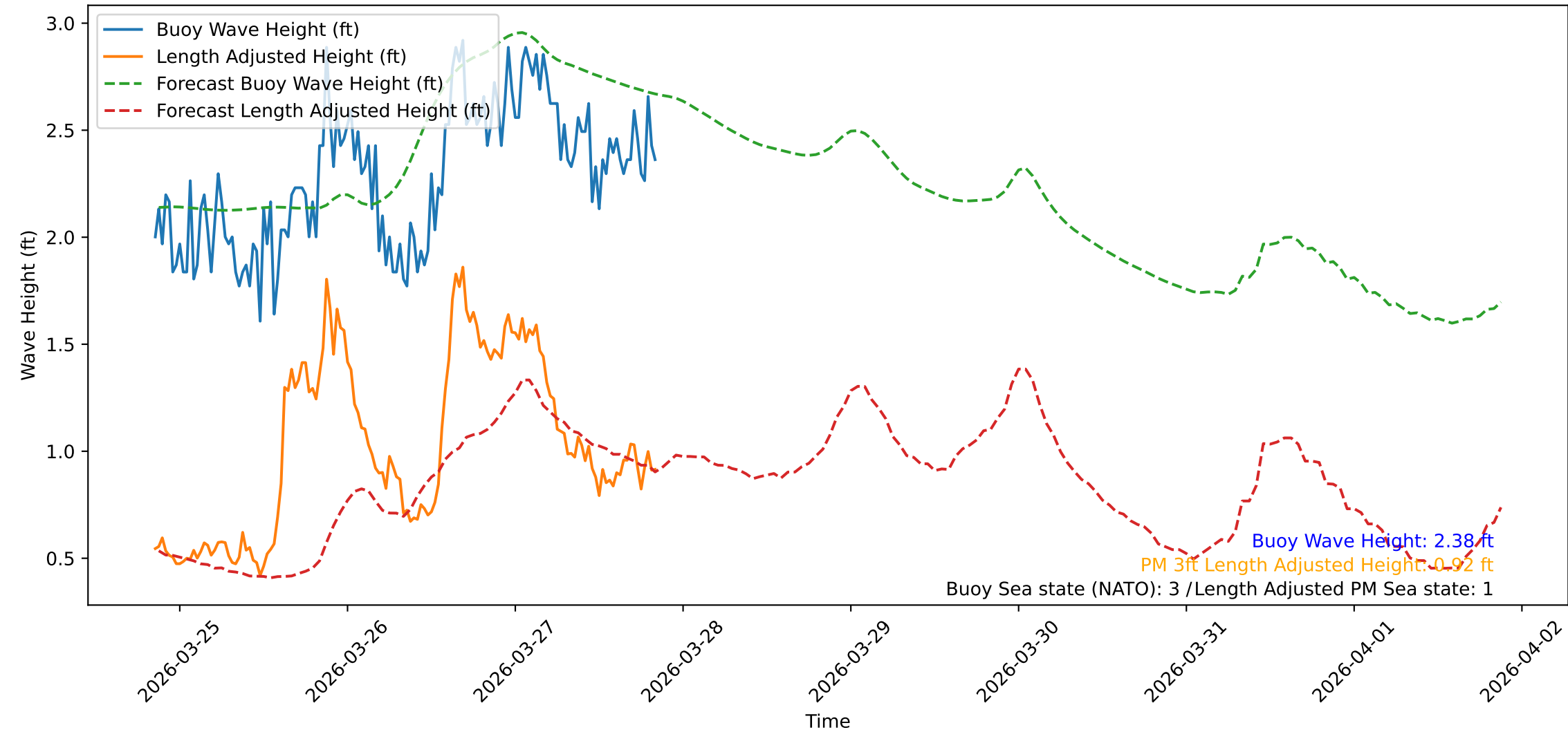
Wave Heights over Time for Oceanside Harbor at 2026-03-27 20:30:31
