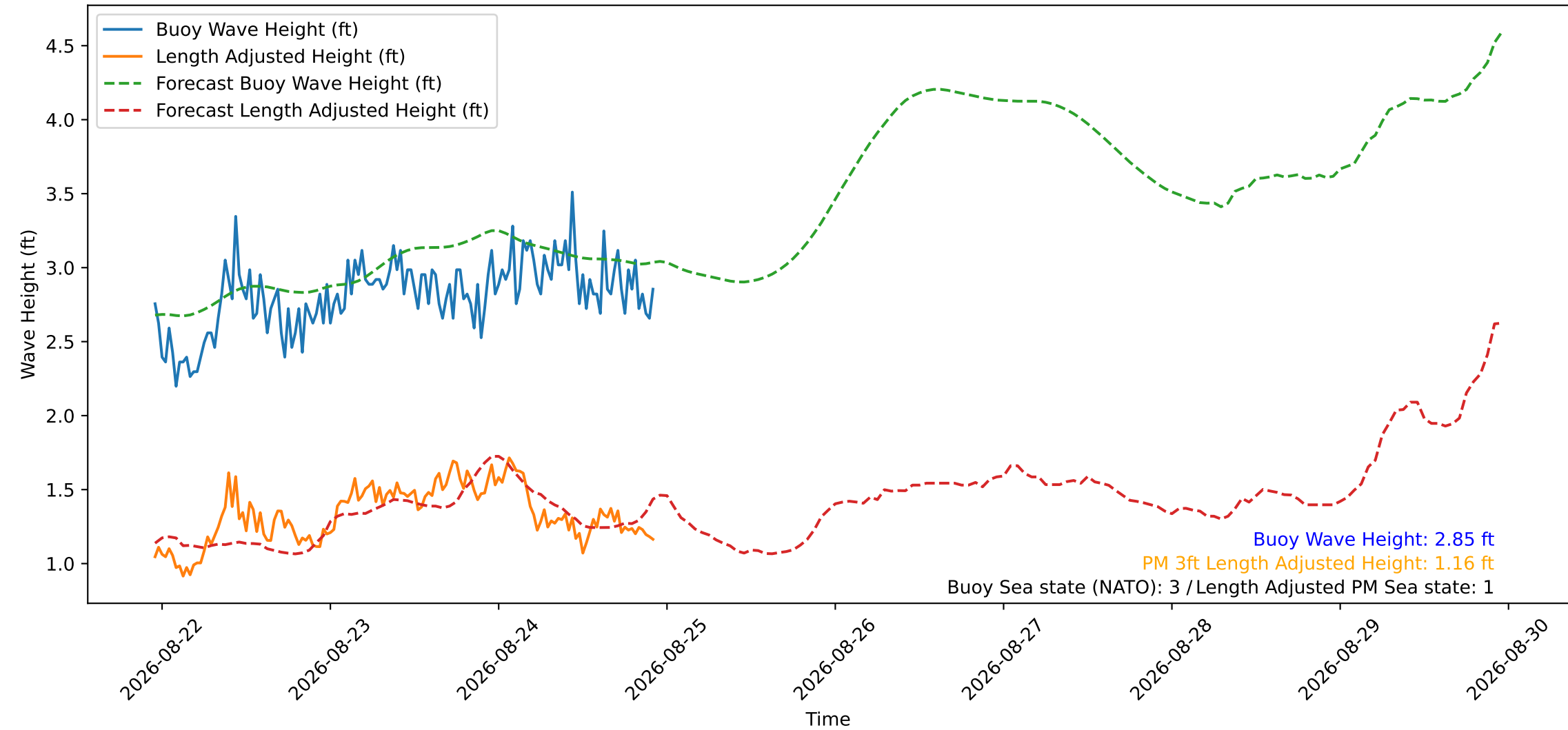
Wave Heights over Time for Oceanside Harbor at 2026-08-24 22:50:30
