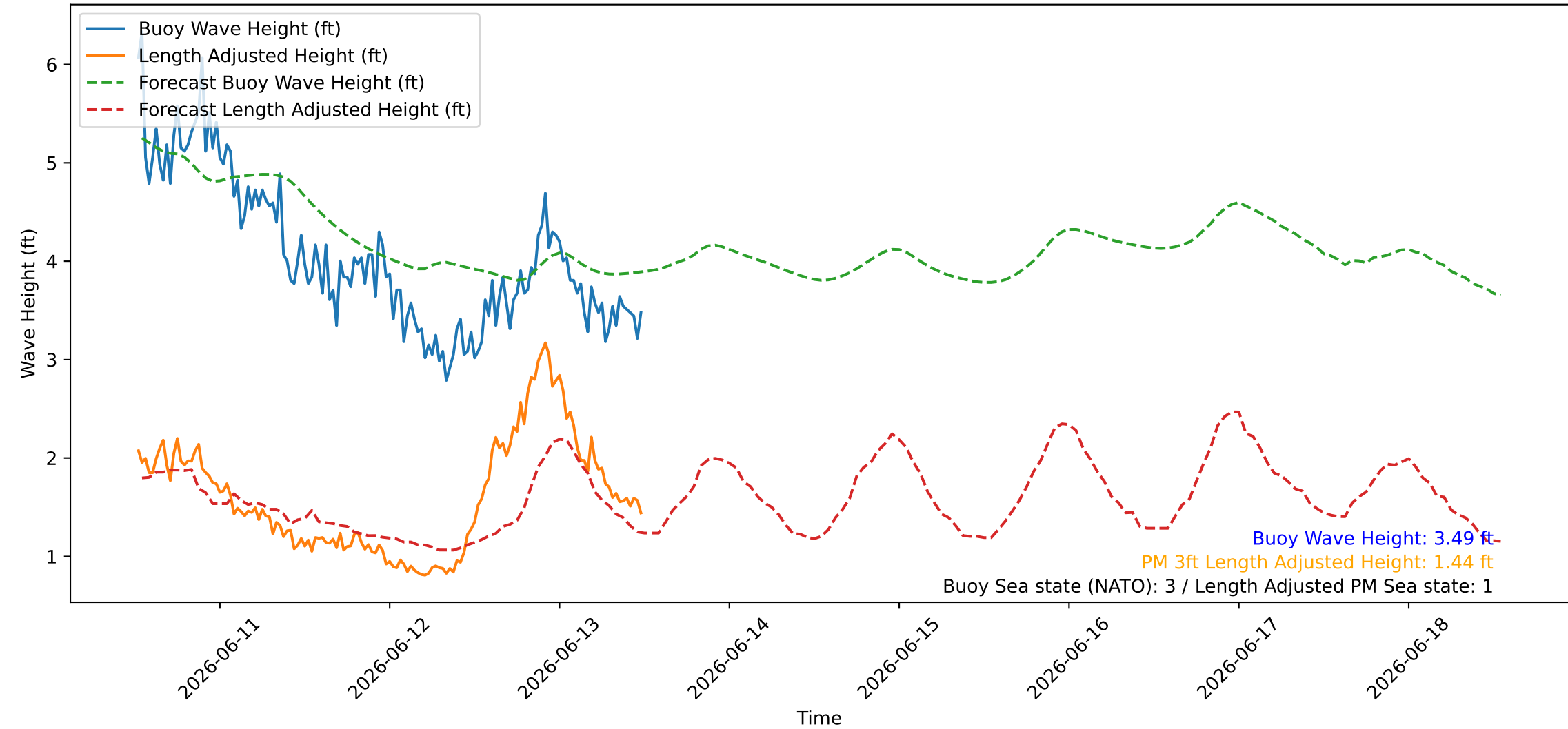
Wave Heights over Time for Oceanside Harbor at 2026-06-13 12:30:27
