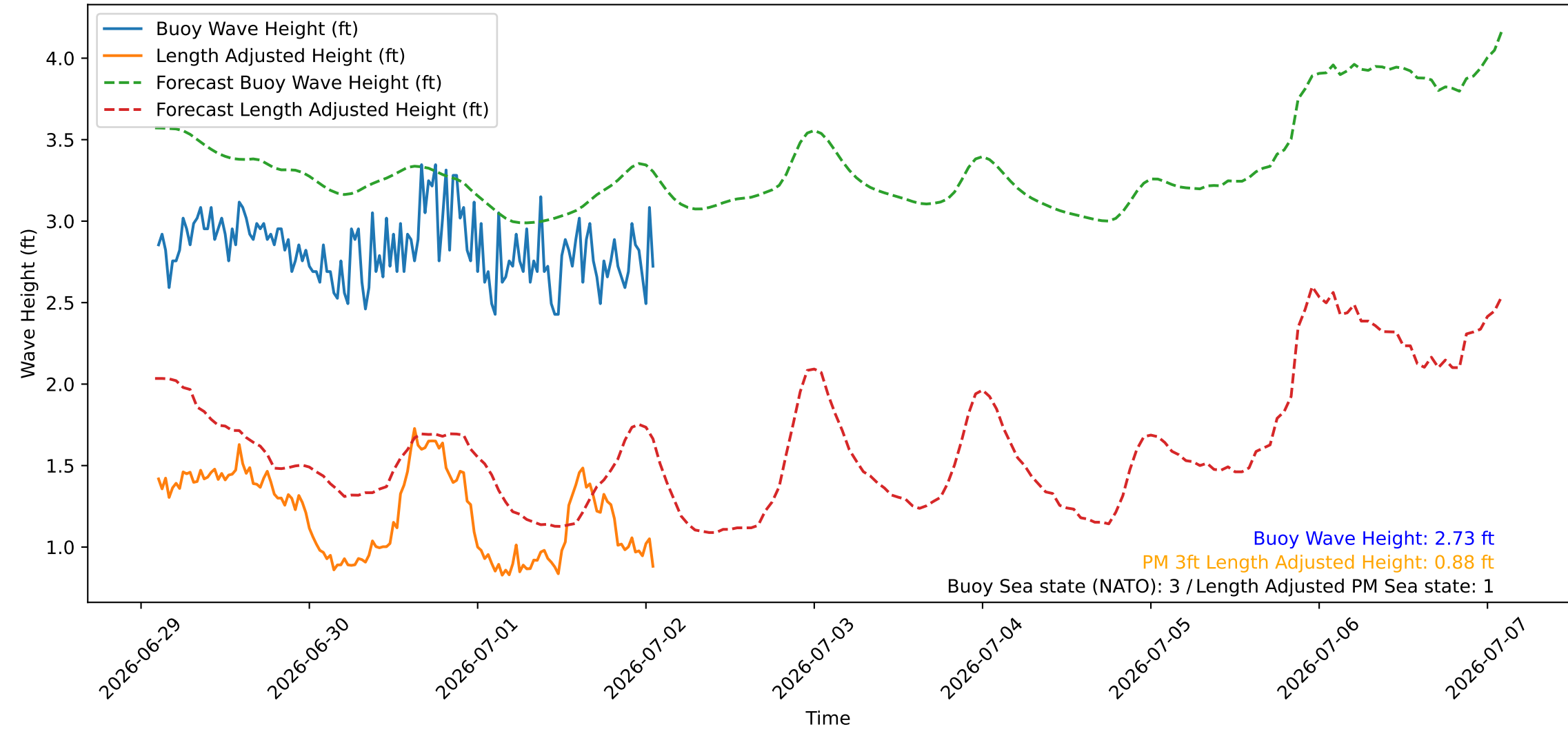
Wave Heights over Time for Red Beach at 2026-07-02 02:00:47
