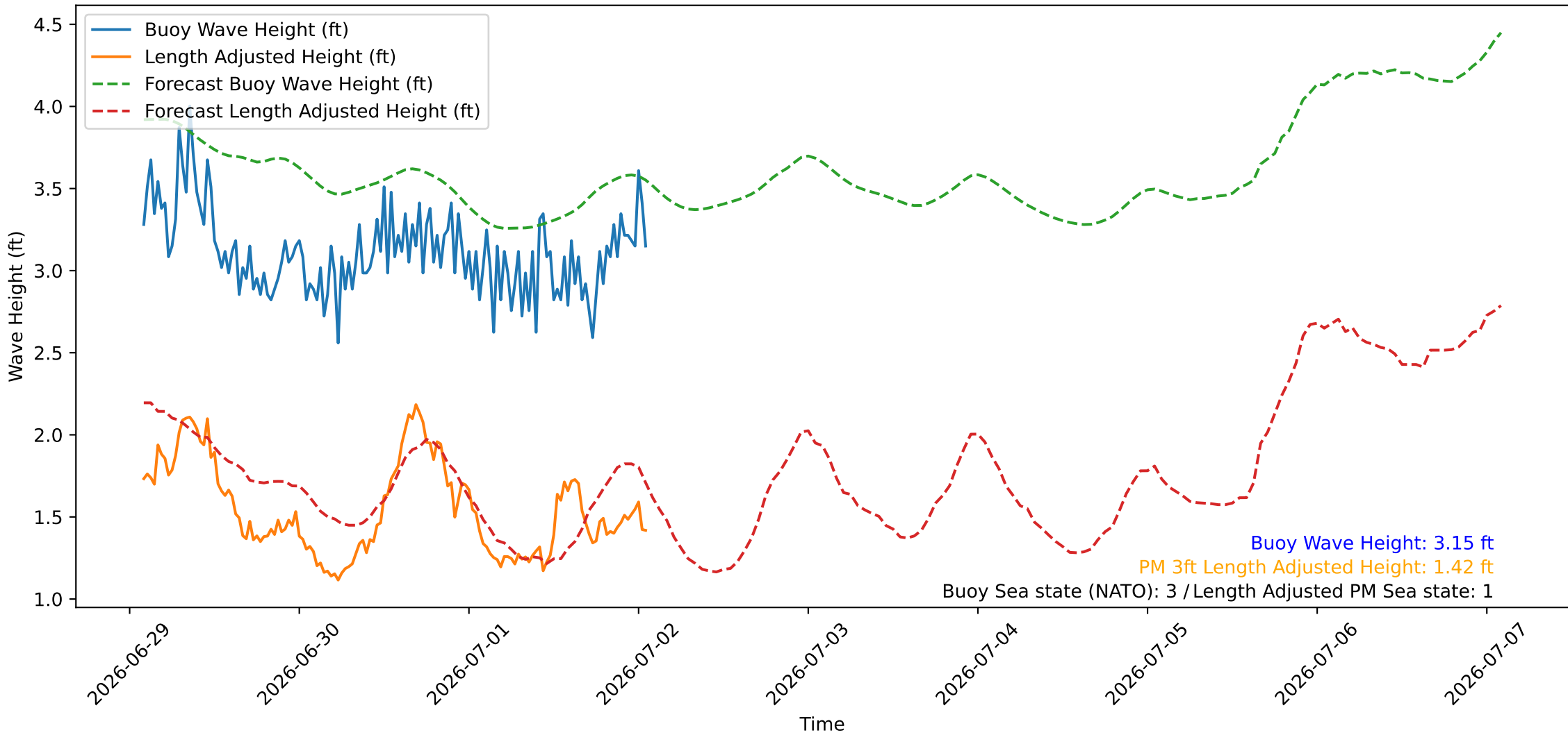
Wave Heights over Time for Oceanside Harbor at 2026-07-02 02:00:26
