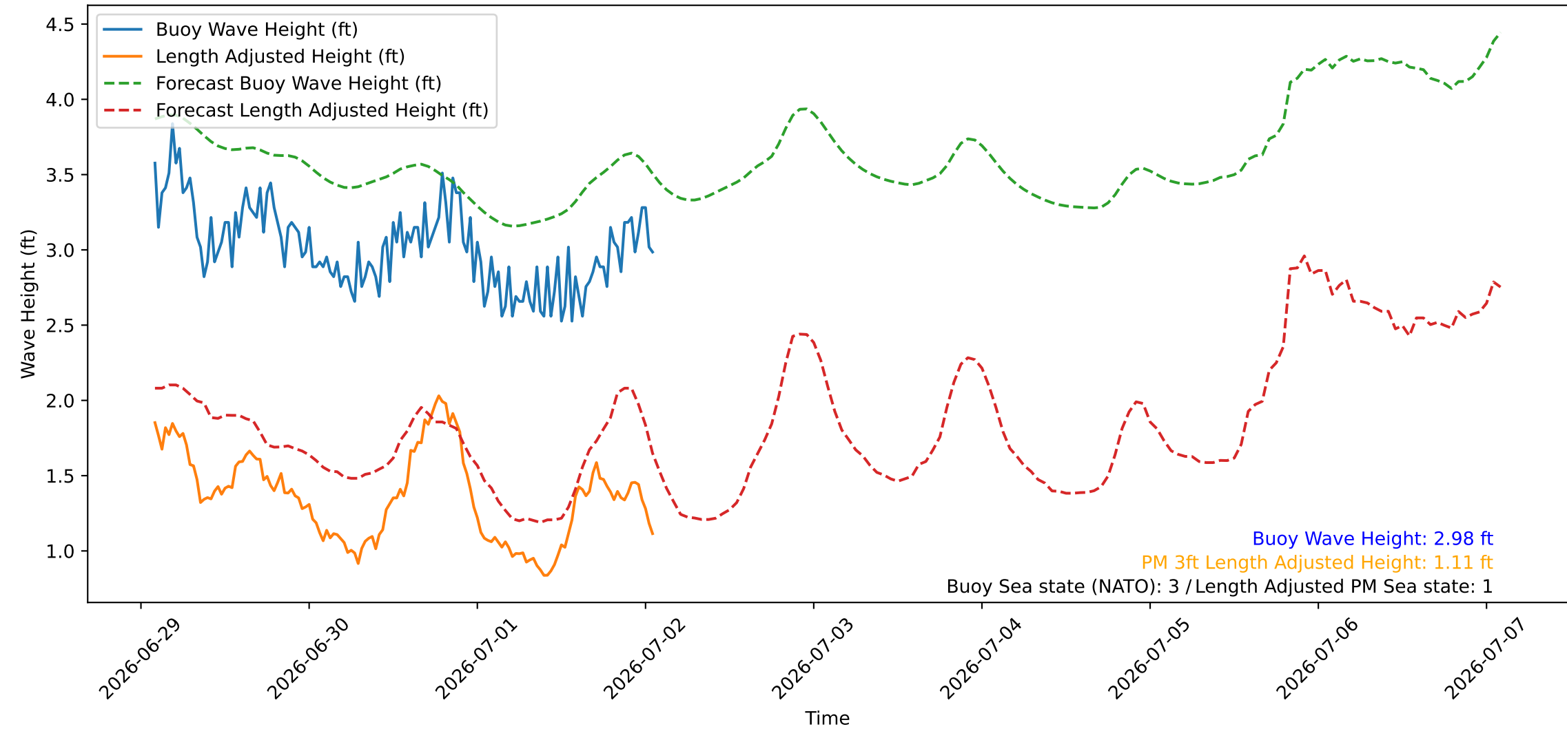
Wave Heights over Time for Green Beach at 2026-07-02 02:01:10
