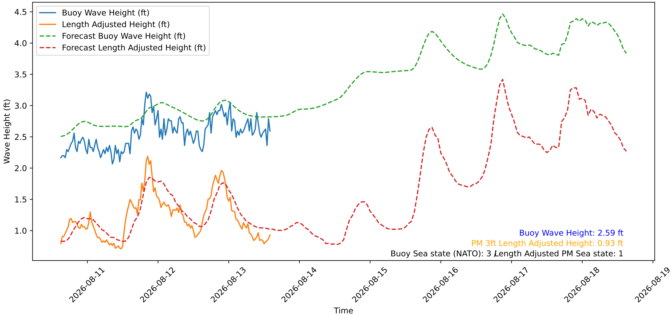
Wave Heights over Time for Green Beach at 2026-08-13 14:51:10
