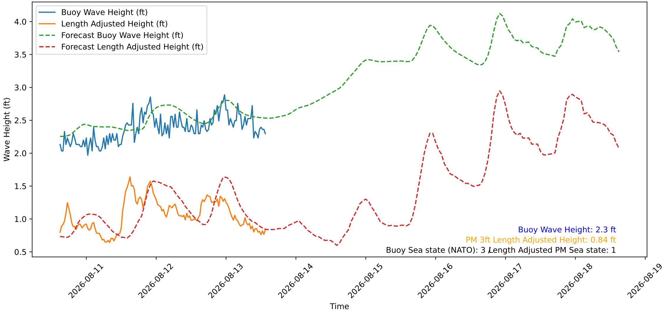
Wave Heights over Time for Red Beach at 2026-08-13 14:50:47
