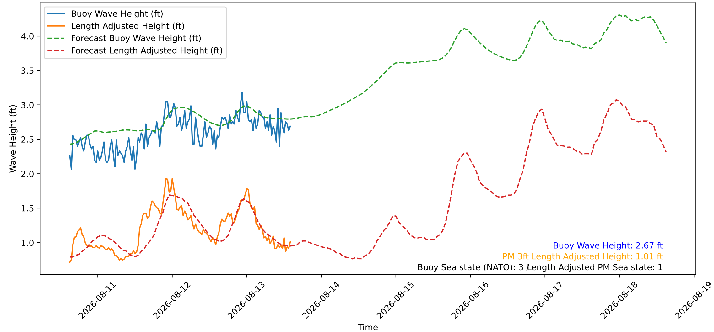
Wave Heights over Time for Oceanside Harbor at 2026-08-13 14:50:26
