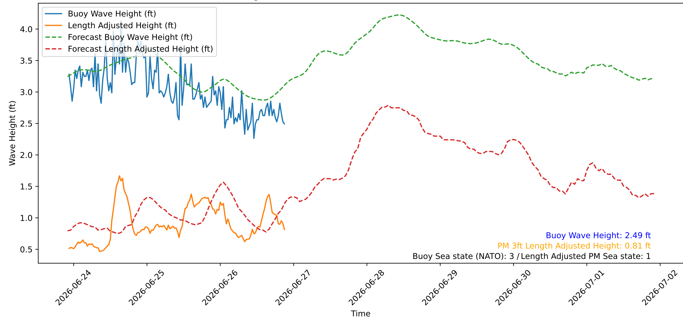
Wave Heights over Time for Red Beach at 2026-06-26 22:00:46
