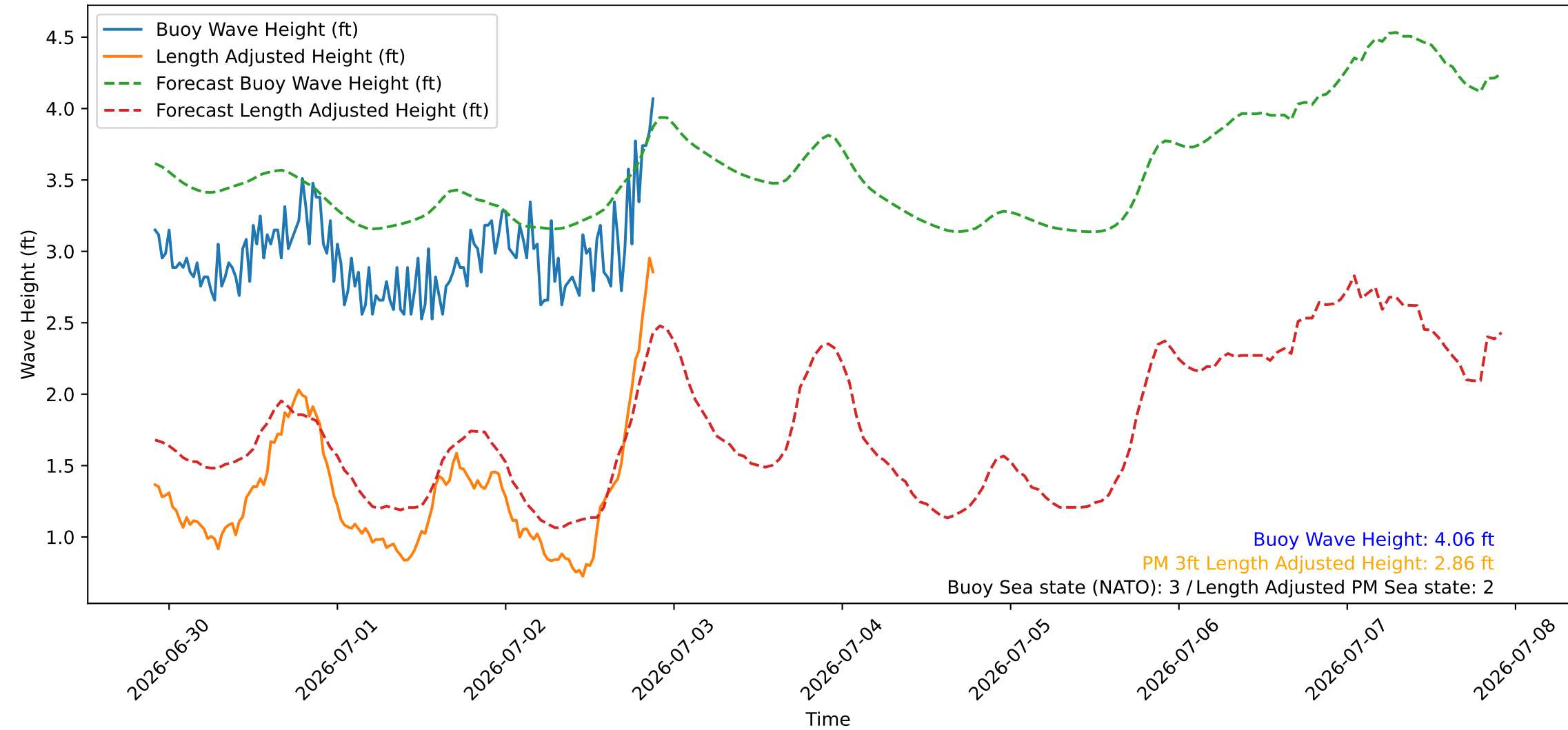
Wave Heights over Time for Green Beach at 2026-07-02 22:01:08
