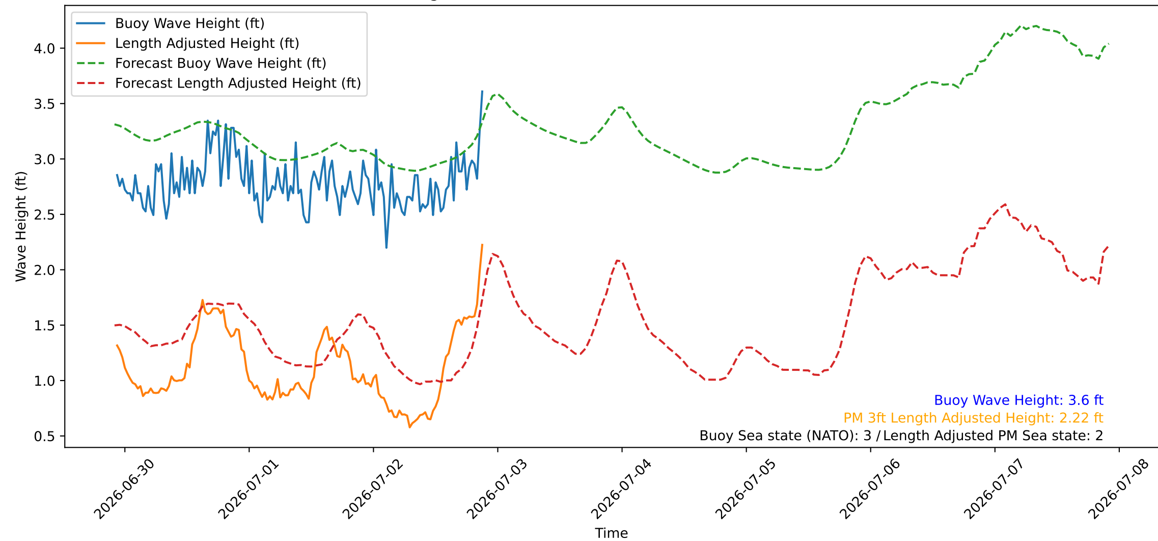
Wave Heights over Time for Red Beach at 2026-07-02 22:00:46
