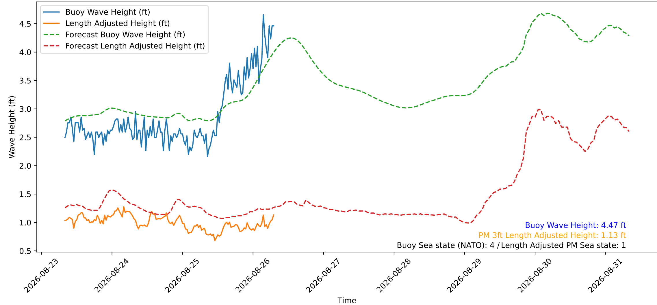
Wave Heights over Time for Red Beach at 2026-08-26 07:40:50
