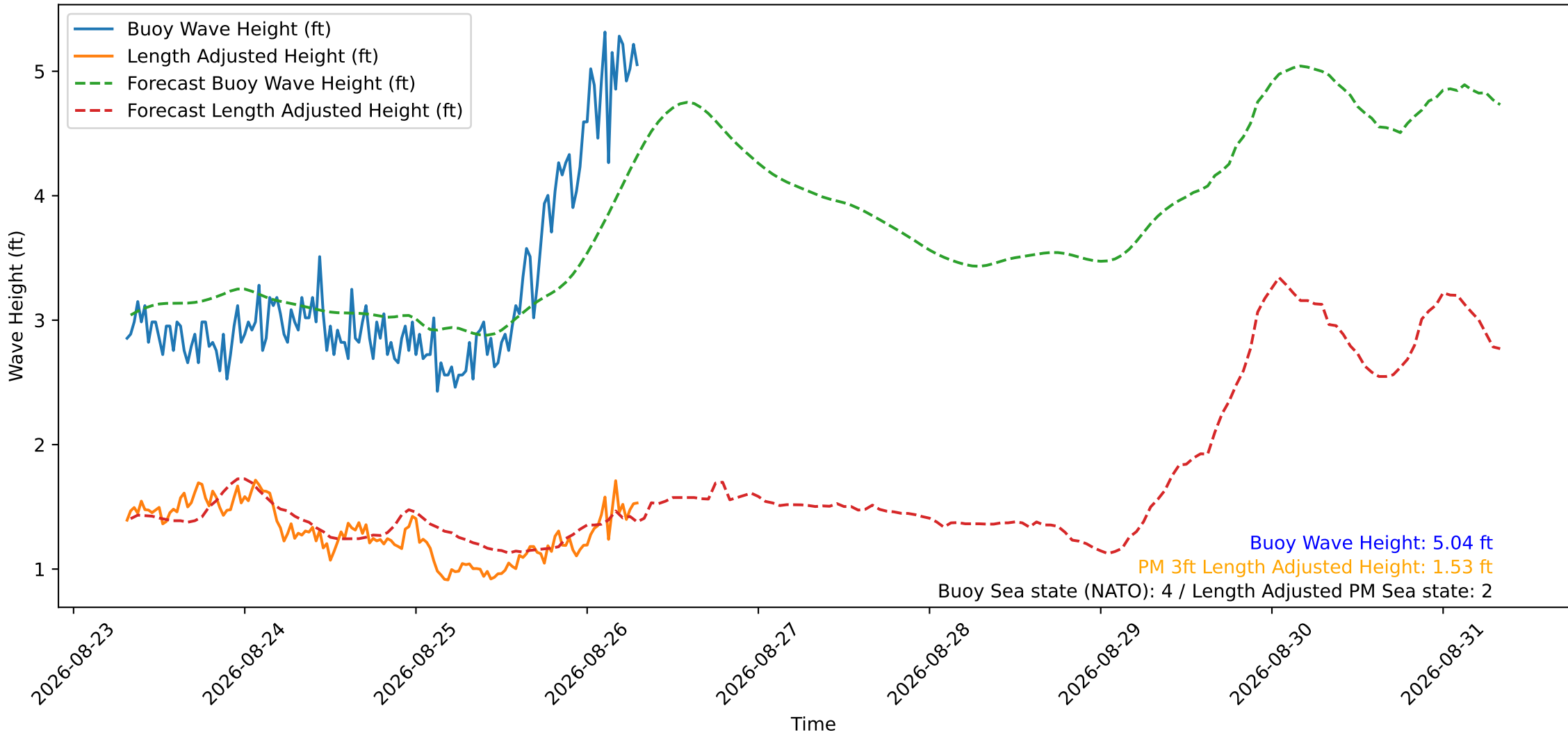
Wave Heights over Time for Oceanside Harbor at 2026-08-26 07:40:30
