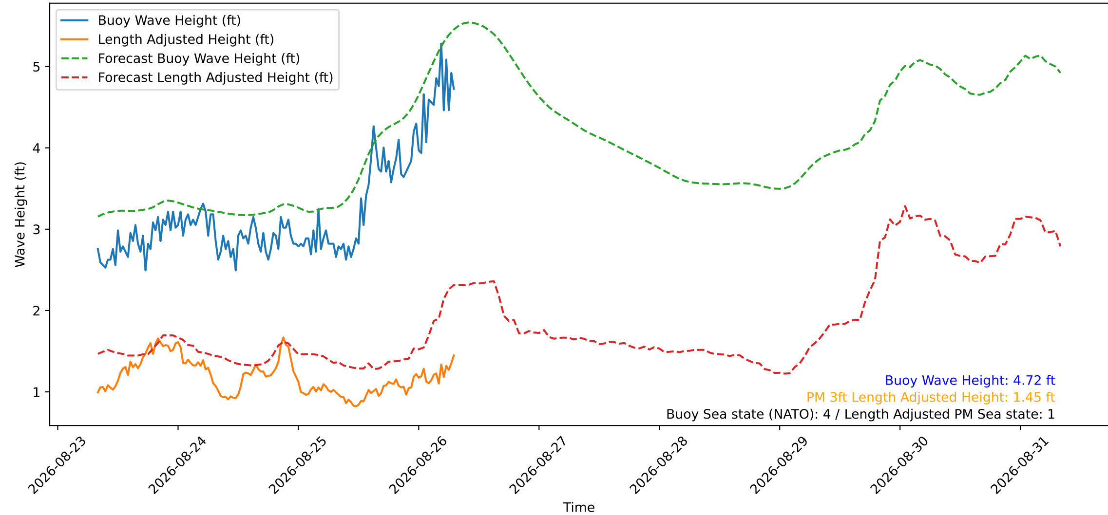
Wave Heights over Time for Green Beach at 2026-08-26 07:41:13
