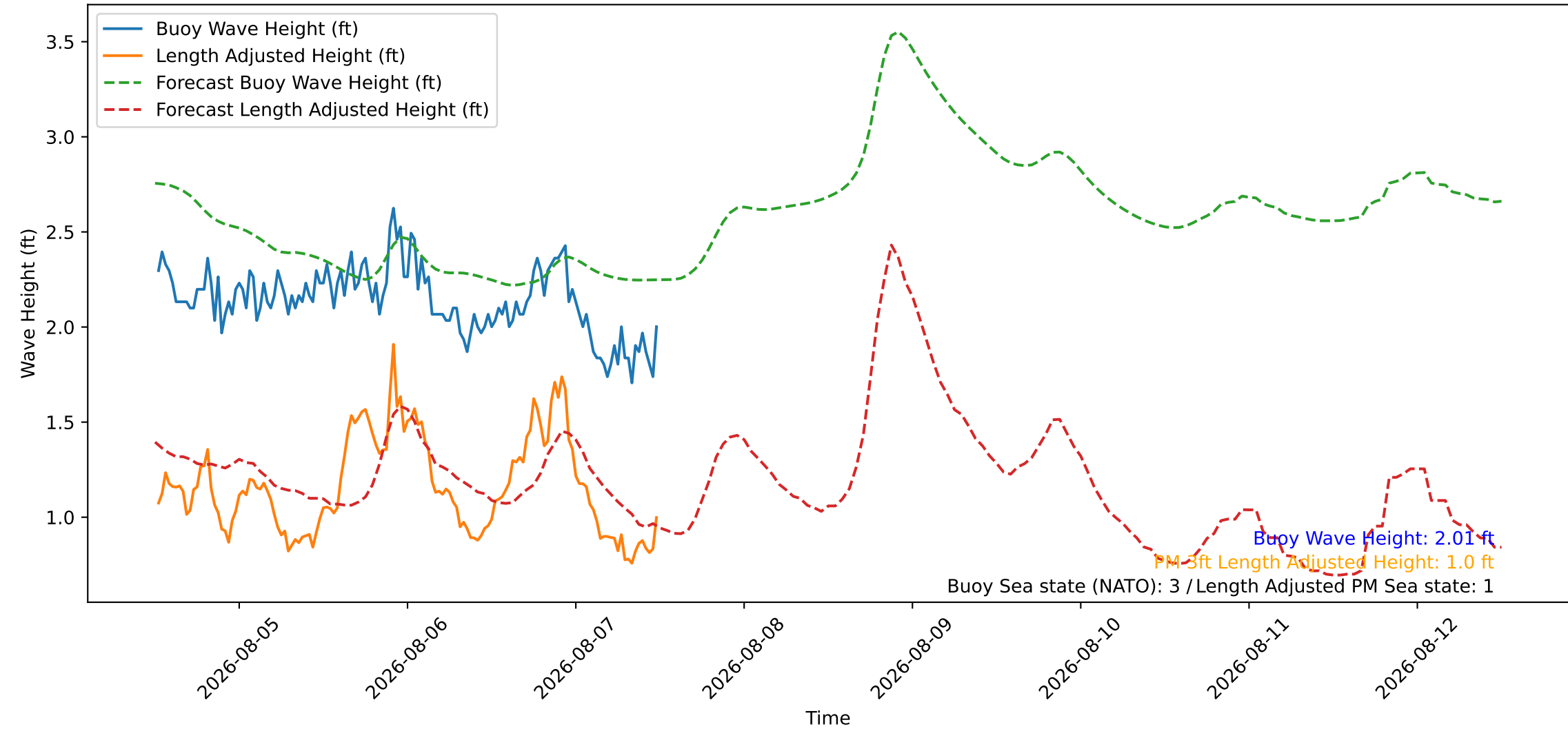
Wave Heights over Time for Green Beach at 2026-08-07 12:21:10
