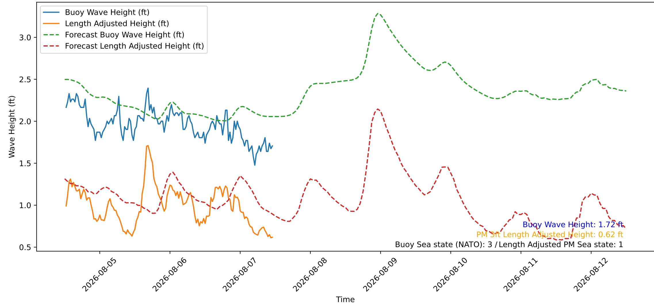
Wave Heights over Time for Red Beach at 2026-08-07 12:20:48
