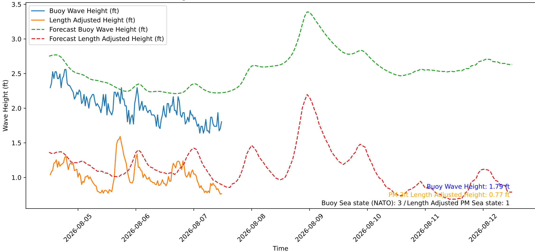
Wave Heights over Time for Oceanside Harbor at 2026-08-07 12:20:27
