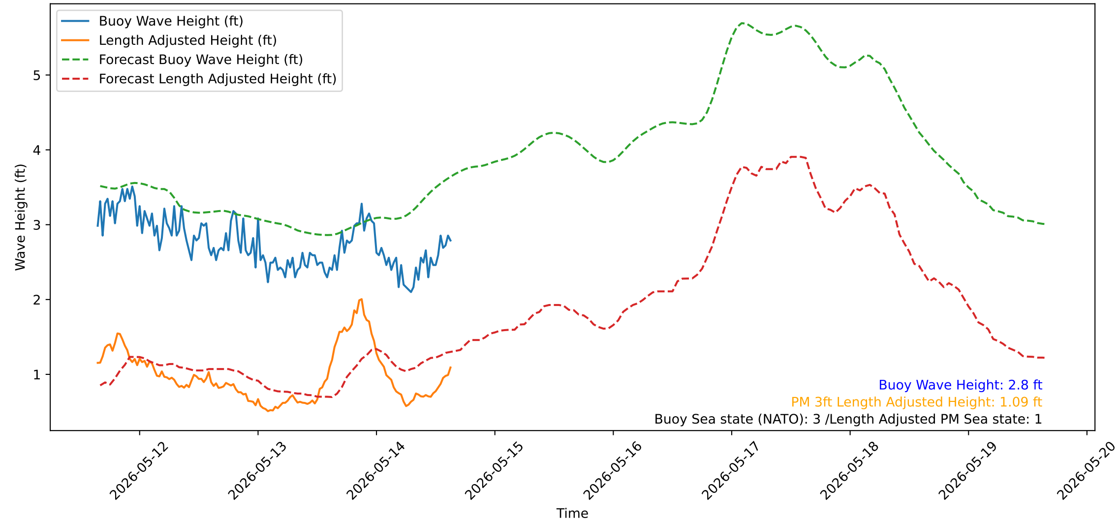
Wave Heights over Time for Green Beach at 2026-05-14 15:41:14
