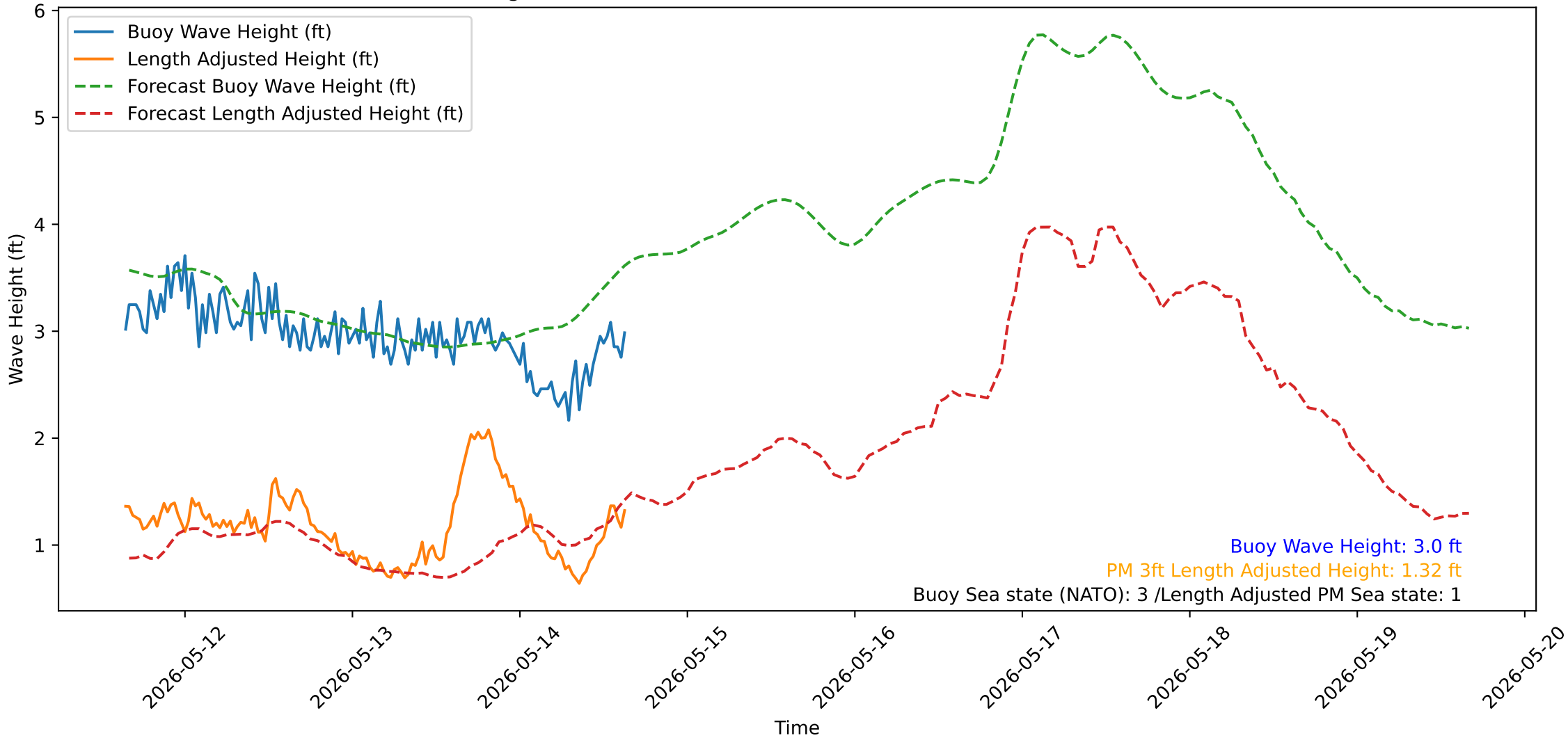
Wave Heights over Time for Oceanside Harbor at 2026-05-14 15:40:31
