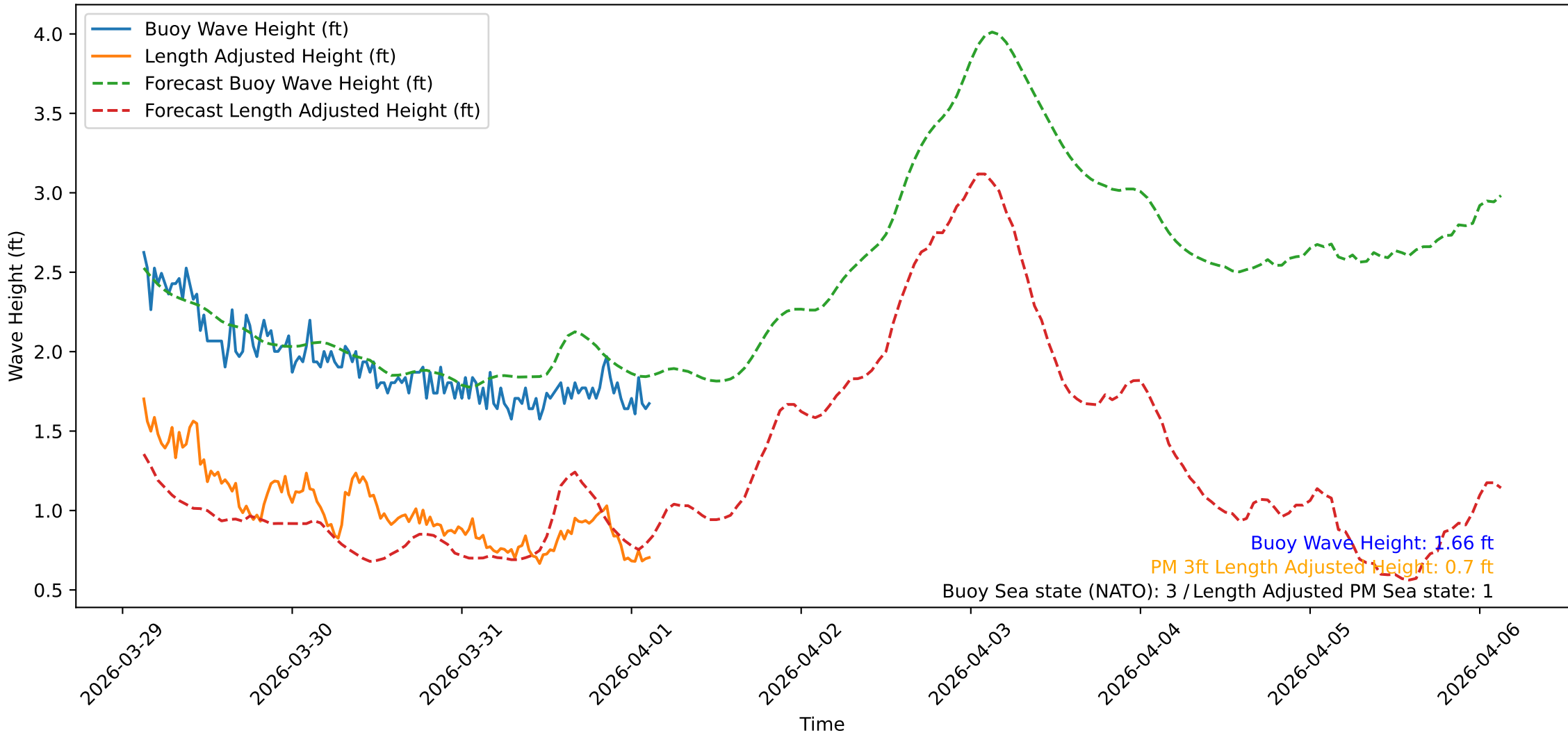
Wave Heights over Time for Oceanside Harbor at 2026-04-01 03:10:32
