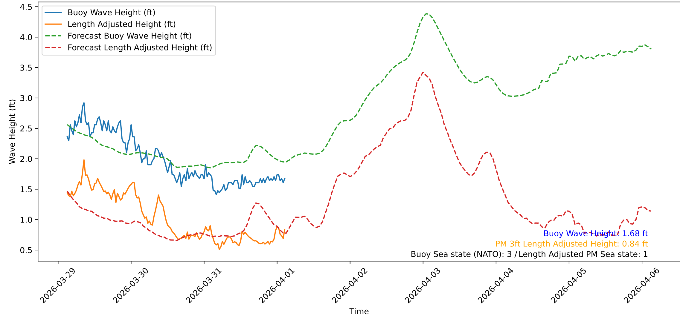
Wave Heights over Time for Green Beach at 2026-04-01 03:11:10
