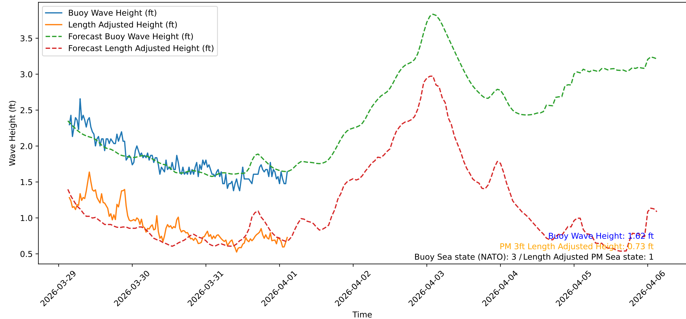
Wave Heights over Time for Red Beach at 2026-04-01 03:10:48
