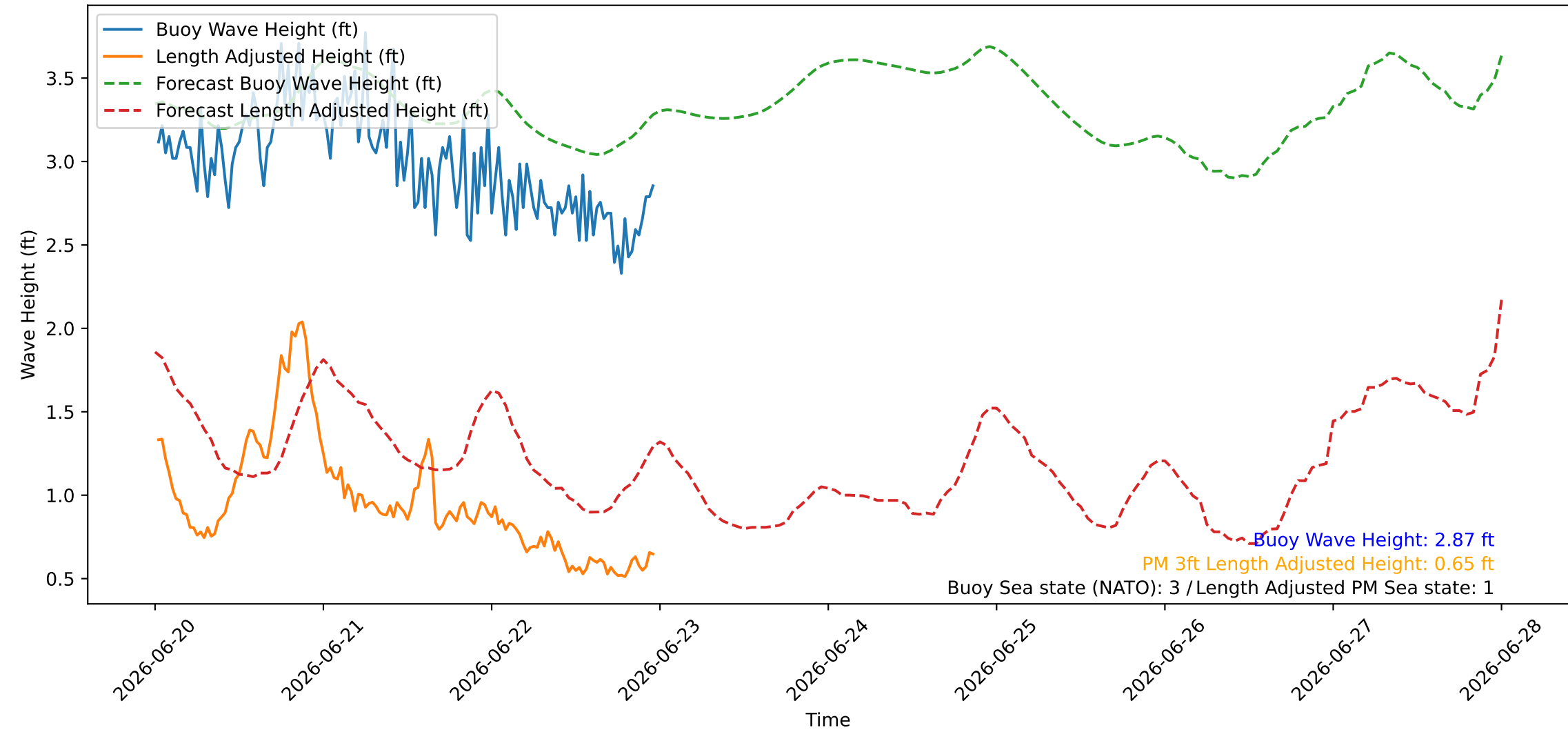
Wave Heights over Time for Red Beach at 2026-06-23 00:00:45
