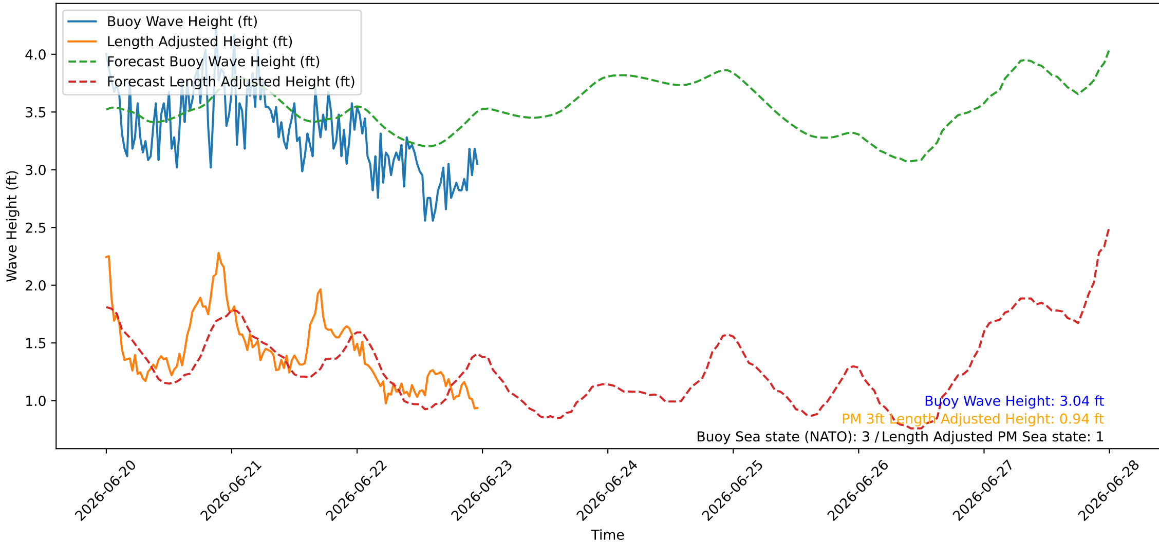
Wave Heights over Time for Oceanside Harbor at 2026-06-23 00:00:26
