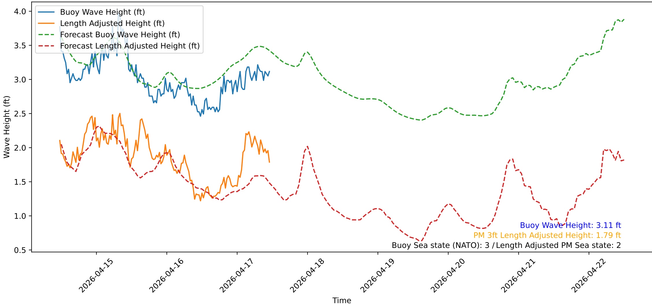
Wave Heights over Time for Green Beach at 2026-04-17 11:41:14
