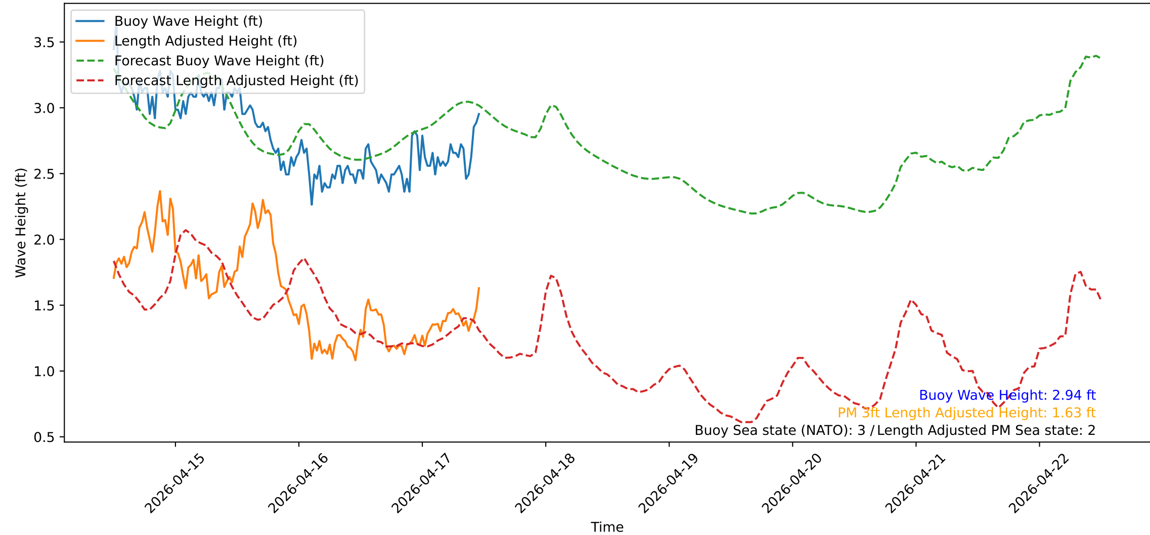
Wave Heights over Time for Red Beach at 2026-04-17 11:40:51
