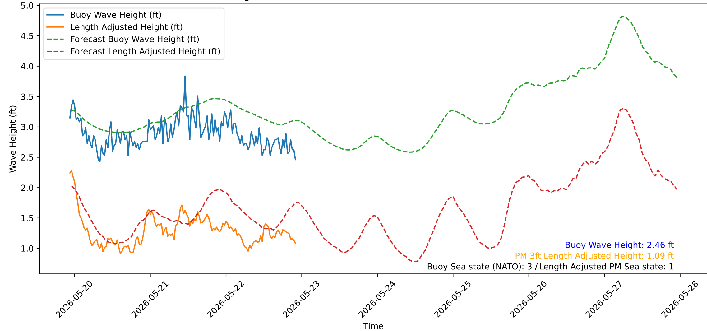
Wave Heights over Time for Oceanside Harbor at 2026-05-22 22:30:32
