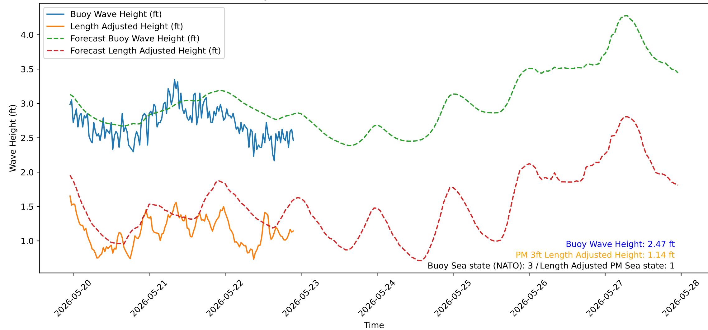
Wave Heights over Time for Red Beach at 2026-05-22 22:30:51
