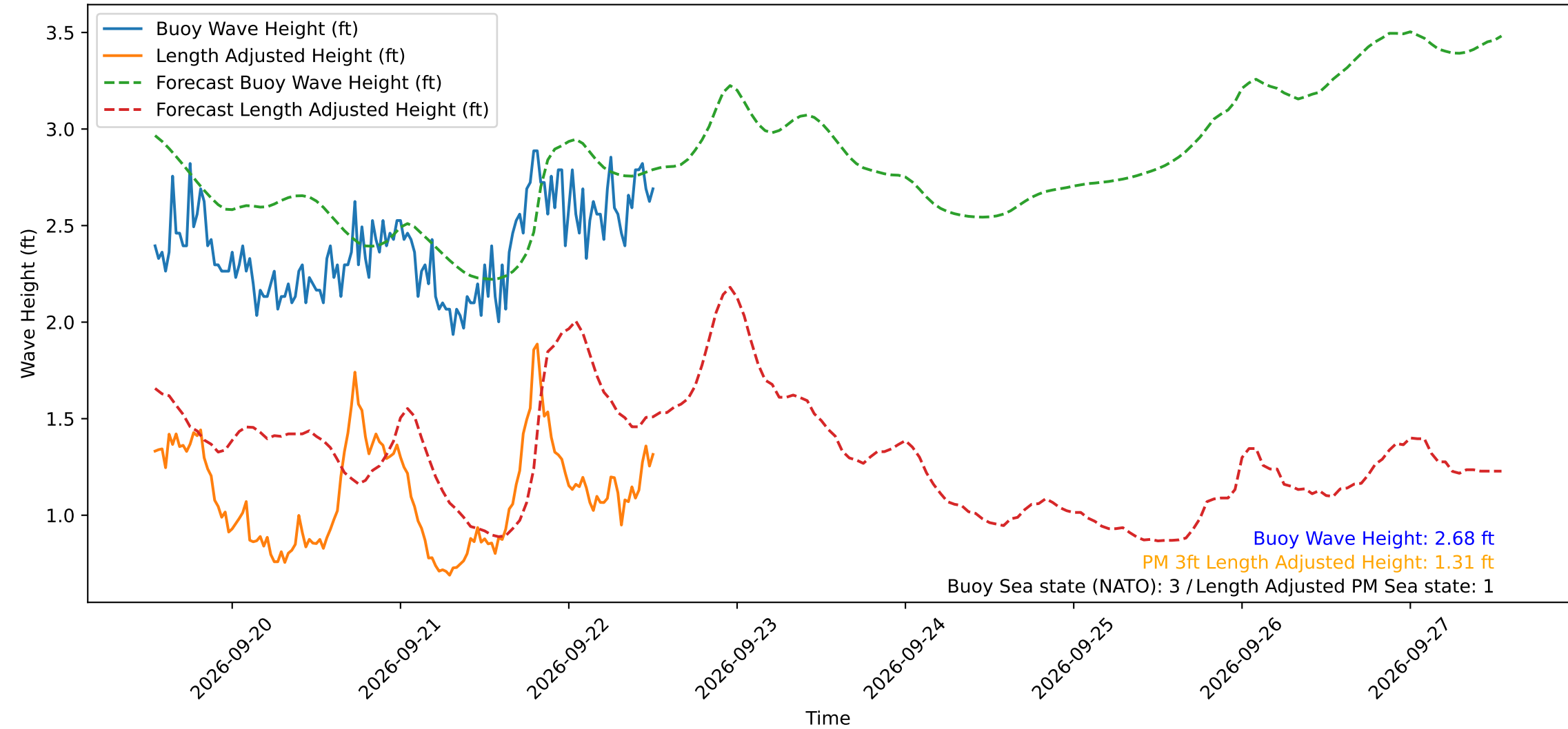
Wave Heights over Time for Red Beach at 2026-09-22 12:40:49
