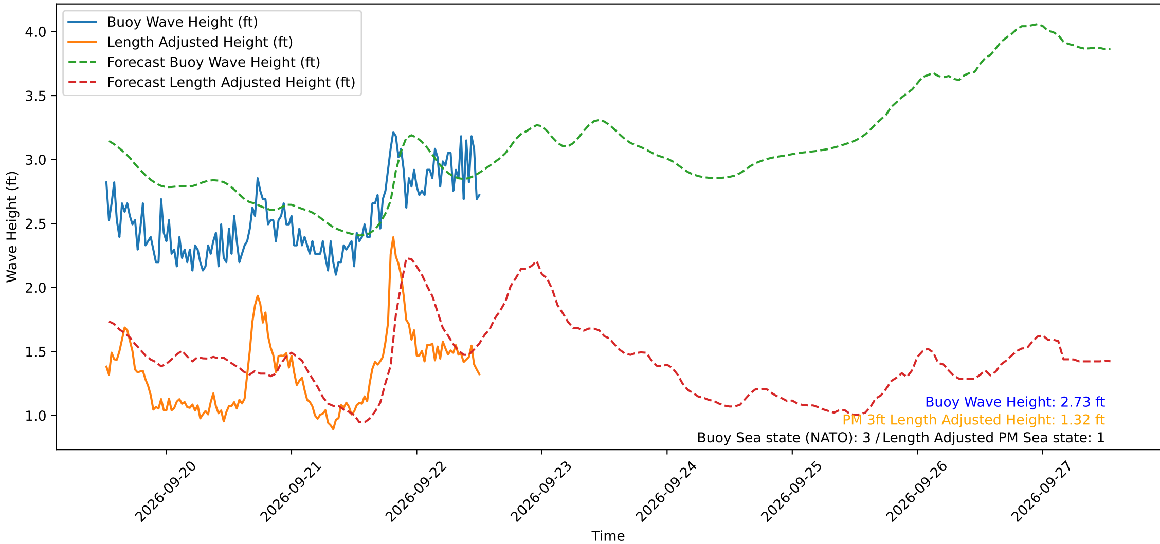
Wave Heights over Time for Oceanside Harbor at 2026-09-22 12:40:29
