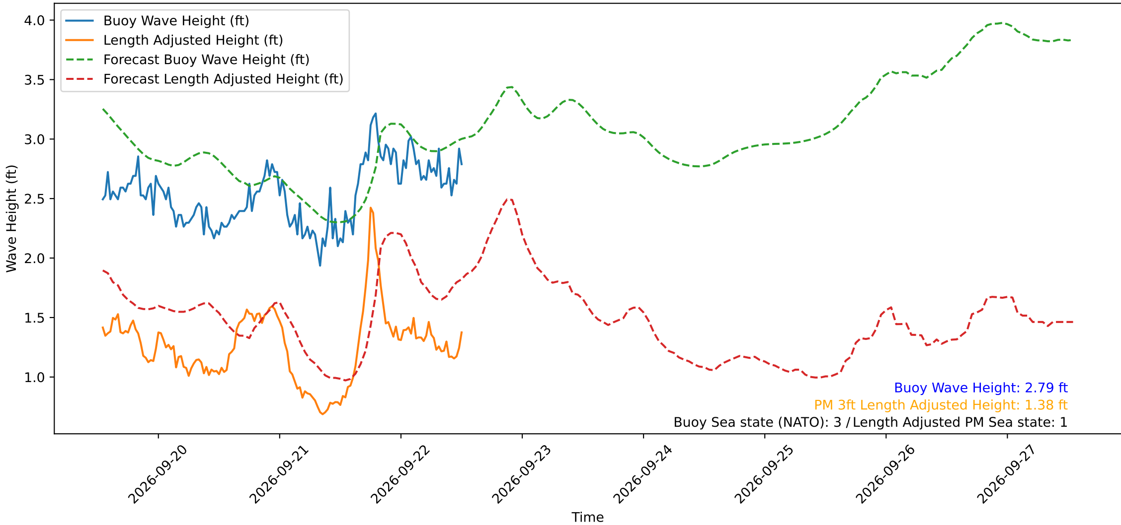
Wave Heights over Time for Green Beach at 2026-09-22 12:41:11
