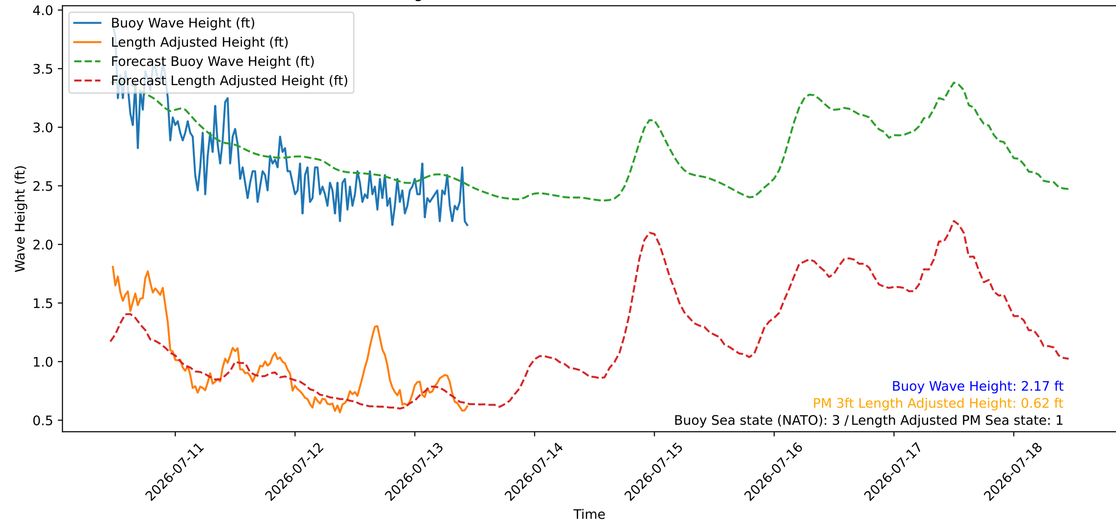
Wave Heights over Time for Red Beach at 2026-07-13 11:20:46
