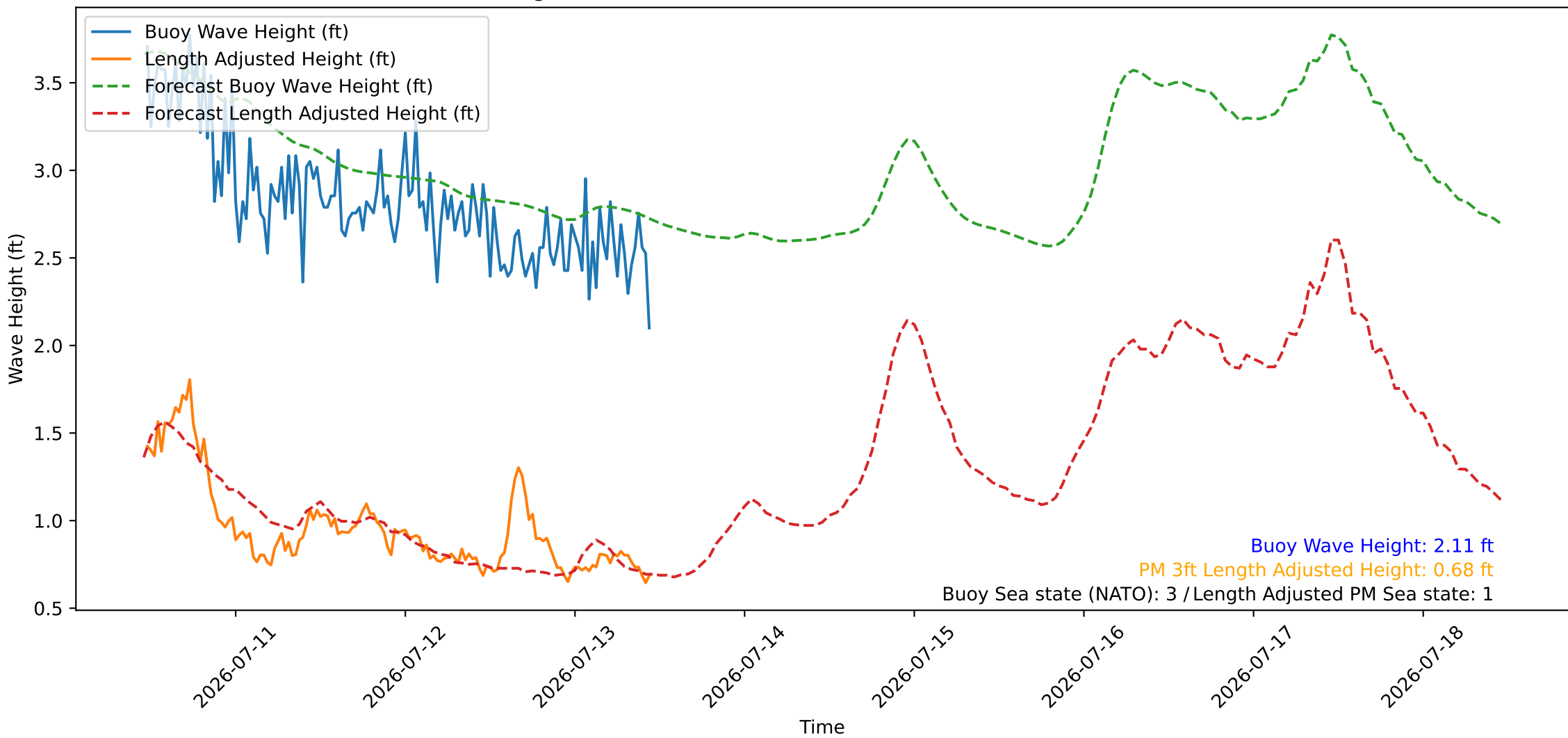
Wave Heights over Time for Oceanside Harbor at 2026-07-13 11:20:26
