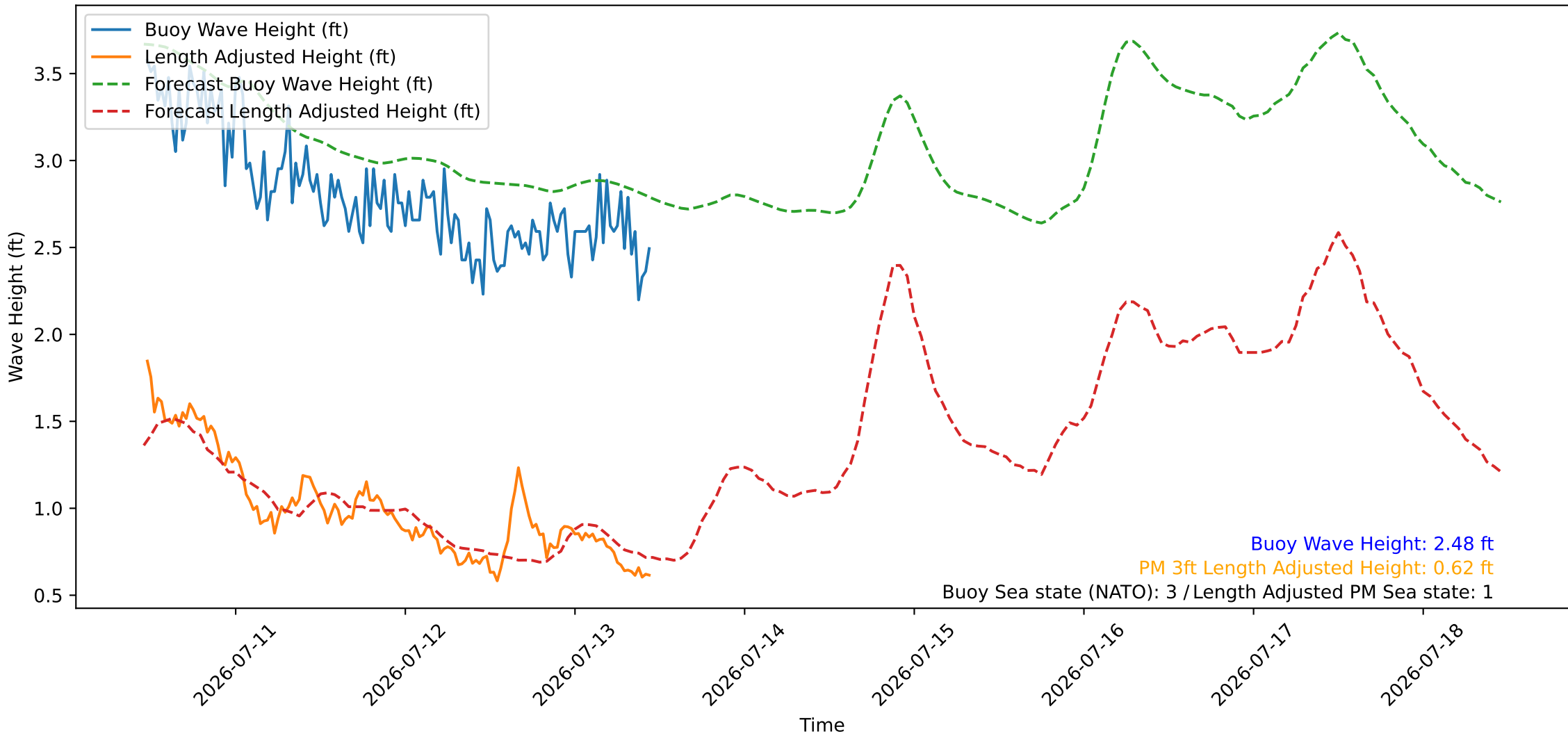
Wave Heights over Time for Green Beach at 2026-07-13 11:21:09
