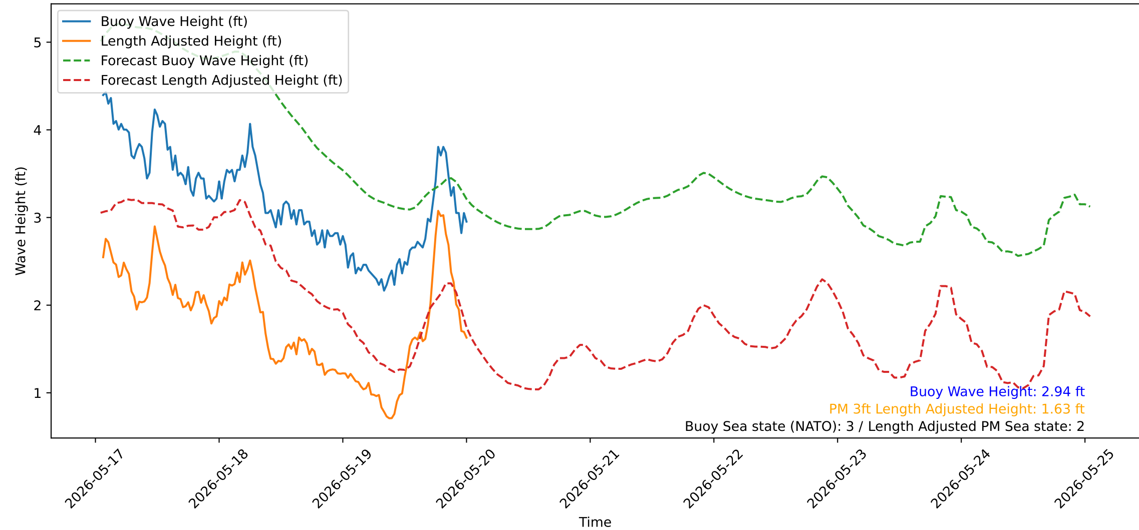
Wave Heights over Time for Green Beach at 2026-05-20 01:21:14
