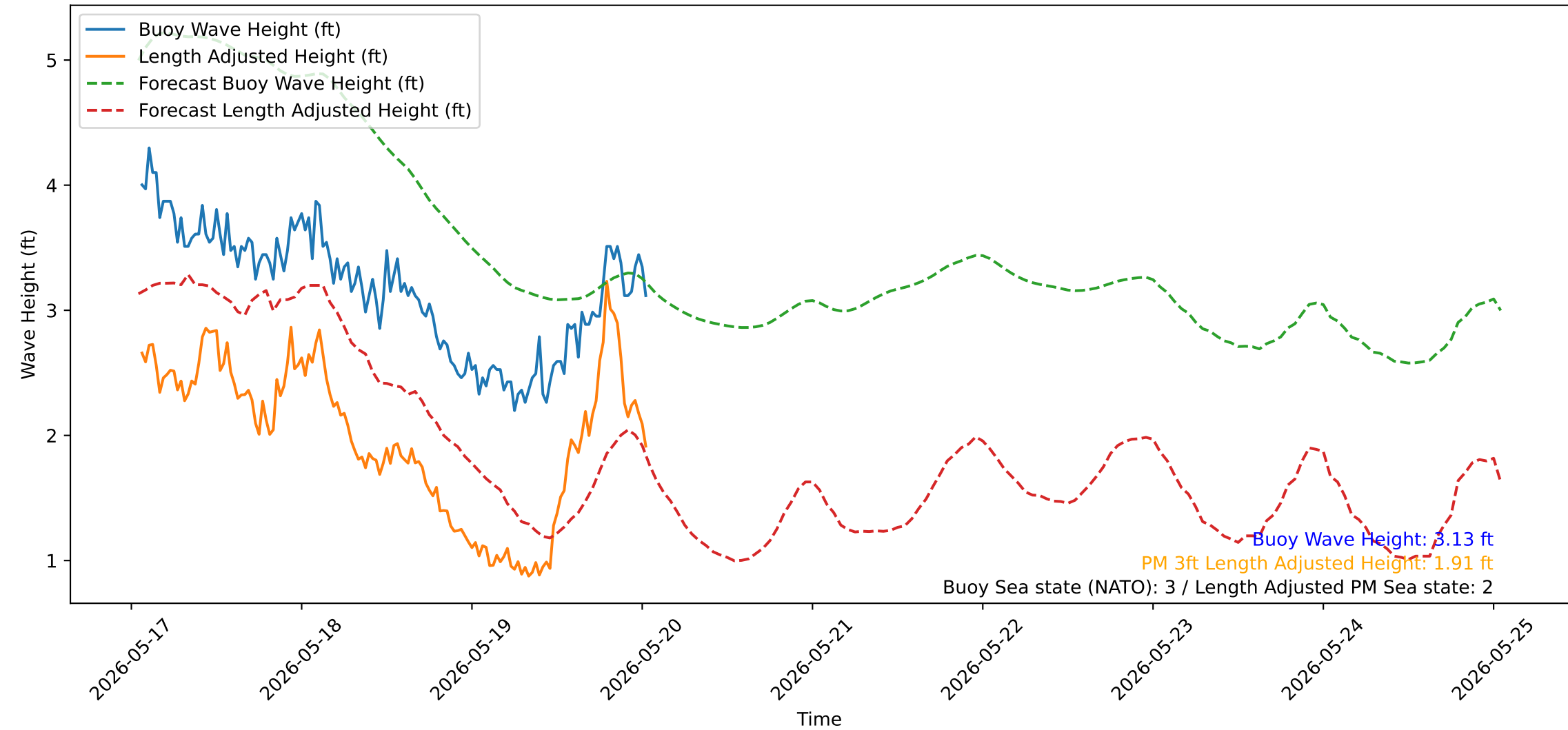
Wave Heights over Time for Oceanside Harbor at 2026-05-20 01:20:31
