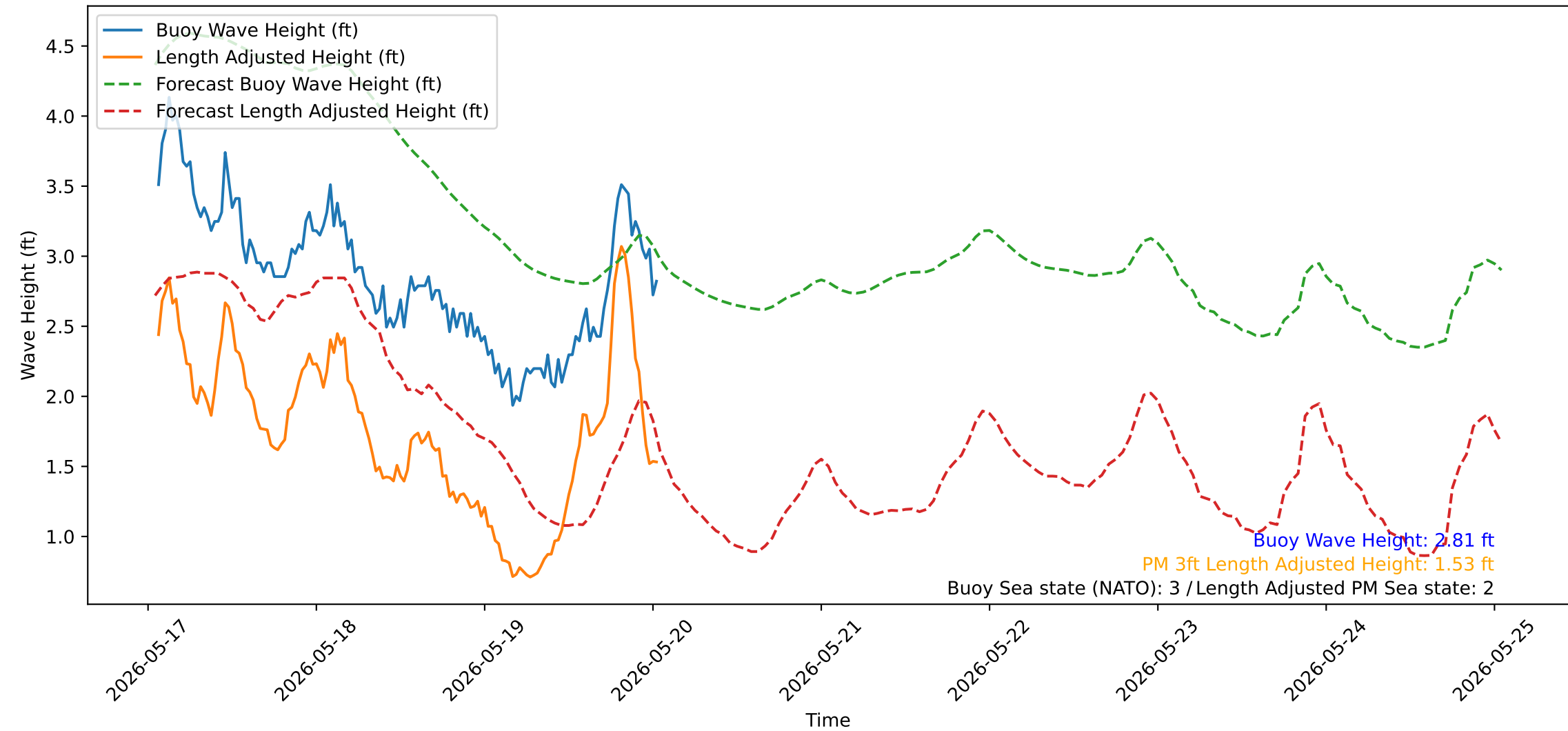
Wave Heights over Time for Red Beach at 2026-05-20 01:20:52
