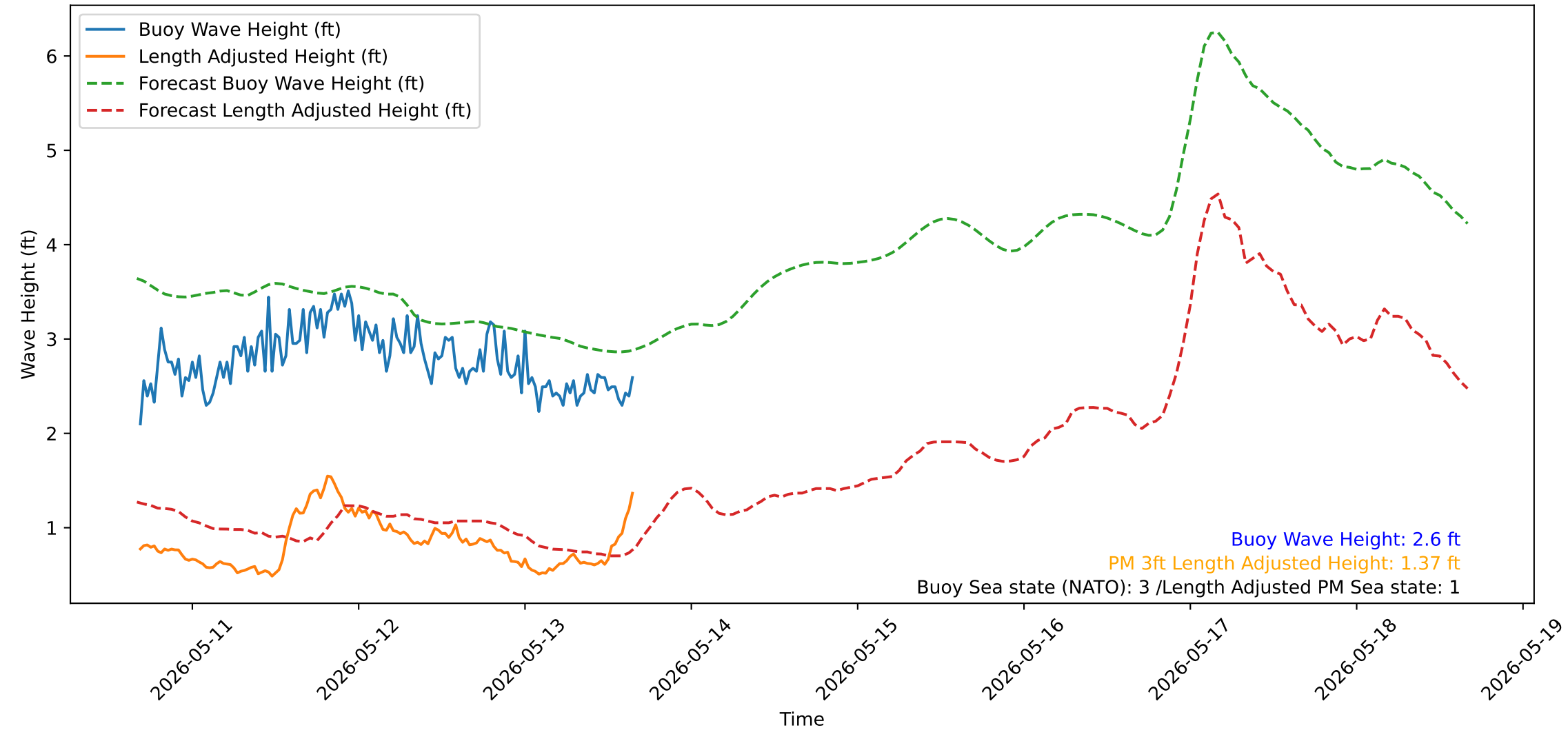
Wave Heights over Time for Green Beach at 2026-05-13 16:21:14
