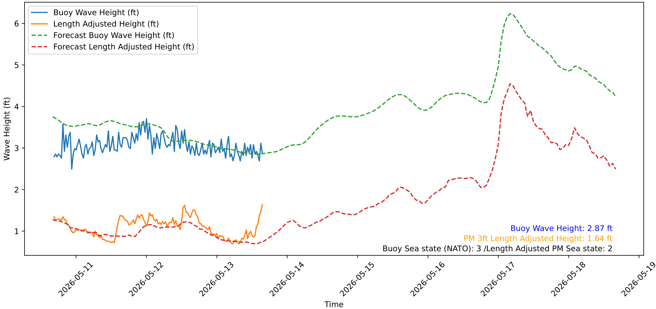
Wave Heights over Time for Oceanside Harbor at 2026-05-13 16:20:32
