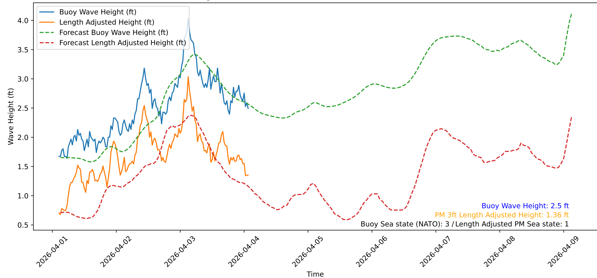
Wave Heights over Time for Oceanside Harbor at 2026-04-04 02:30:32
