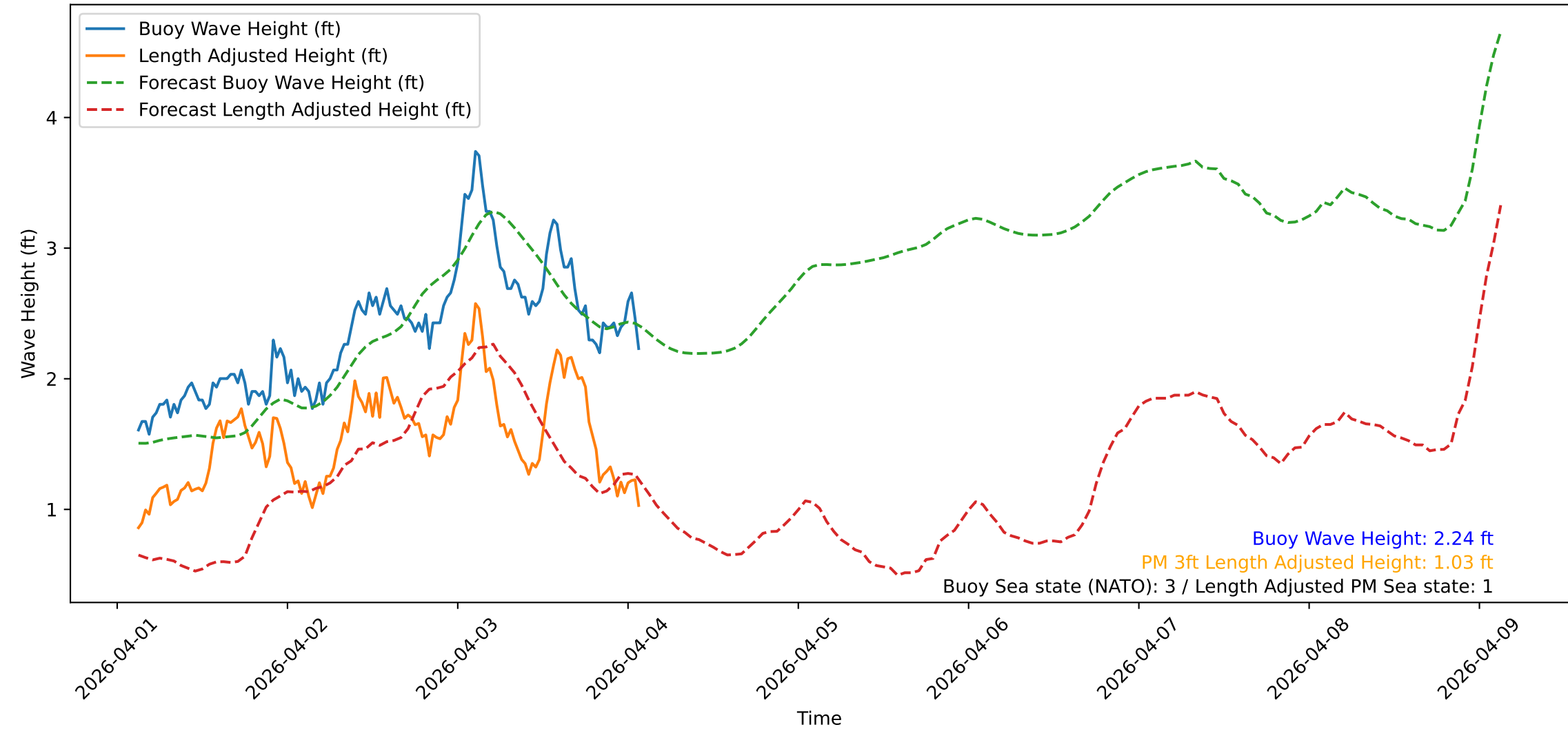
Wave Heights over Time for Red Beach at 2026-04-04 02:30:48
