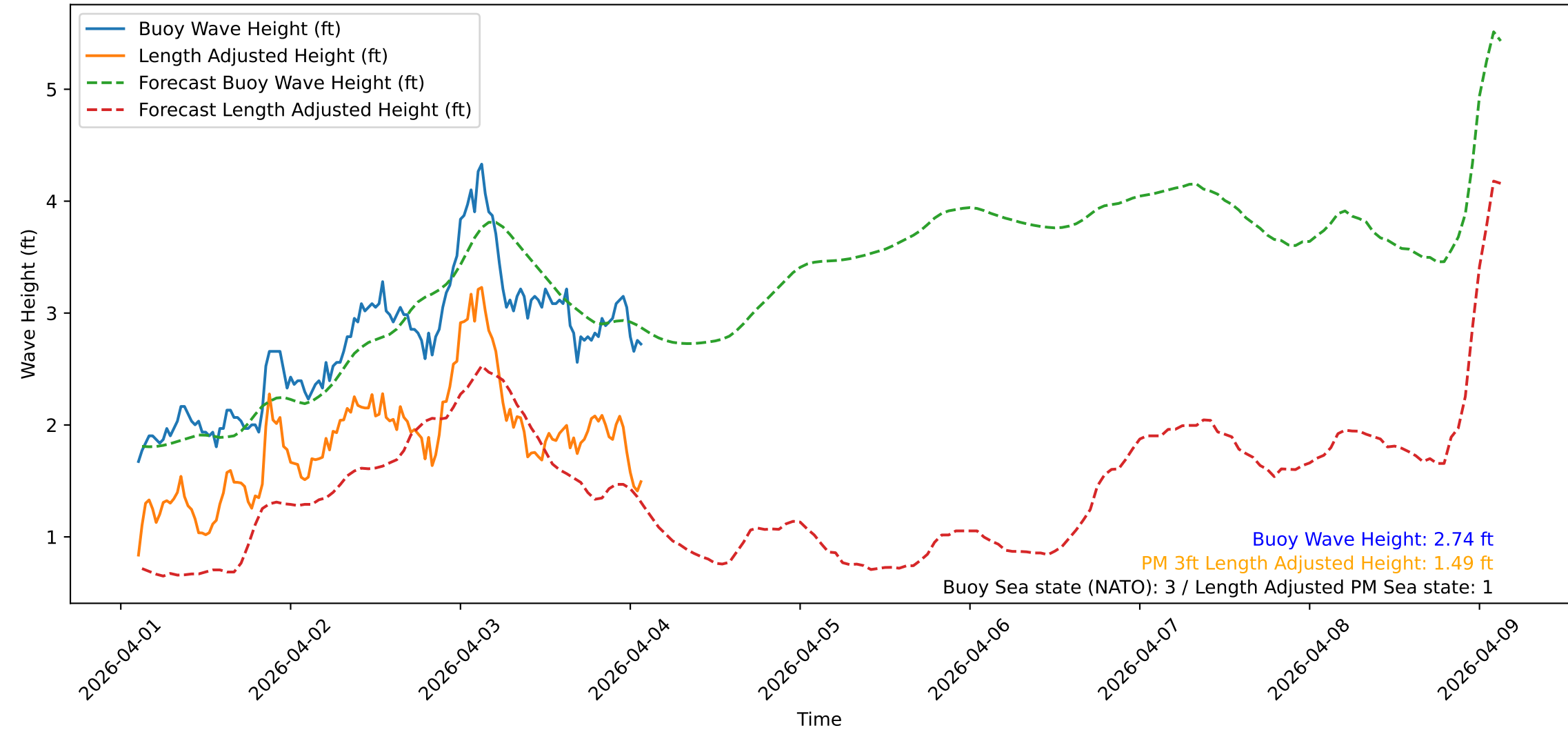
Wave Heights over Time for Green Beach at 2026-04-04 02:31:09
