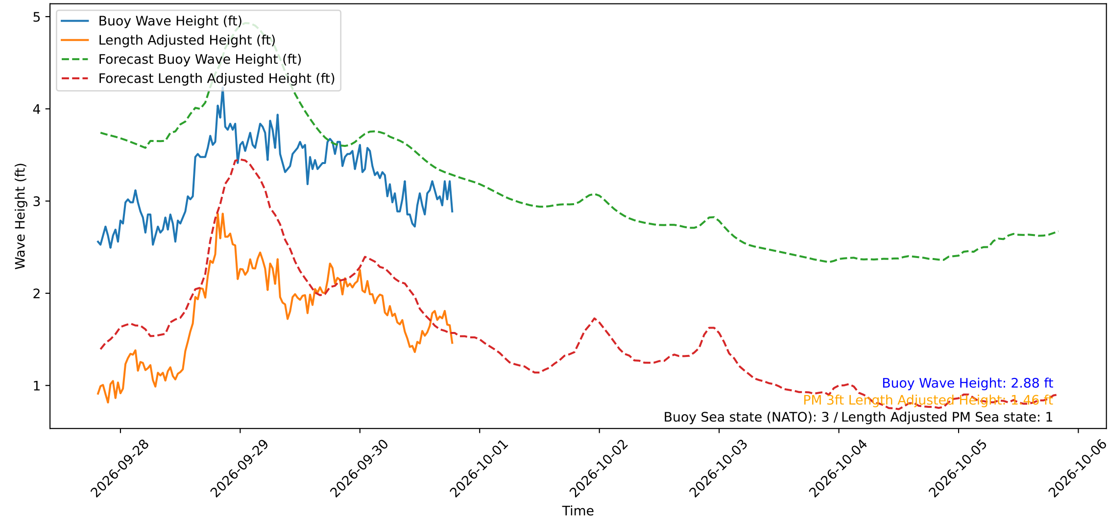
Wave Heights over Time for Oceanside Harbor at 2026-09-30 19:30:29
