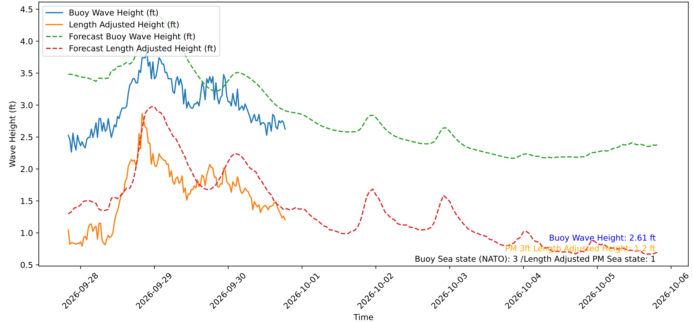
Wave Heights over Time for Red Beach at 2026-09-30 19:30:49
