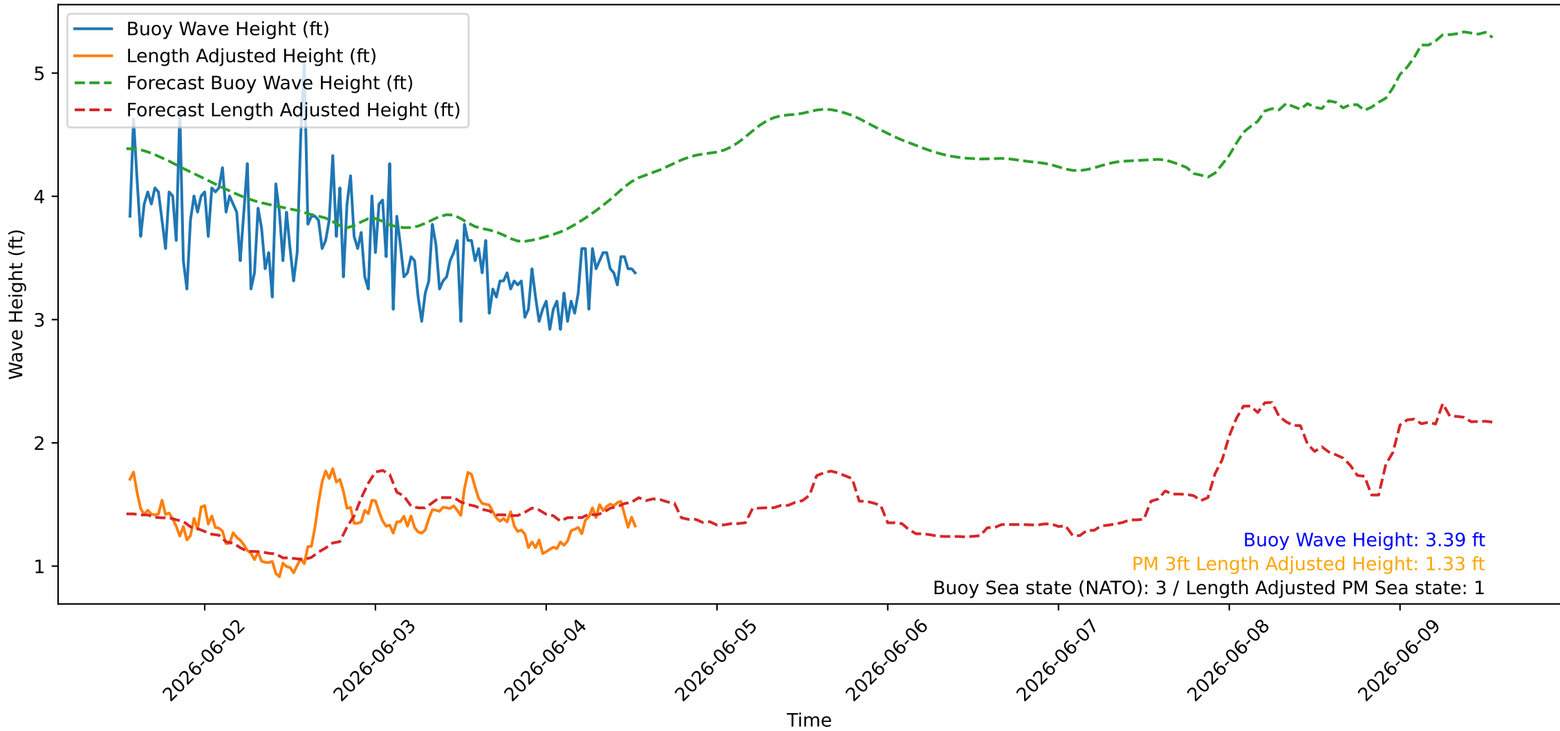
Wave Heights over Time for Oceanside Harbor at 2026-06-04 13:20:26
