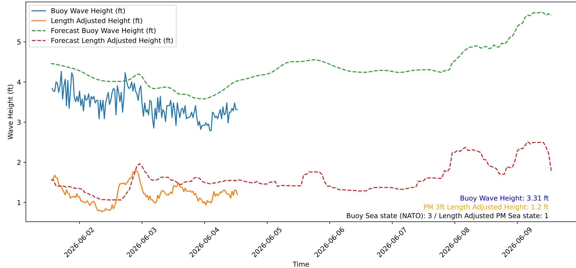
Wave Heights over Time for Green Beach at 2026-06-04 13:21:09
