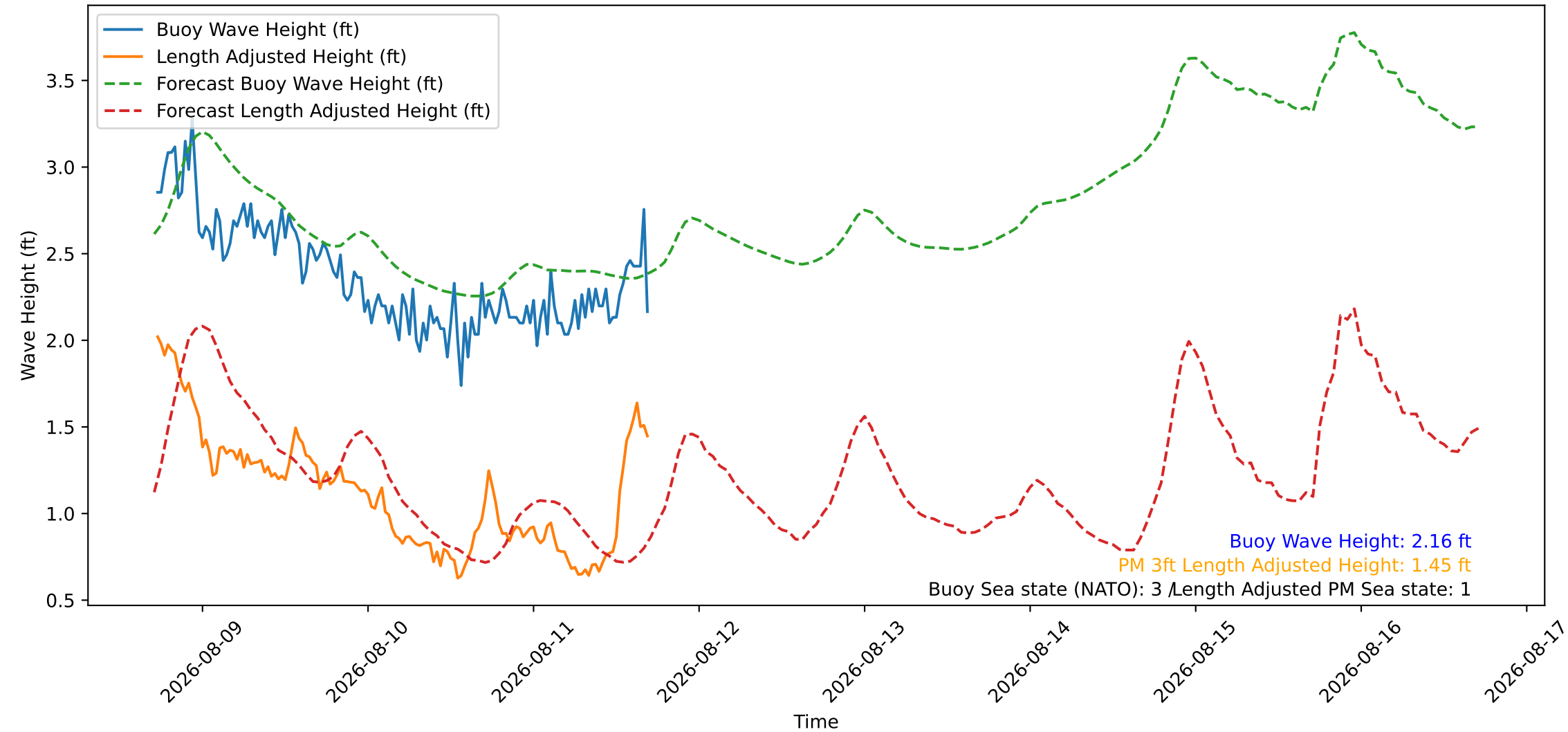
Wave Heights over Time for Red Beach at 2026-08-11 17:20:48
