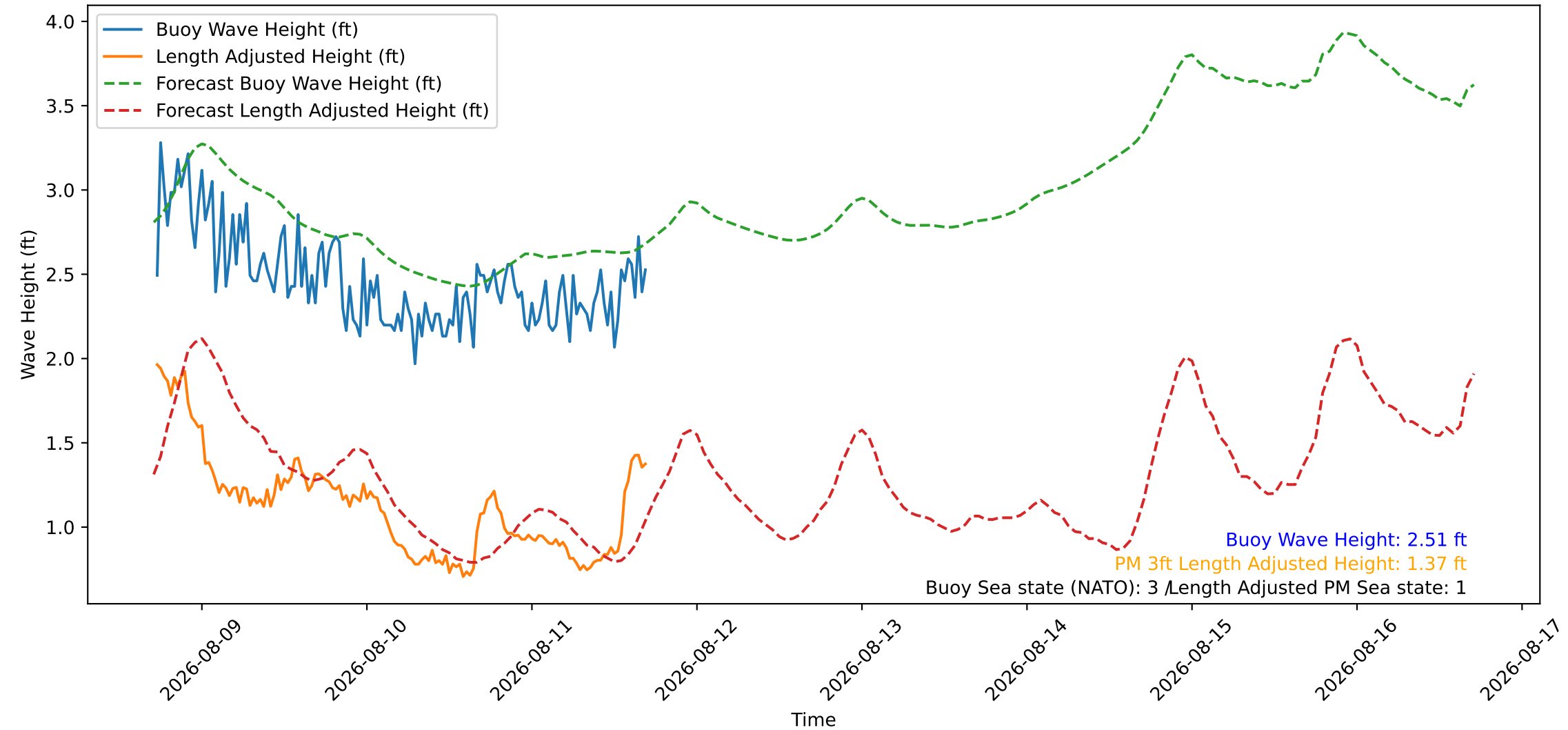
Wave Heights over Time for Oceanside Harbor at 2026-08-11 17:20:27
