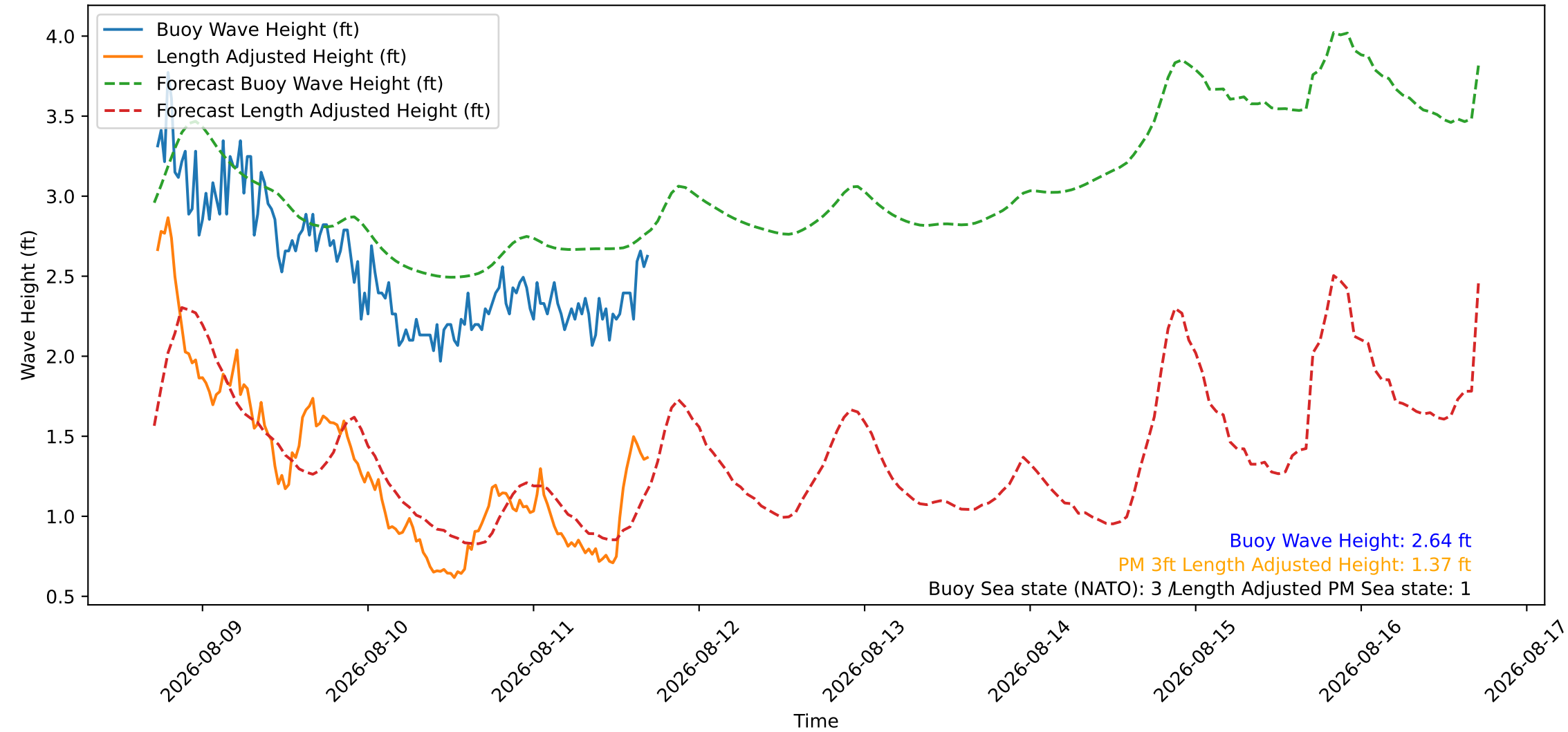
Wave Heights over Time for Green Beach at 2026-08-11 17:21:10
