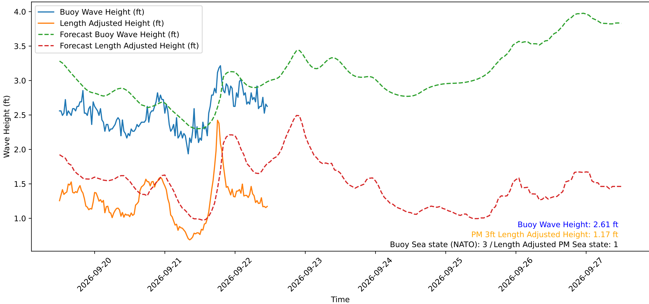
Wave Heights over Time for Green Beach at 2026-09-22 11:41:12
