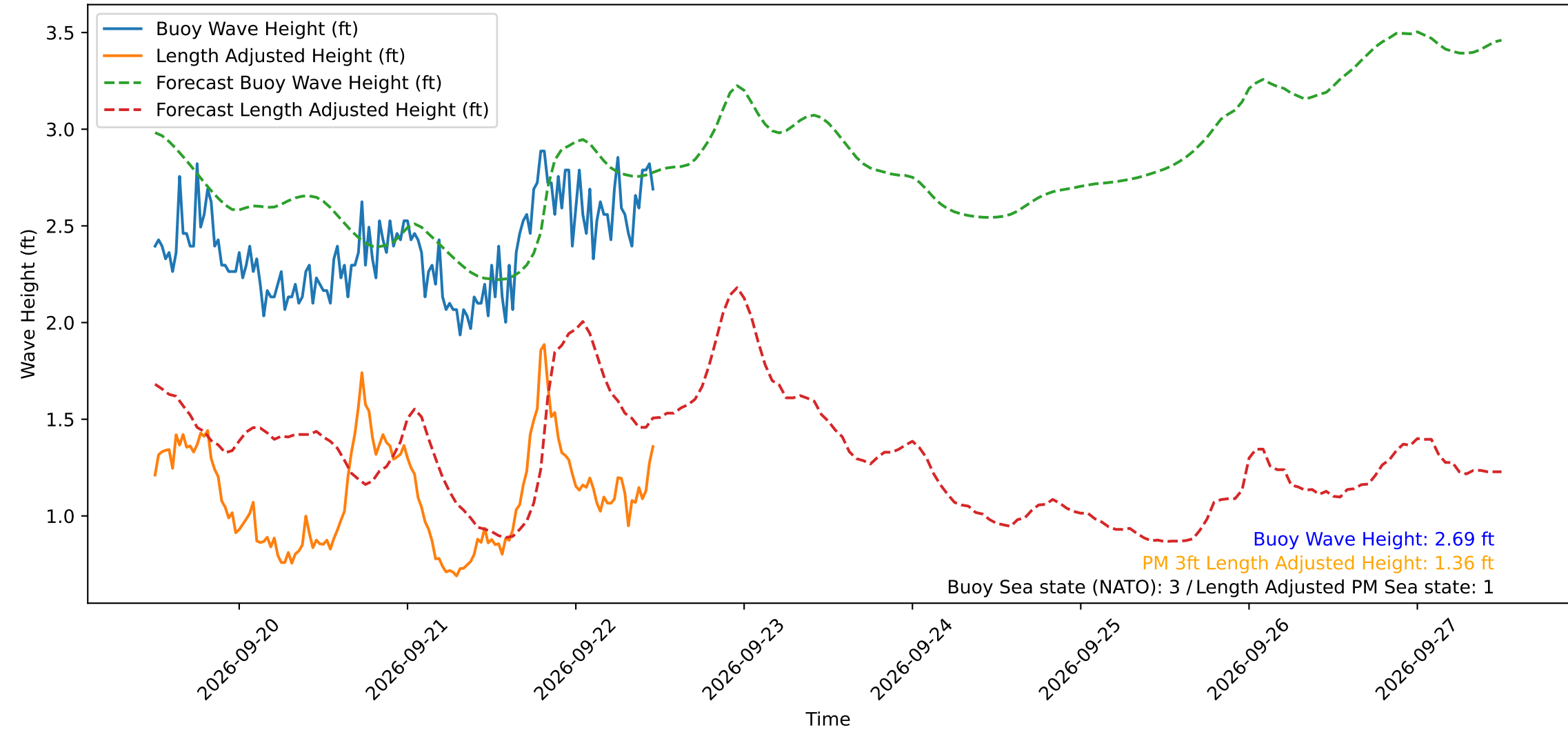
Wave Heights over Time for Red Beach at 2026-09-22 11:40:49
