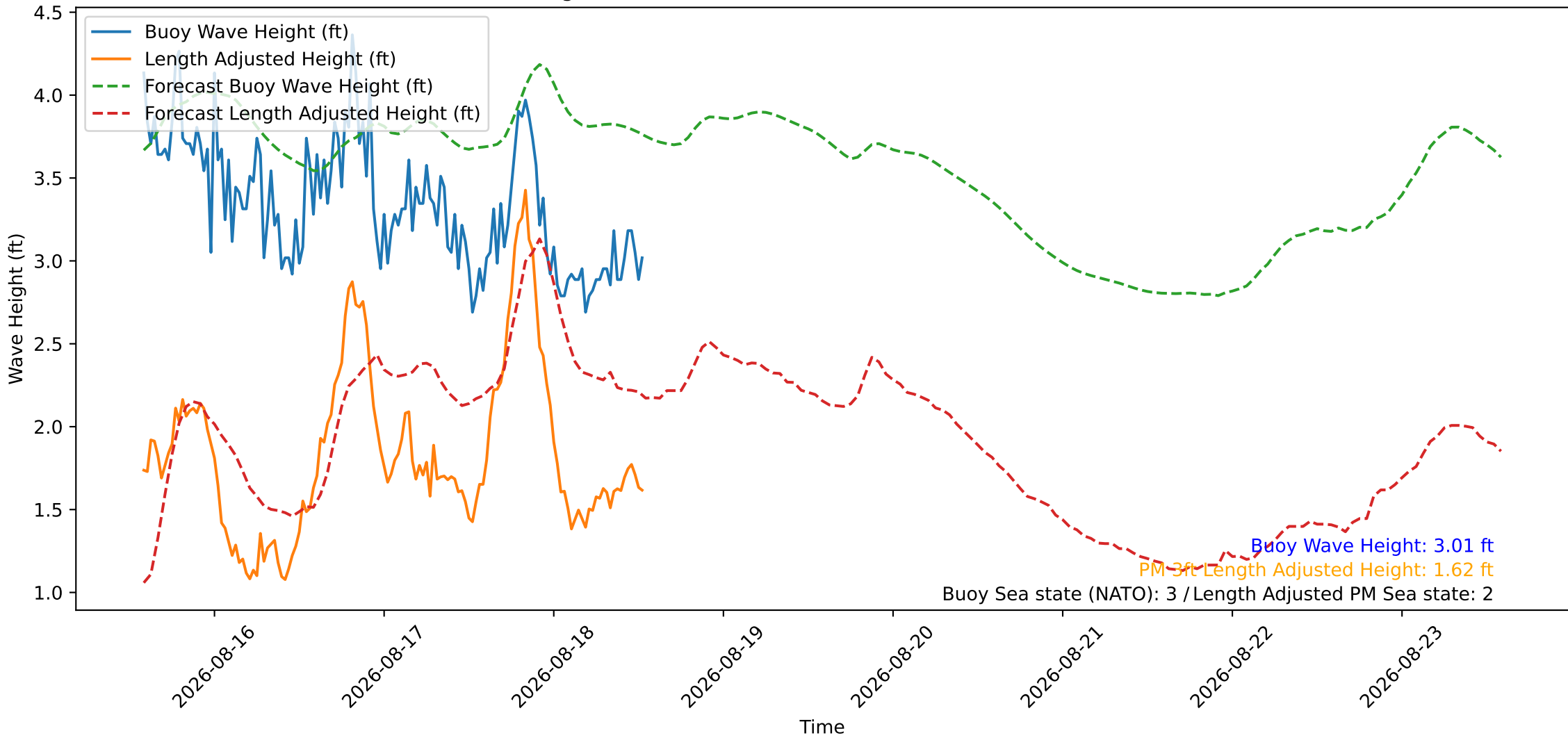
Wave Heights over Time for Green Beach at 2026-08-18 13:31:09
