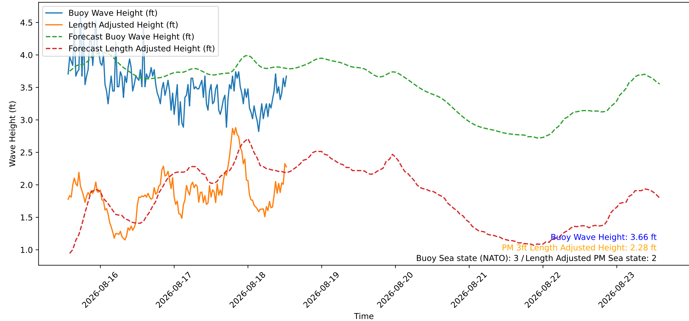
Wave Heights over Time for Oceanside Harbor at 2026-08-18 13:30:26
