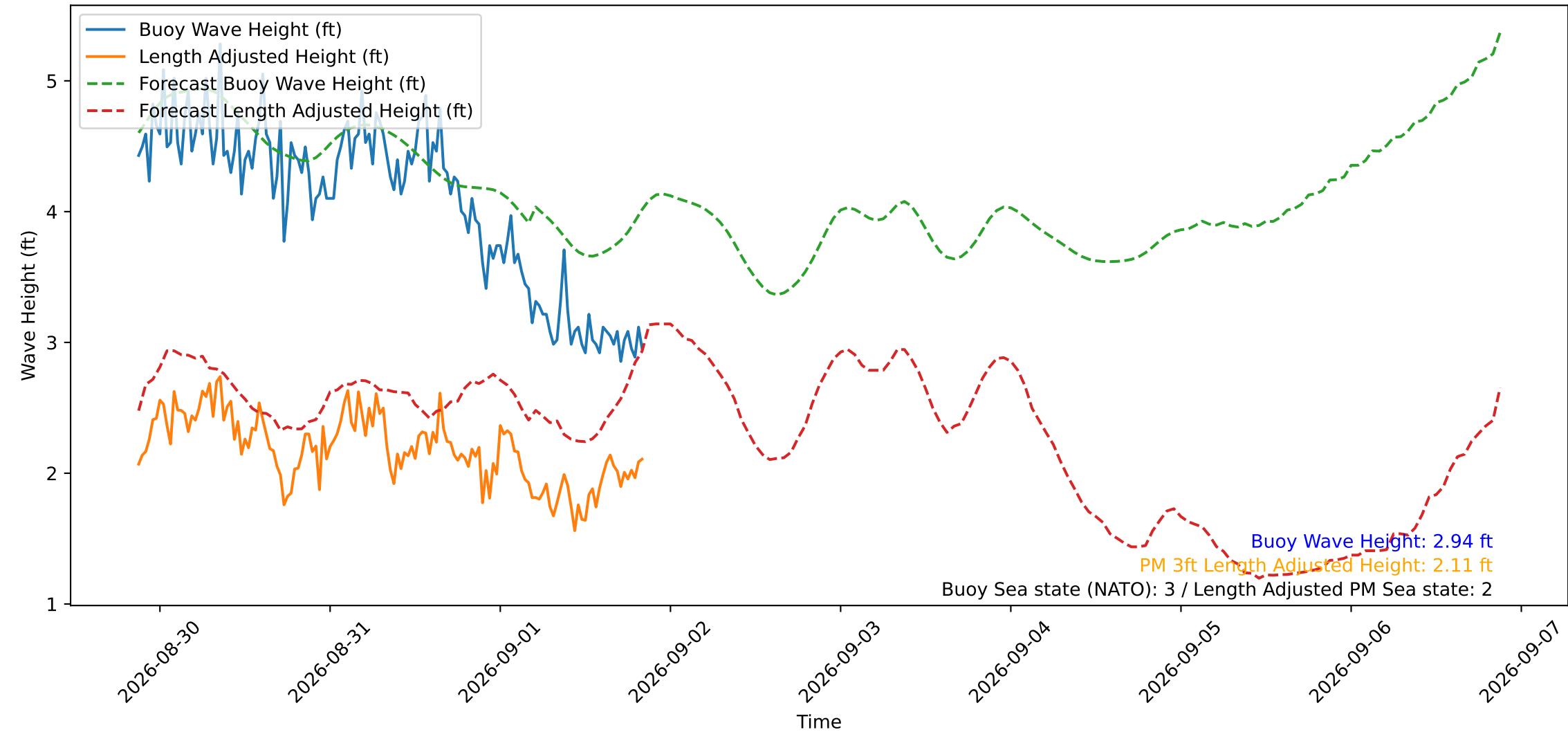
Wave Heights over Time for Oceanside Harbor at 2026-09-01 21:10:30
