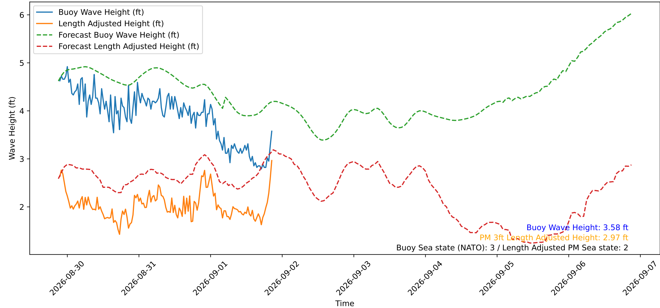
Wave Heights over Time for Green Beach at 2026-09-01 21:11:12
