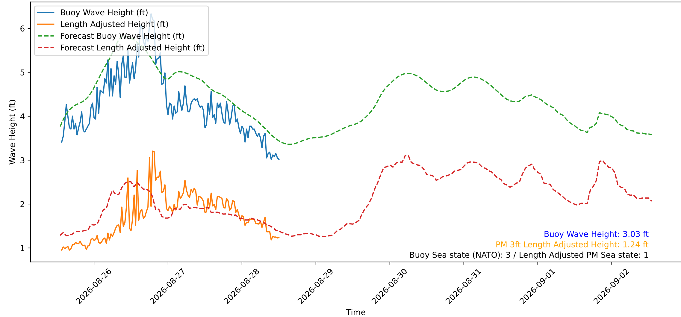
Wave Heights over Time for Green Beach at 2026-08-28 13:01:11
