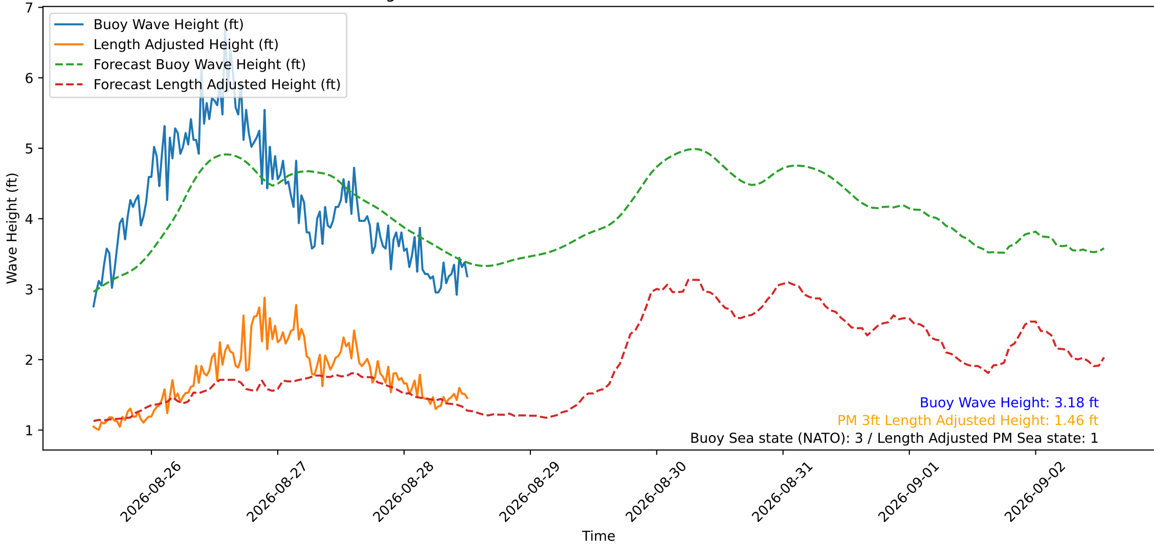
Wave Heights over Time for Oceanside Harbor at 2026-08-28 13:00:30
