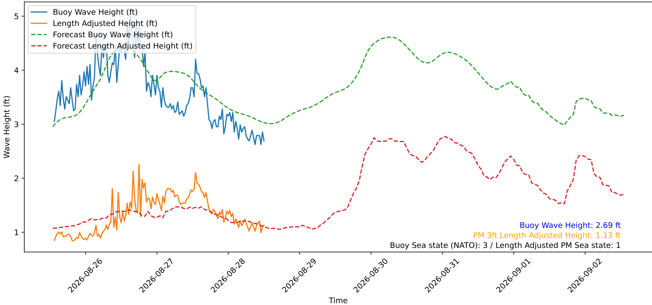
Wave Heights over Time for Red Beach at 2026-08-28 13:00:49
