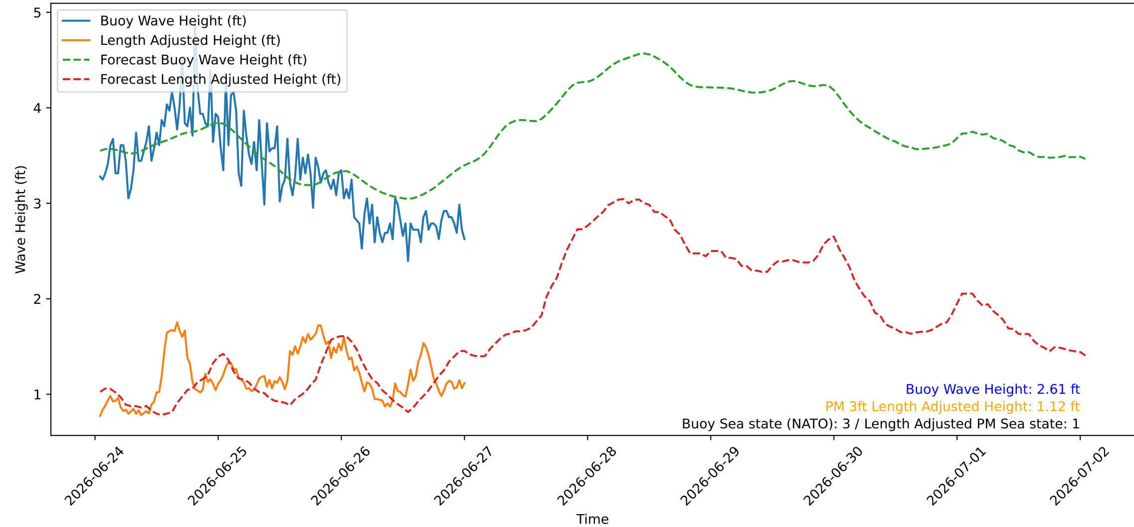
Wave Heights over Time for Oceanside Harbor at 2026-06-27 00:50:26
