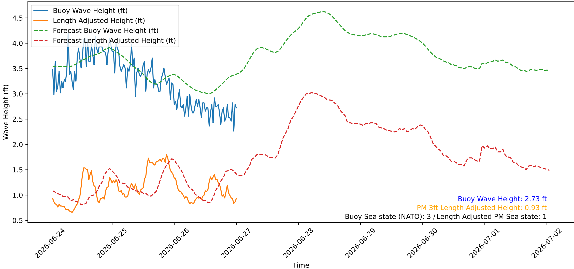
Wave Heights over Time for Green Beach at 2026-06-27 00:51:09
