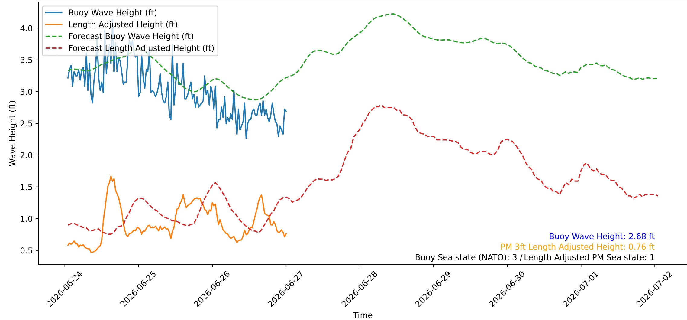
Wave Heights over Time for Red Beach at 2026-06-27 00:50:47
