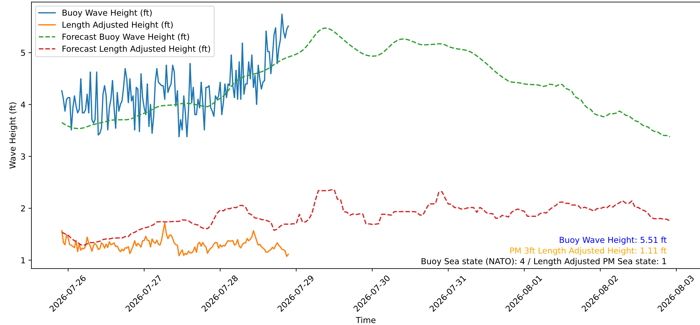
Wave Heights over Time for Green Beach at 2026-07-28 22:11:08
