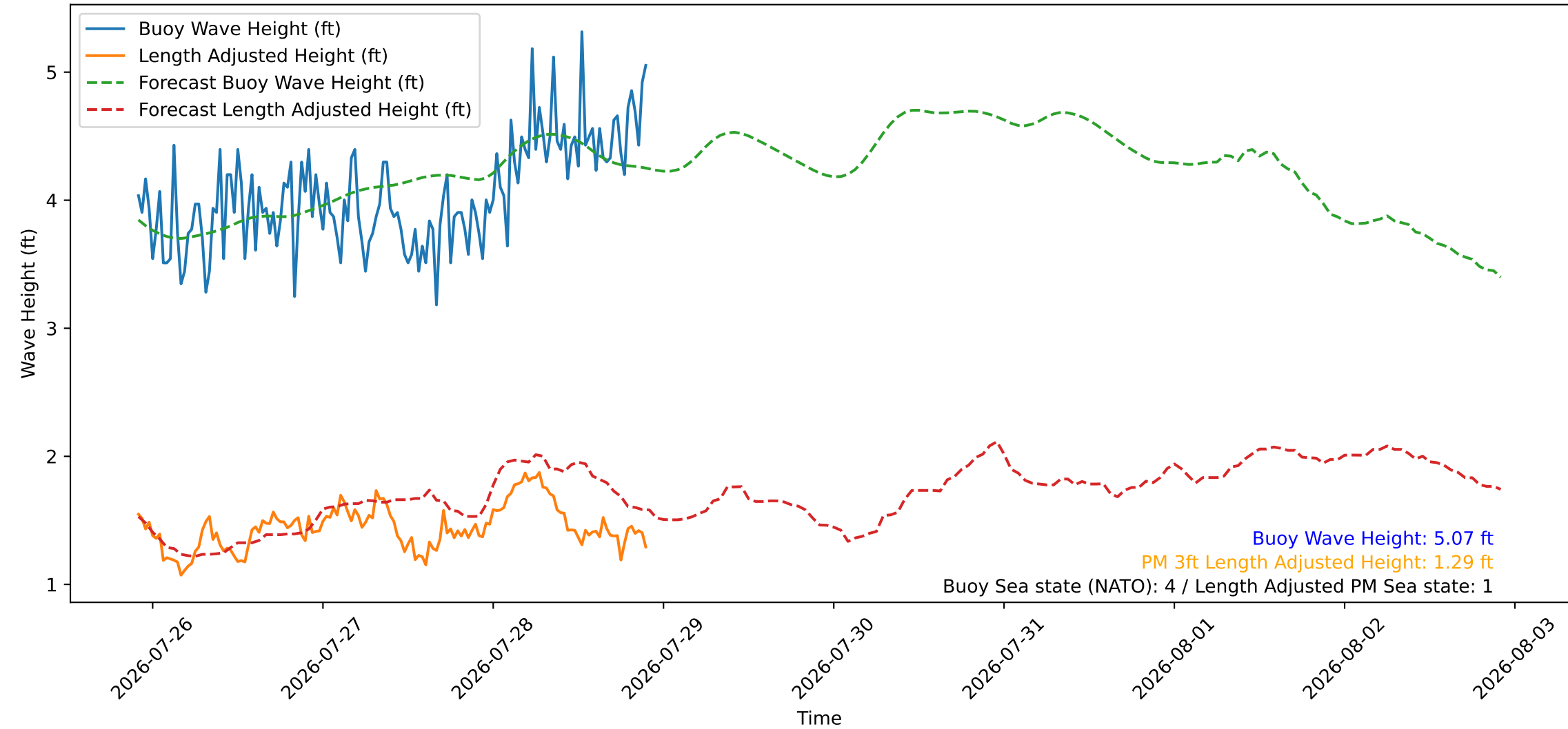
Wave Heights over Time for Oceanside Harbor at 2026-07-28 22:10:26
