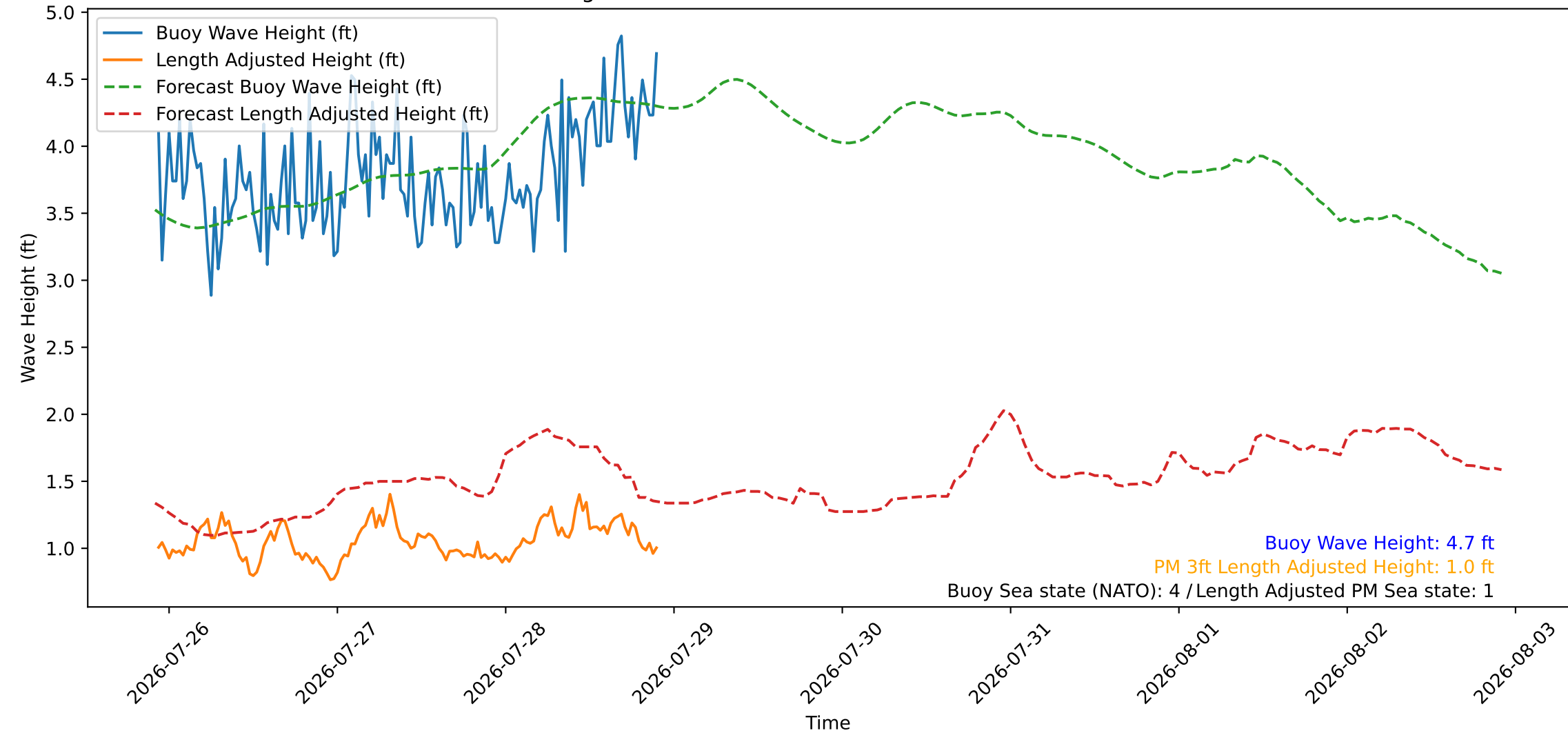
Wave Heights over Time for Red Beach at 2026-07-28 22:10:46
