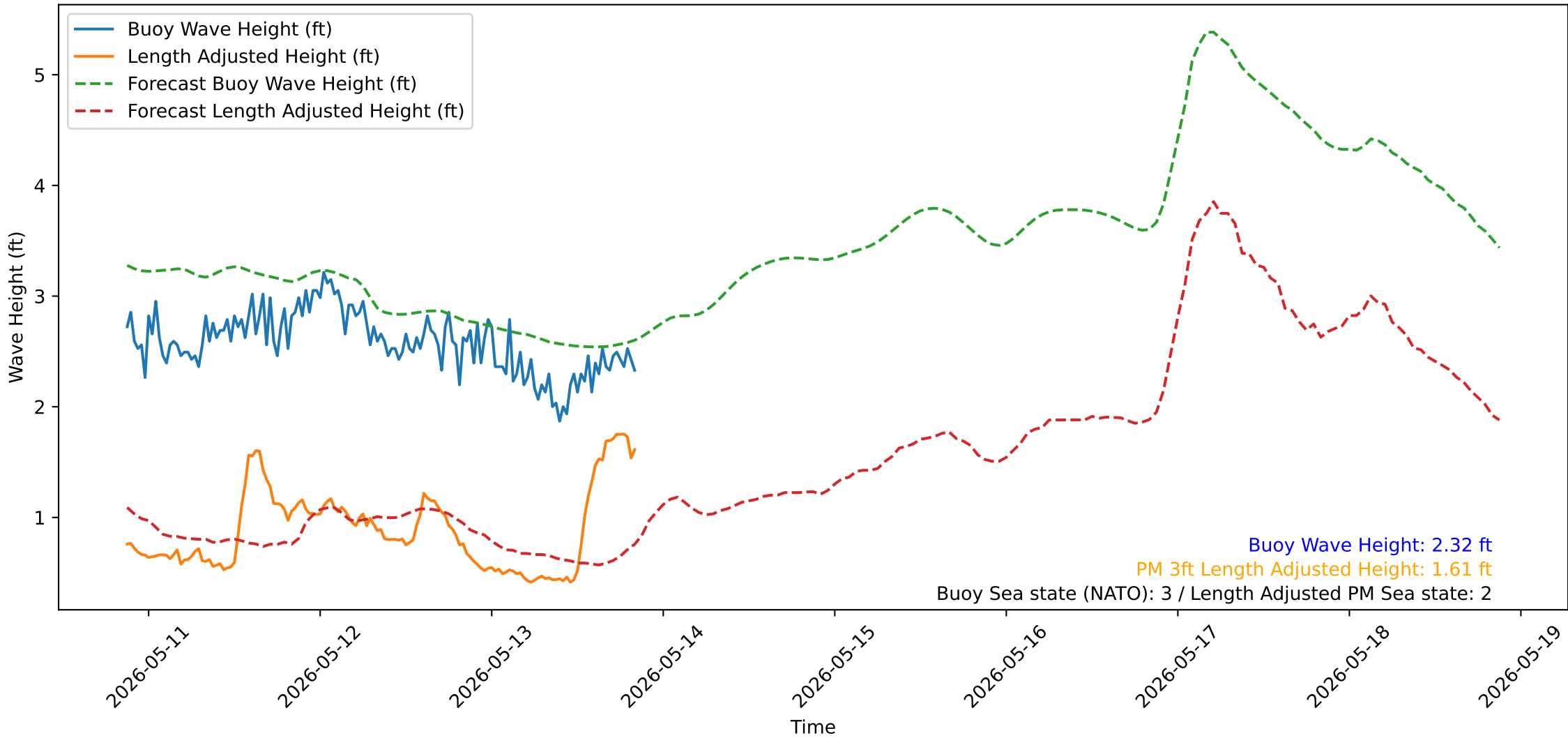
Wave Heights over Time for Red Beach at 2026-05-13 20:50:51
