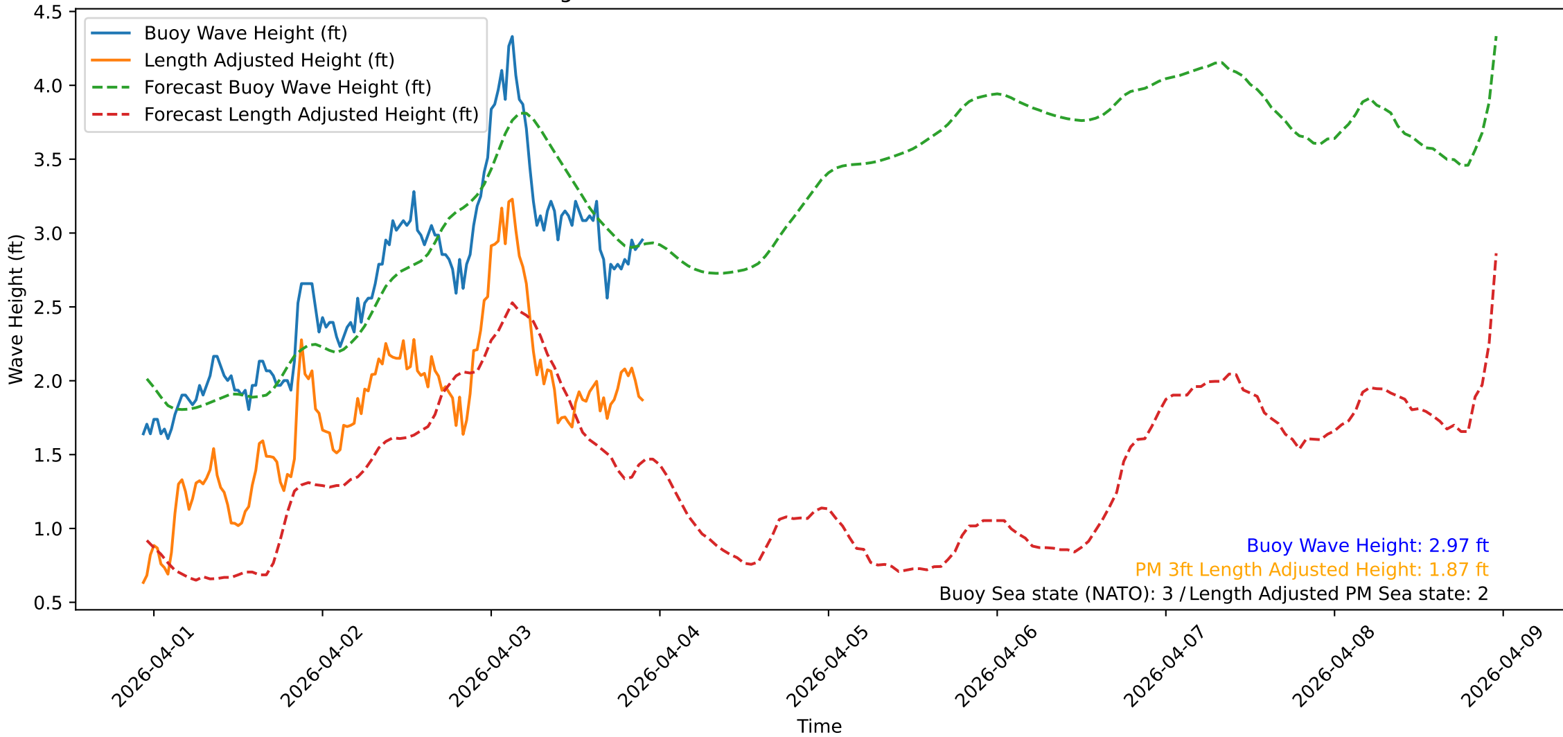
Wave Heights over Time for Green Beach at 2026-04-03 22:31:29
