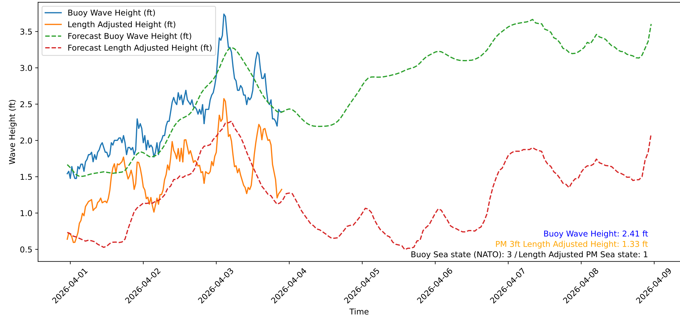
Wave Heights over Time for Red Beach at 2026-04-03 22:31:00
