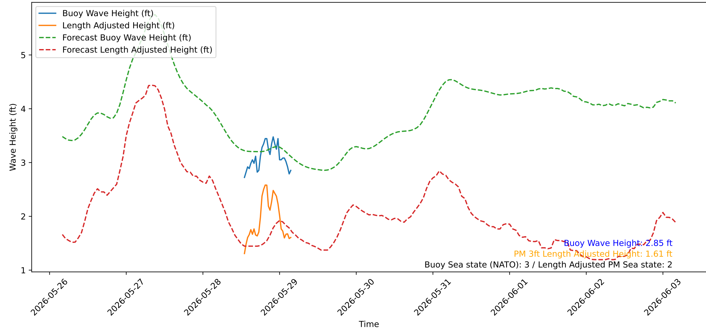
Wave Heights over Time for Oceanside Harbor at 2026-05-29 04:20:21
