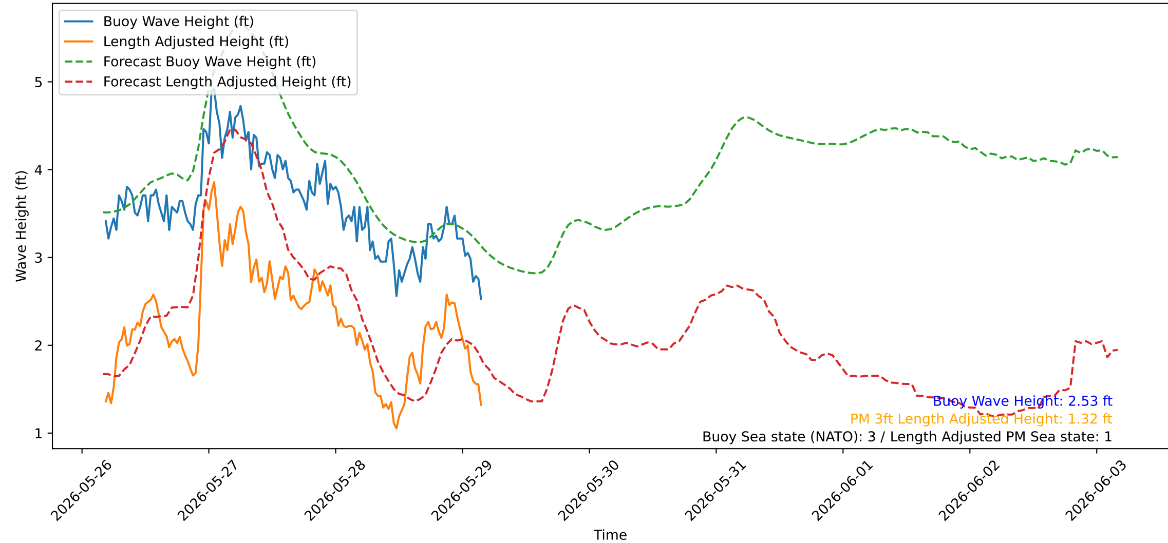
Wave Heights over Time for Green Beach at 2026-05-29 04:21:03
