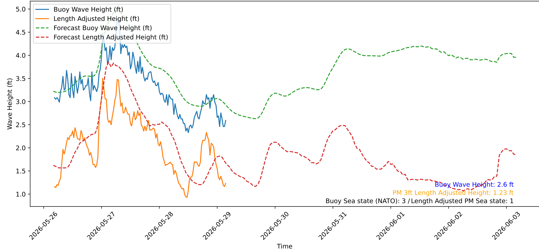
Wave Heights over Time for Red Beach at 2026-05-29 04:20:41
