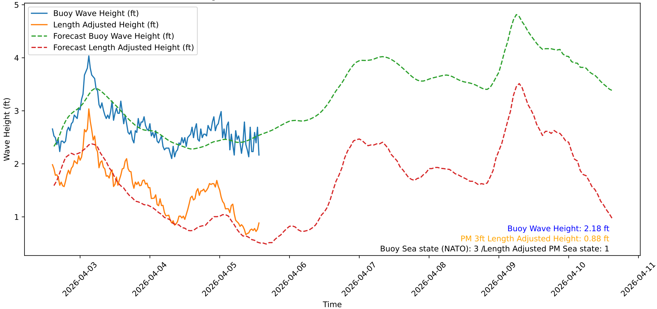
Wave Heights over Time for Oceanside Harbor at 2026-04-05 14:30:31
