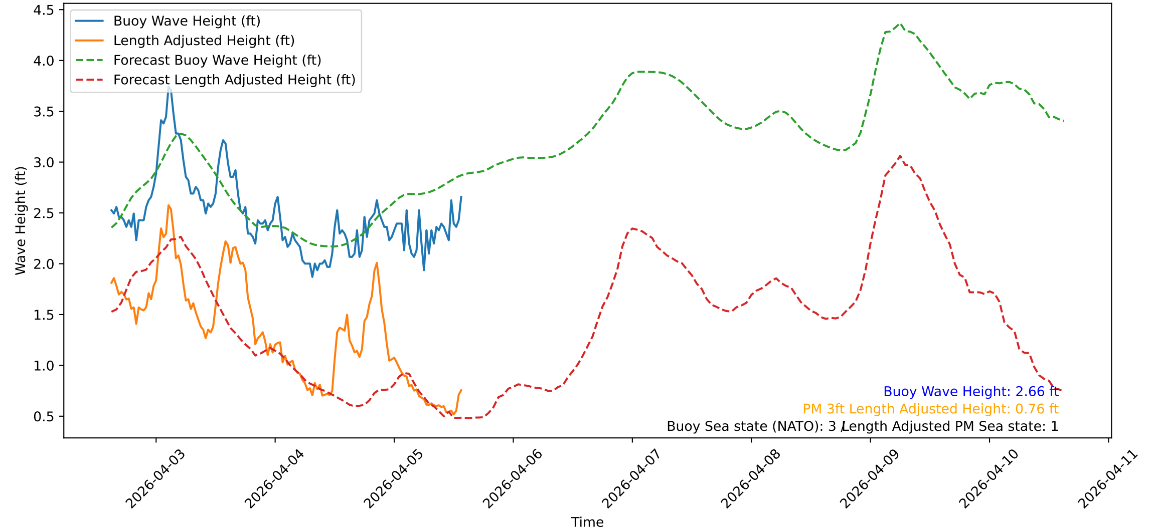
Wave Heights over Time for Red Beach at 2026-04-05 14:30:47
