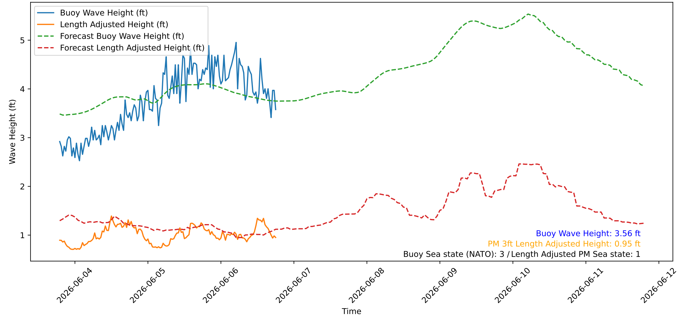
Wave Heights over Time for Red Beach at 2026-06-06 18:50:46
