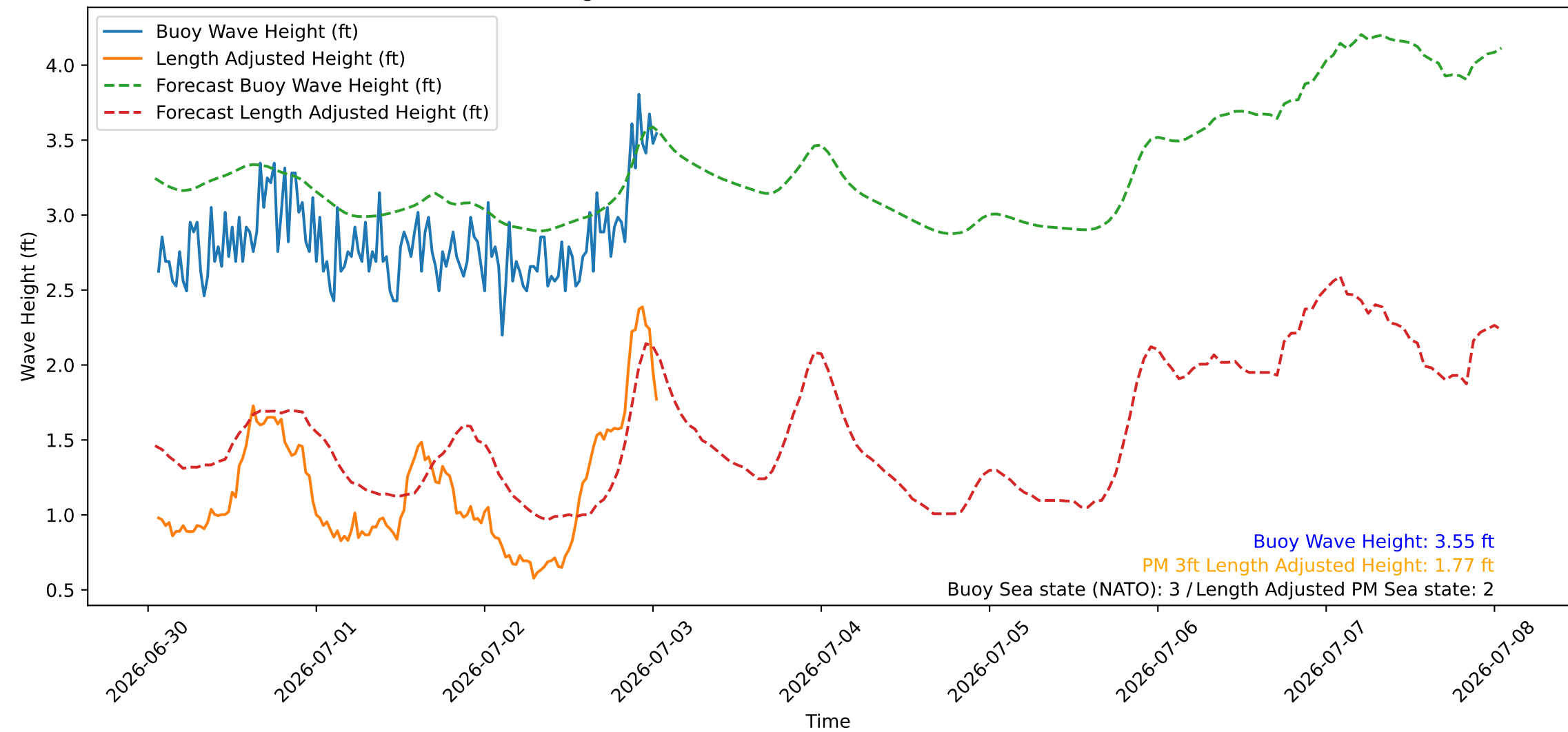
Wave Heights over Time for Red Beach at 2026-07-03 01:10:45
