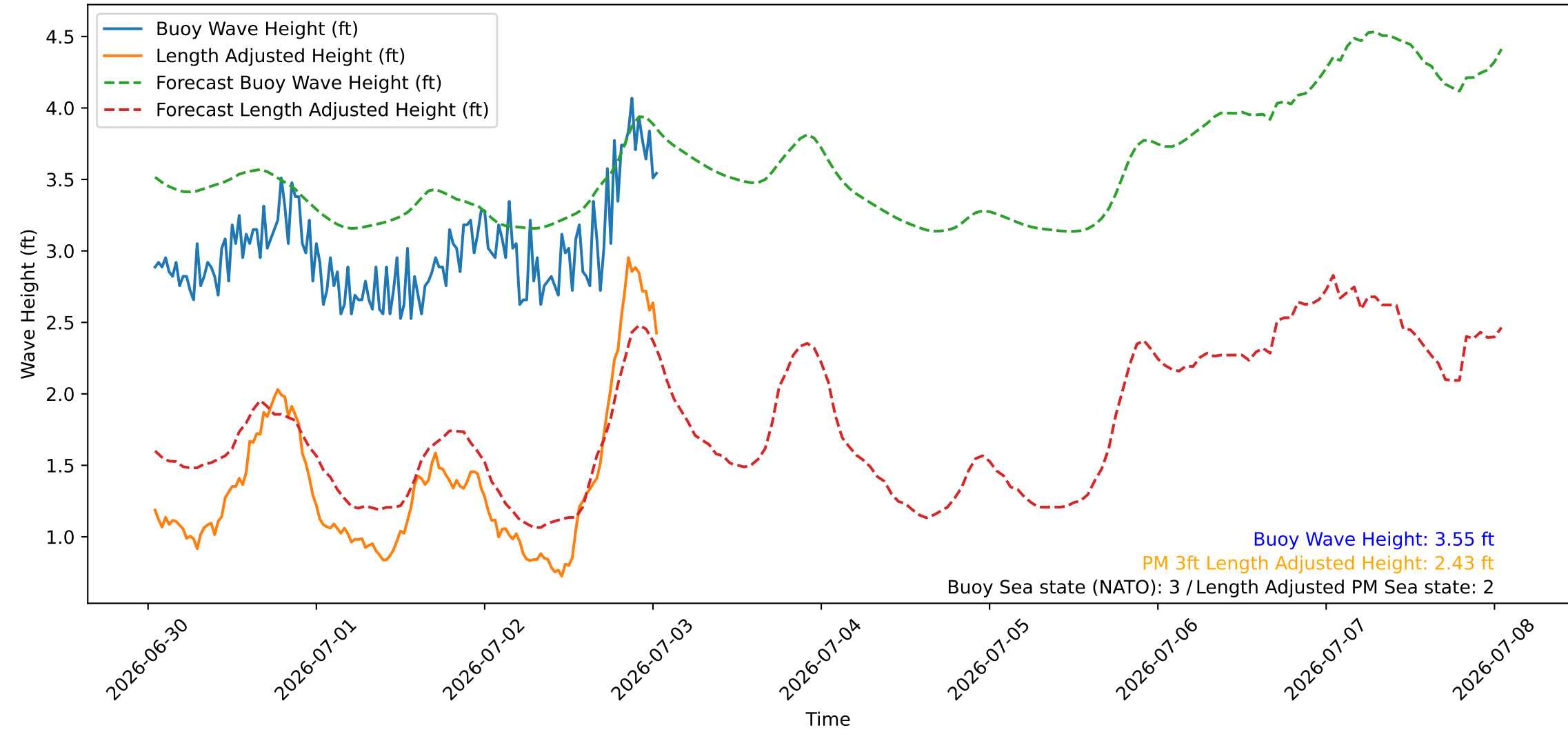
Wave Heights over Time for Green Beach at 2026-07-03 01:11:07
