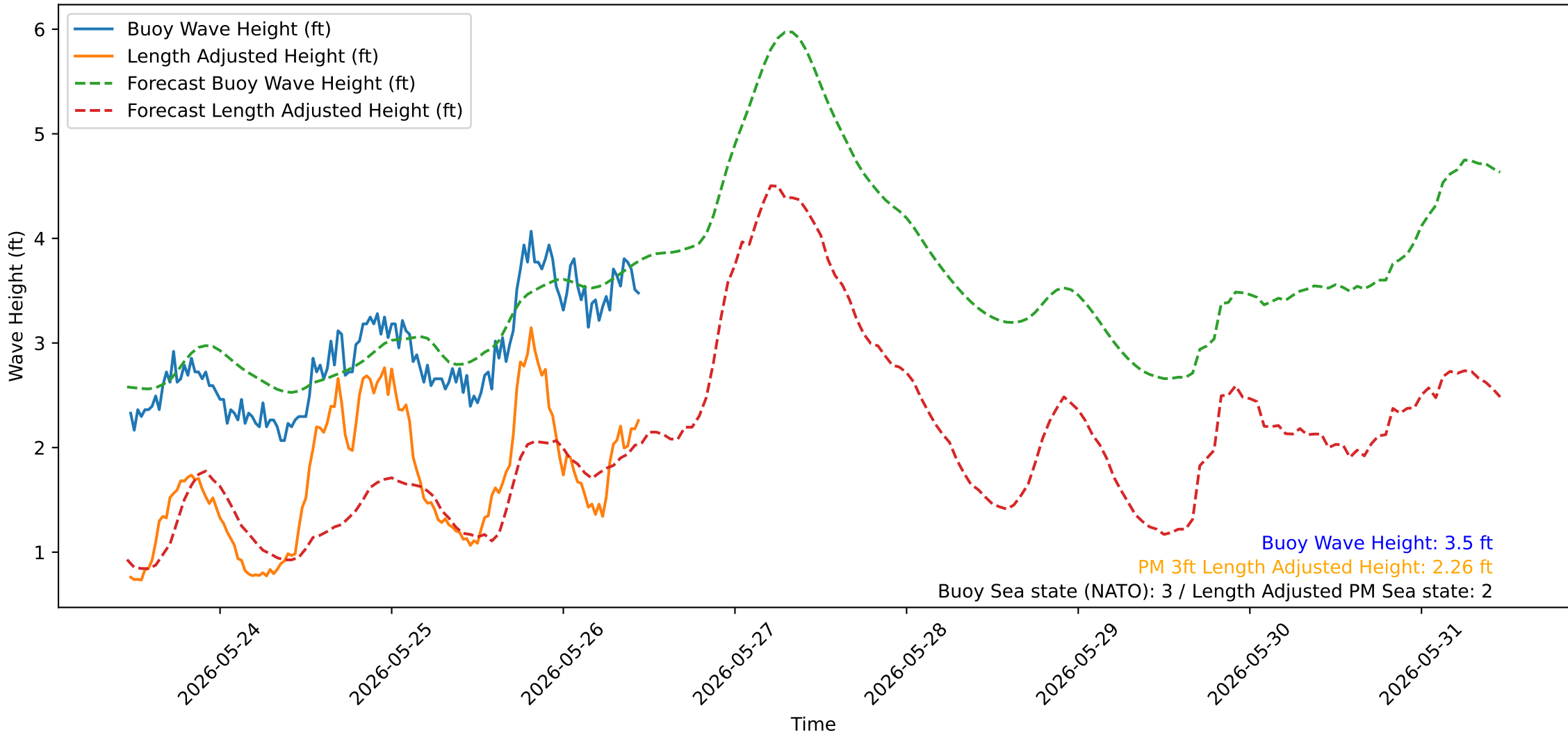
Wave Heights over Time for Green Beach at 2026-05-26 11:21:10
