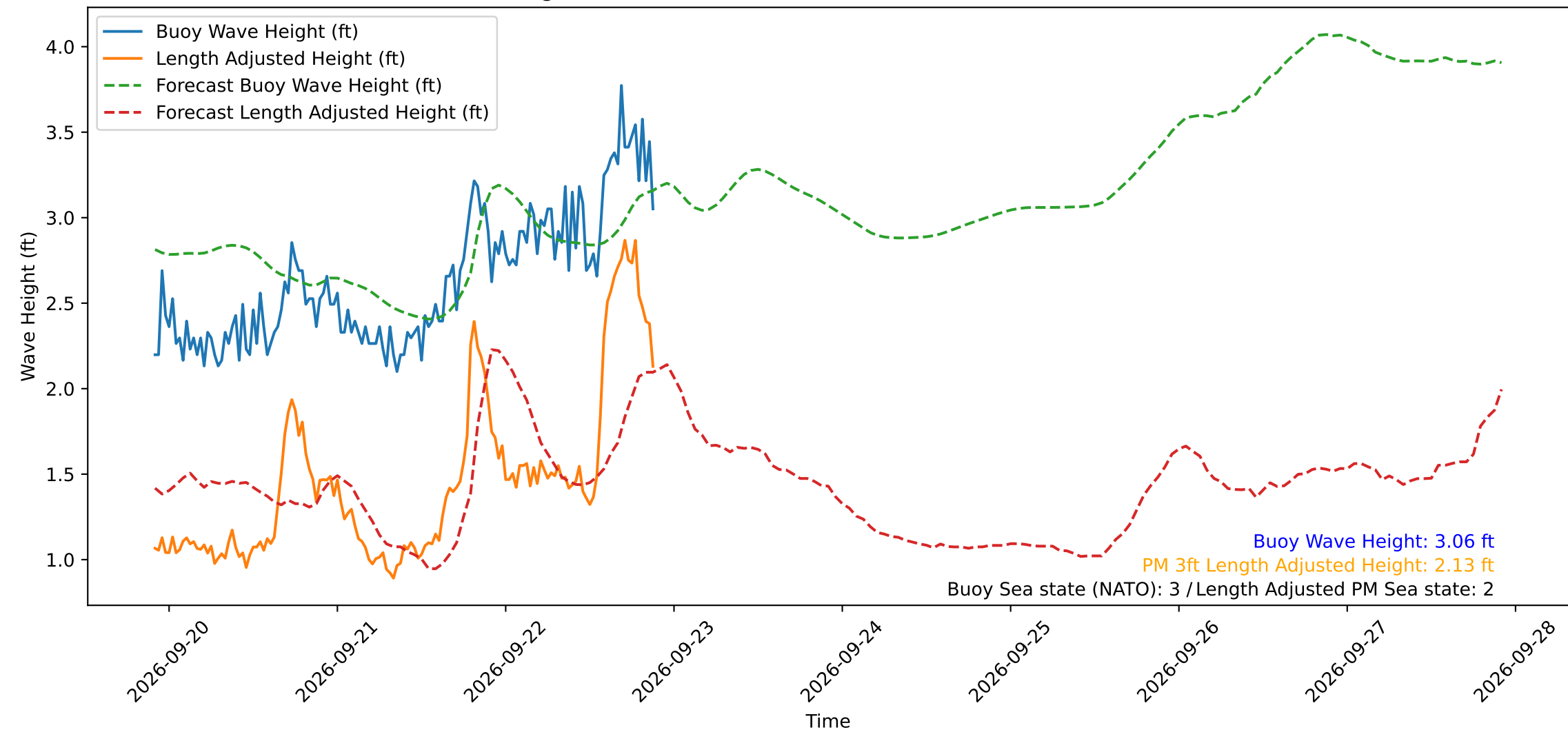
Wave Heights over Time for Oceanside Harbor at 2026-09-22 21:50:29
